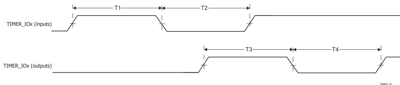
Figure 6-117. Timer Timing
