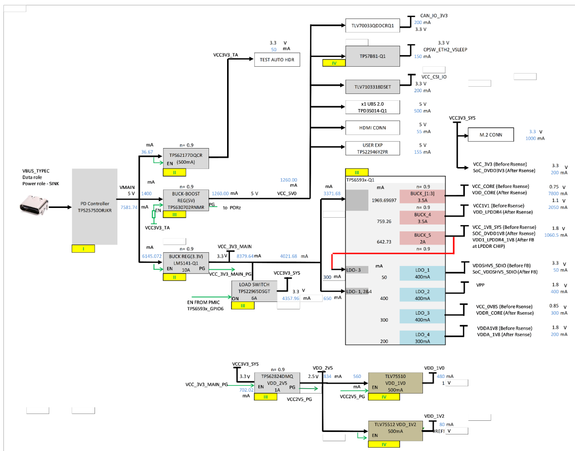
Figure 2-31. Power Architecture
