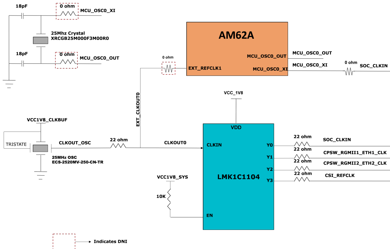
Figure 2-11. Clock Architecture
