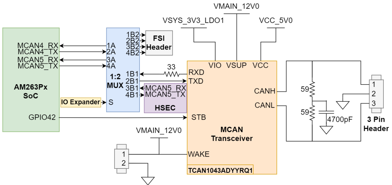
Figure 2-28. MCAN Transceiver
