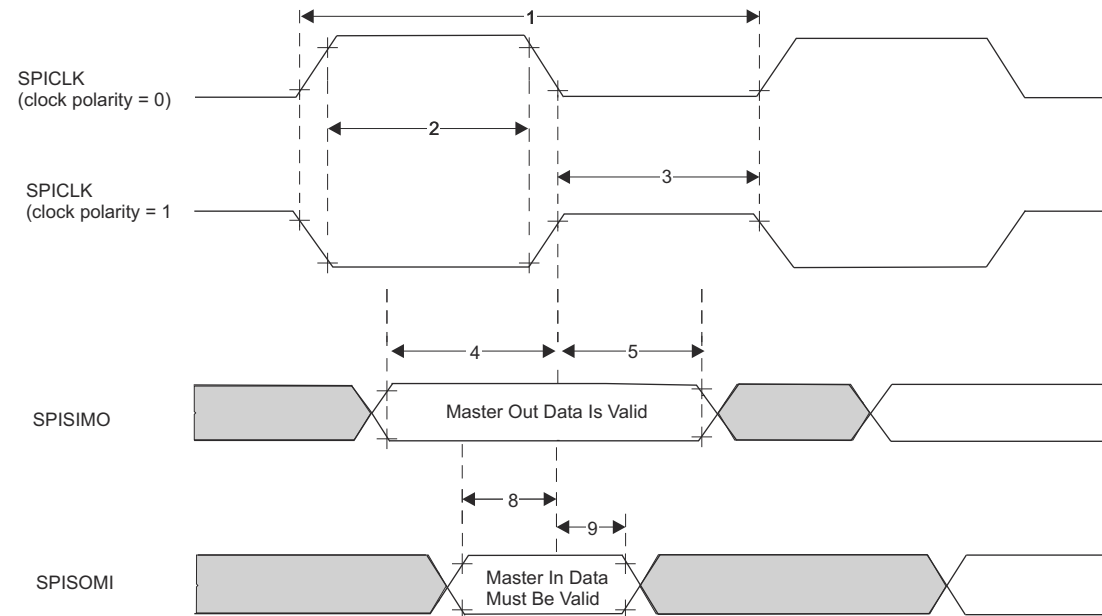
Figure 6-8. SPI Controller Mode External Timing (CLOCK PHASE = 0)
