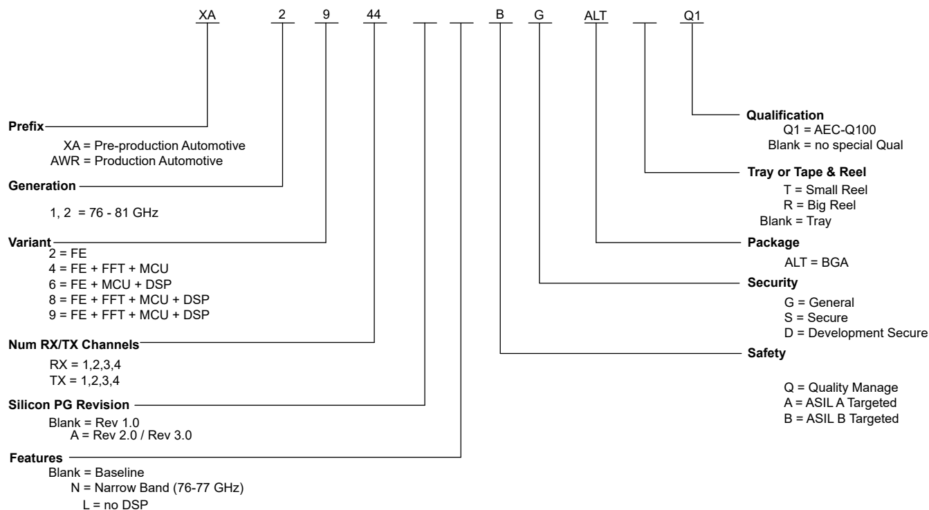
Figure 10-1. Device Nomenclature
