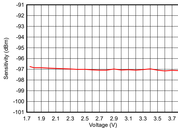
Figure 7-18. Sensitivity vs Supply Voltage (VDD) (BLE 1Mbps, 2.44GHz)
