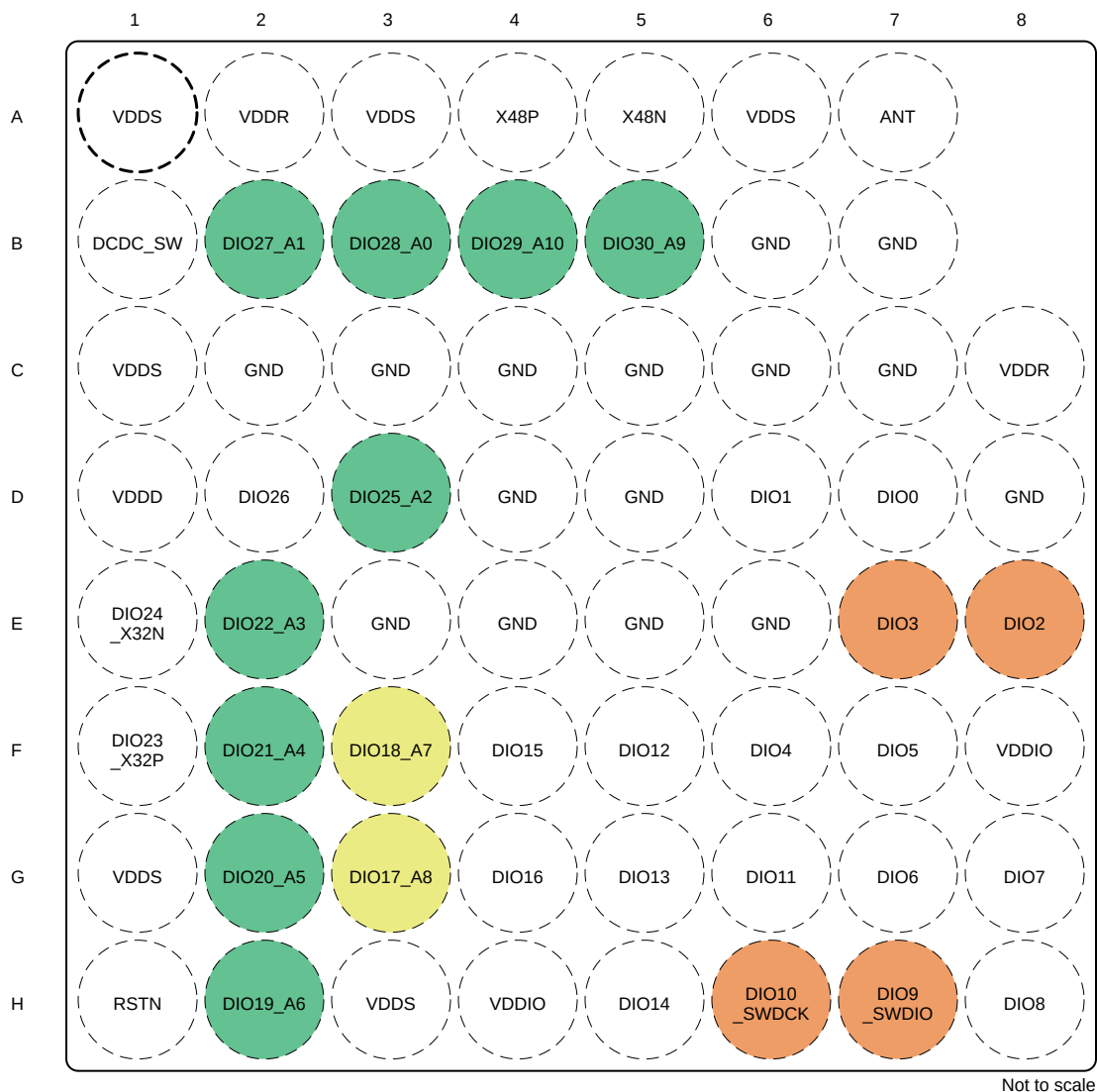
Figure 6-2. YCJ WCSP Pinout (Top View)
