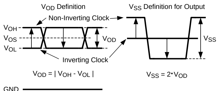
Figure 8. Two Different Definitions for Differential Output Signals
