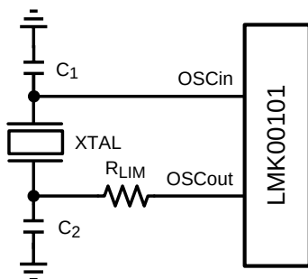
Figure 12. Crystal Interface
