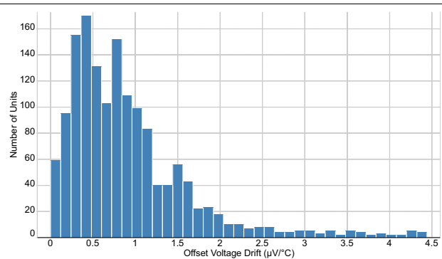
Figure 8-26. OA Offset Voltage Drift Sample Production Distribution
