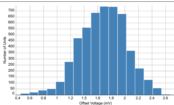
Figure 8-25. OA Offset Voltage Sample Production Distribution
