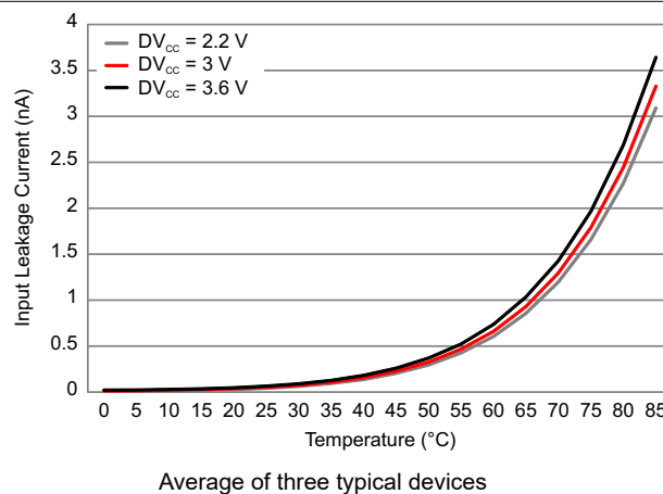
Figure 8-27. Ground Switch Input Leakage Current vs Temperature
