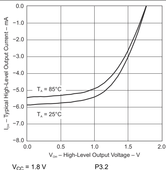
Figure 8-6. Typical High-Level Output Current Vs High-Level Output Voltage
