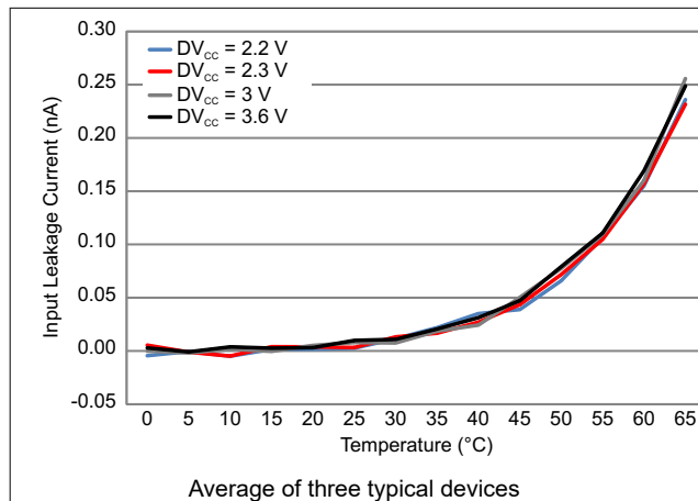
Figure 8-28. OA Switch Input Leakage Current vs Temperature
