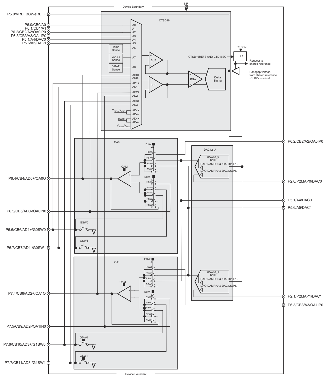
Figure 9-2. Signal Chain
