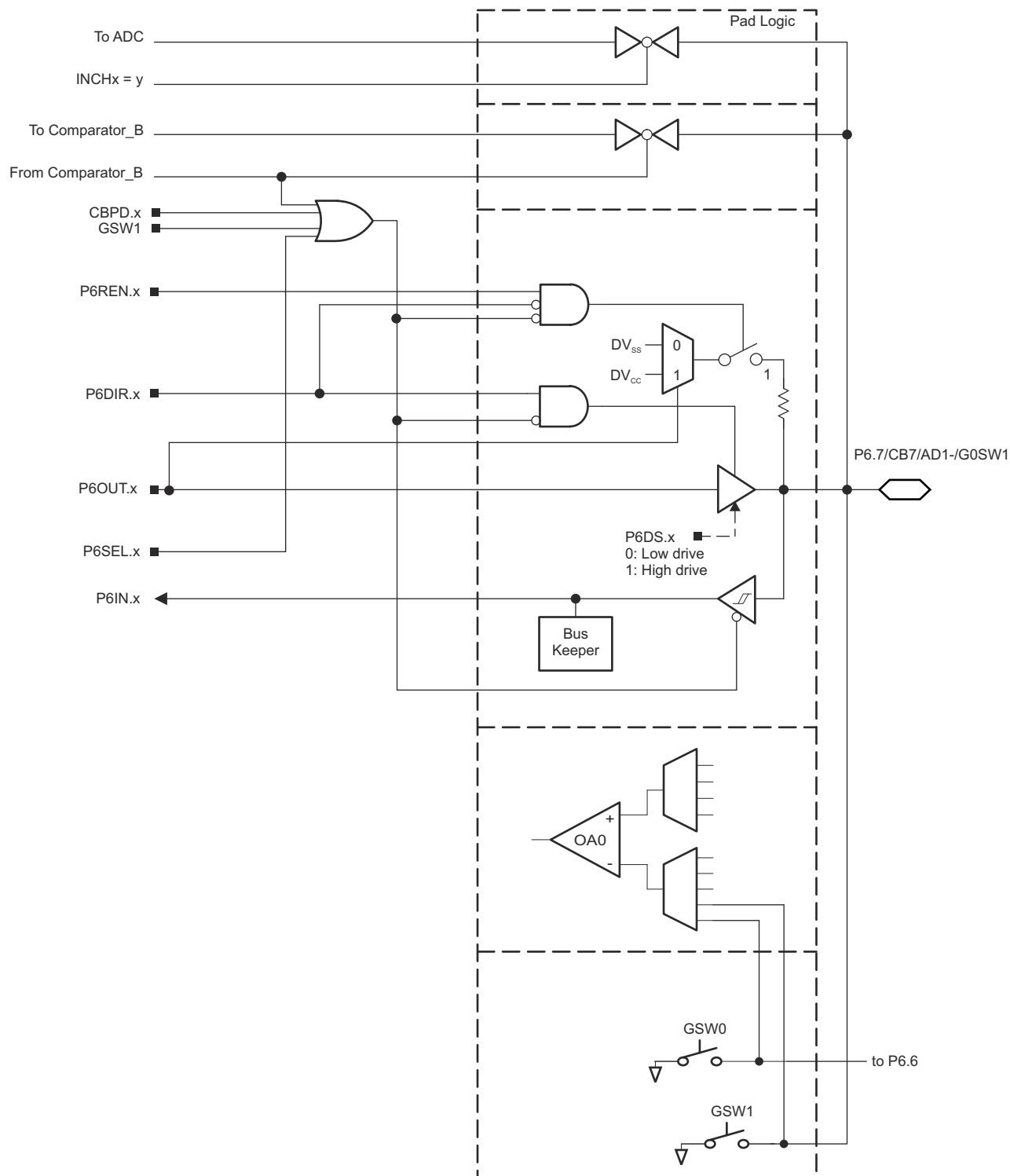
Figure 9-15. Port P6 (P6.7) Diagram
