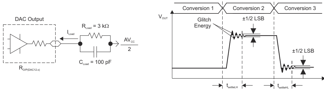
Figure 8-21. Settling Time and Glitch Energy Testing
