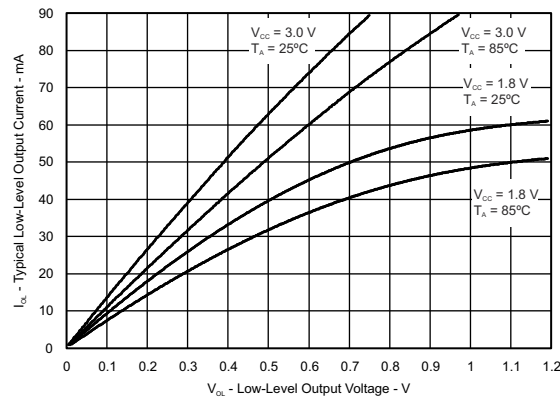
Figure 8-30. Ports PU.0, PU.1 Typical Low-Level Output Characteristics
