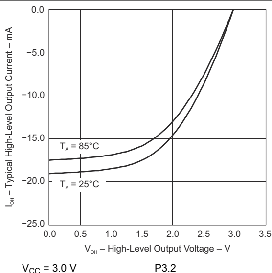
Figure 8-5. Typical High-Level Output Current Vs High-Level Output Voltage
