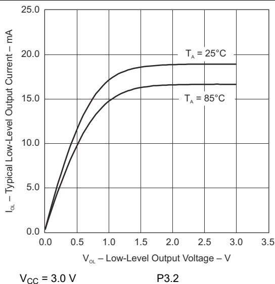
Figure 8-3. Typical Low-Level Output Current vs Low-Level Output Voltage
