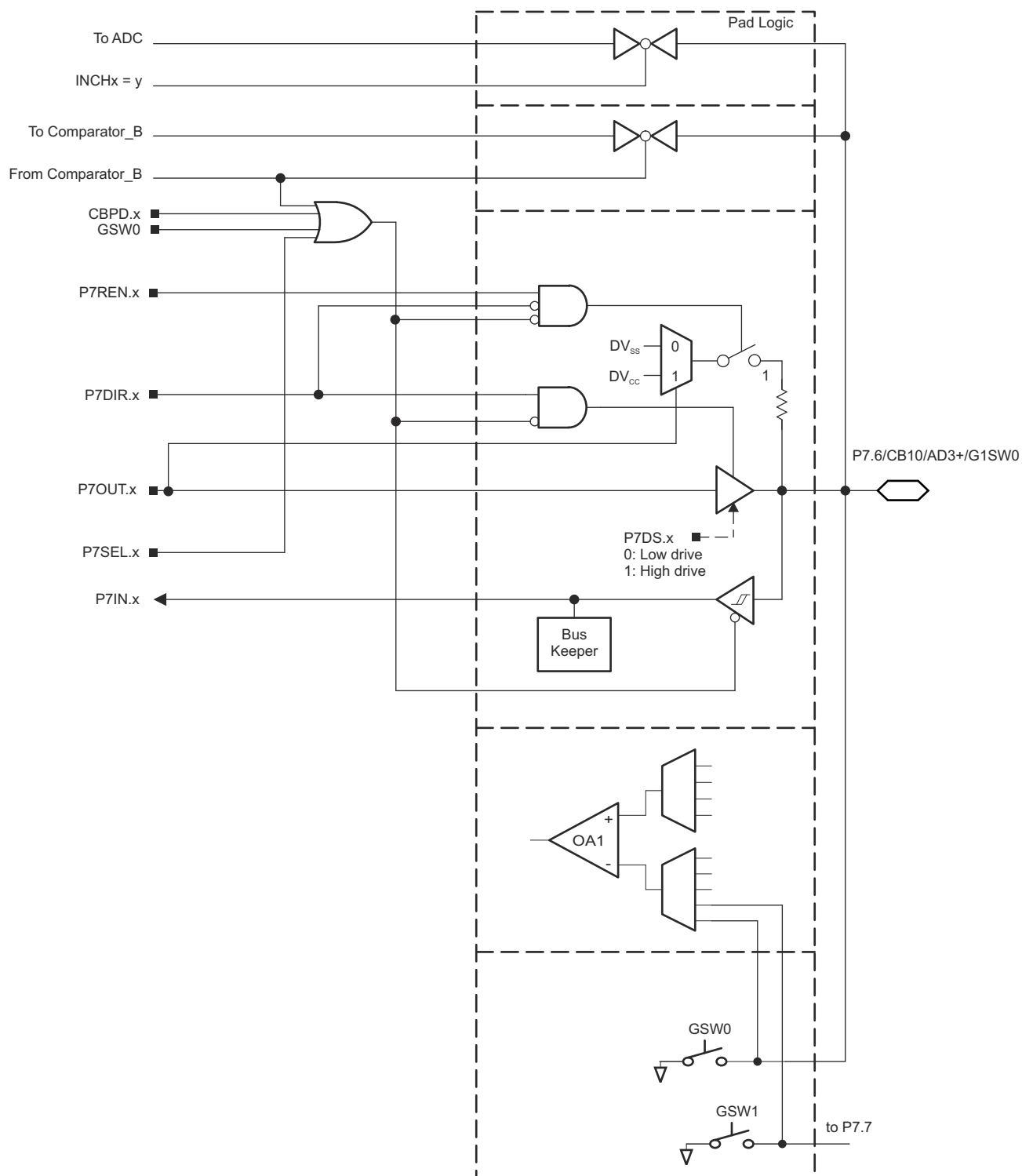
Figure 9-20. Port P7 (P7.6) Diagram
