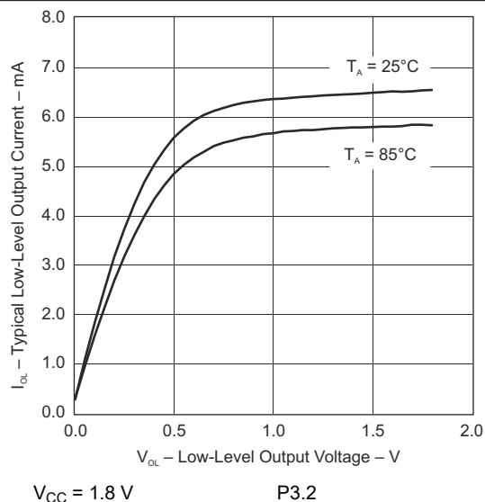
Figure 8-4. Typical Low-Level Output Current vs Low-Level Output Voltage
