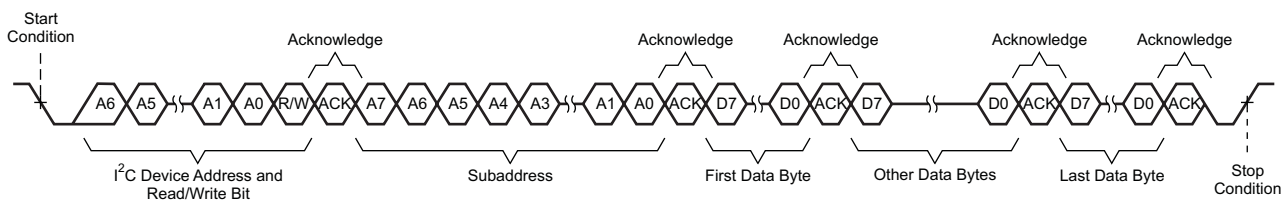
Figure 14. Sequential Write Transfer
