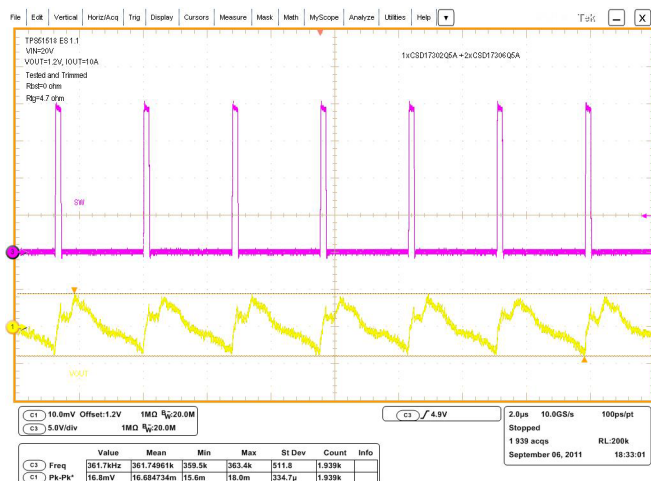
Figure 17. Steady-State Ripple, I_{LOAD} = 10\text{ A}
