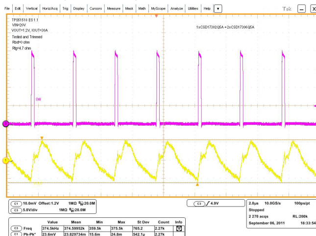
Figure 18. Steady-State Ripple, I_{LOAD} = 30\text{ A}
