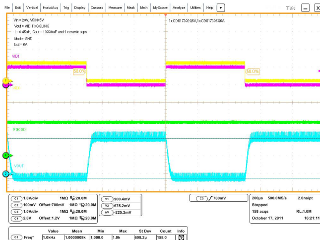
Figure 20. VID transition, I_{LOAD} = 6\text{ A}
