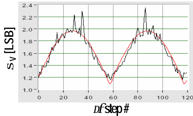
Fig. 9. Final jitter test run on the optimized clock decoupling ADS5420 version, with external filtered clock. The measured value for the jitter is 250fs RMS. This dramatically reduced jitter value exposes statistical effects of many noise sources which were hidden in Fig. 3, but are effectively averaged out by the coherent sampling algorithm proposed.
