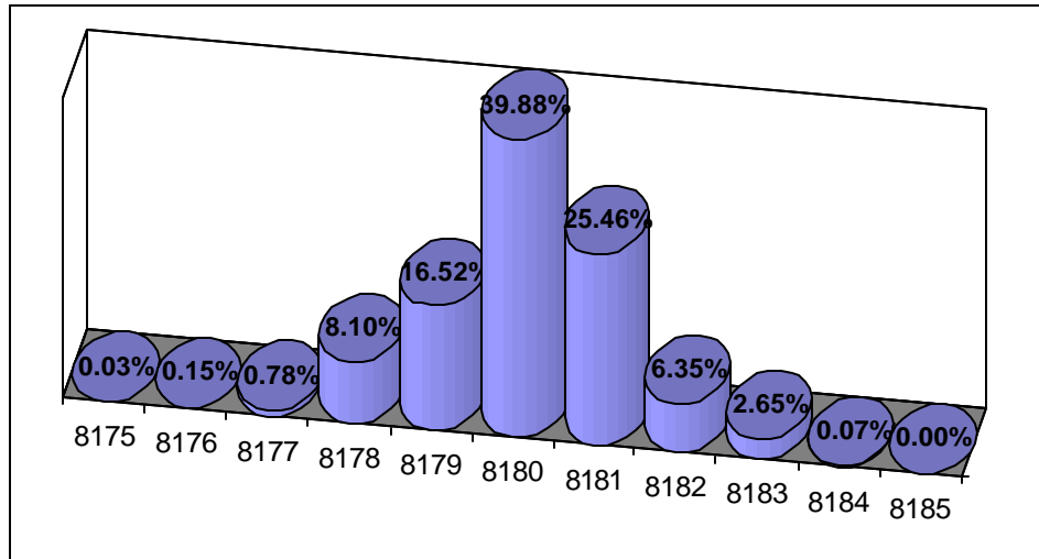
Fig. 2. Histogram of ADC under test with DC input applied (common-mode). The x-axis represents the ADC output code in LSBs, and the height of the barrels the percent hit count for each code in a run of 16384 sample points. The mean of the distribution is 8180 LSBs, indicating an offset of approximately 12 LSBs.
