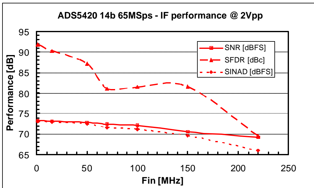
Fig. 10. f_{IN} sweep at 65MSps sampling rate on TI's ADS5420 14 bit 65MSps A-to-D converter for wireless infrastructure applications. The design changes implemented as a result of the application of the jitter measurement technique enabled a dramatic improvement in the ADC's IF performance.
