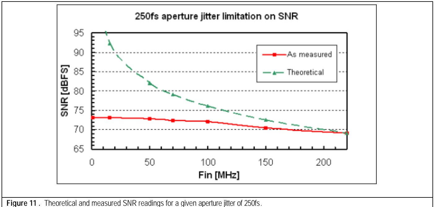
Figure 11 . Theoretical and measured SNR readings for a given aperture jitter of 250fs.
