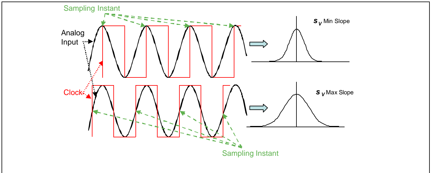
Fig. 1. Sinusoid sampling at different phases: sampling at the top of the input sinewave yields a much tighter output code distribution than sampling the input at its maximum slope (zero-crossing).
