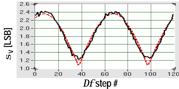
Fig. 4. Total s_V vs. number of Df steps at 30MSps clock rate, 30MHz coherent input: the s_V due to jitter amounts to 2.08LSB. The step between each phase sample is 3^\circ , for a total of 360^\circ .
