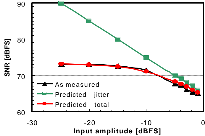
Fig. 8. Measured and predicted SNR vs. A_{IN} at f_{IN} = 150\text{MHz} . The high jitter level overwhelms any other effect, limiting SNR at high A_{IN} .
