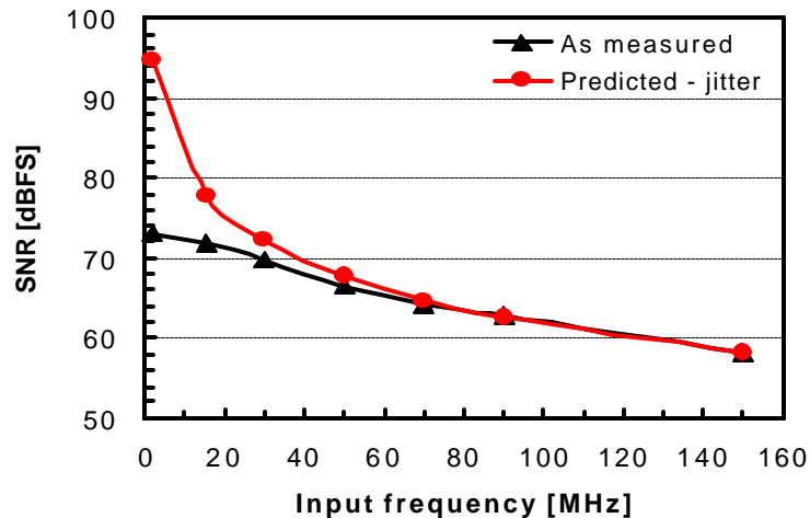
Fig. 7. SNR vs. f_{IN} of a 14b switched-capacitor pipelined ADC, measured at 30MSps, -1dBFS. The SNR is thermal-noise-limited at low f_{IN} , jitter-limited at f_{IN} > 60\text{MHz} (external clock source jitter > 1\text{ps} ).
