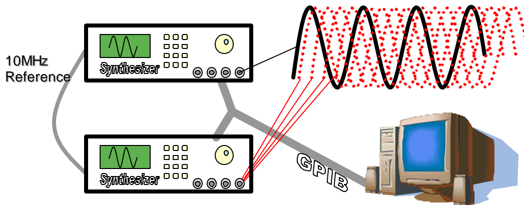
Fig. 3. Typical experimental setup used in order to apply the jitter measurement technique to an ADC. The two synthesizers are connected to the same 10MHz reference for coherency, and through GPIB synchronization commands the relative phase of one synthesizer's output can be incremented in 1^\circ steps.
