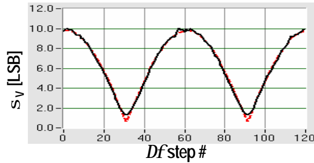
Fig. 5. Total s_V vs. Df steps at 30MSps rate, 90MHz coherent input. The s_V RMS difference is now 5.86LSB.
