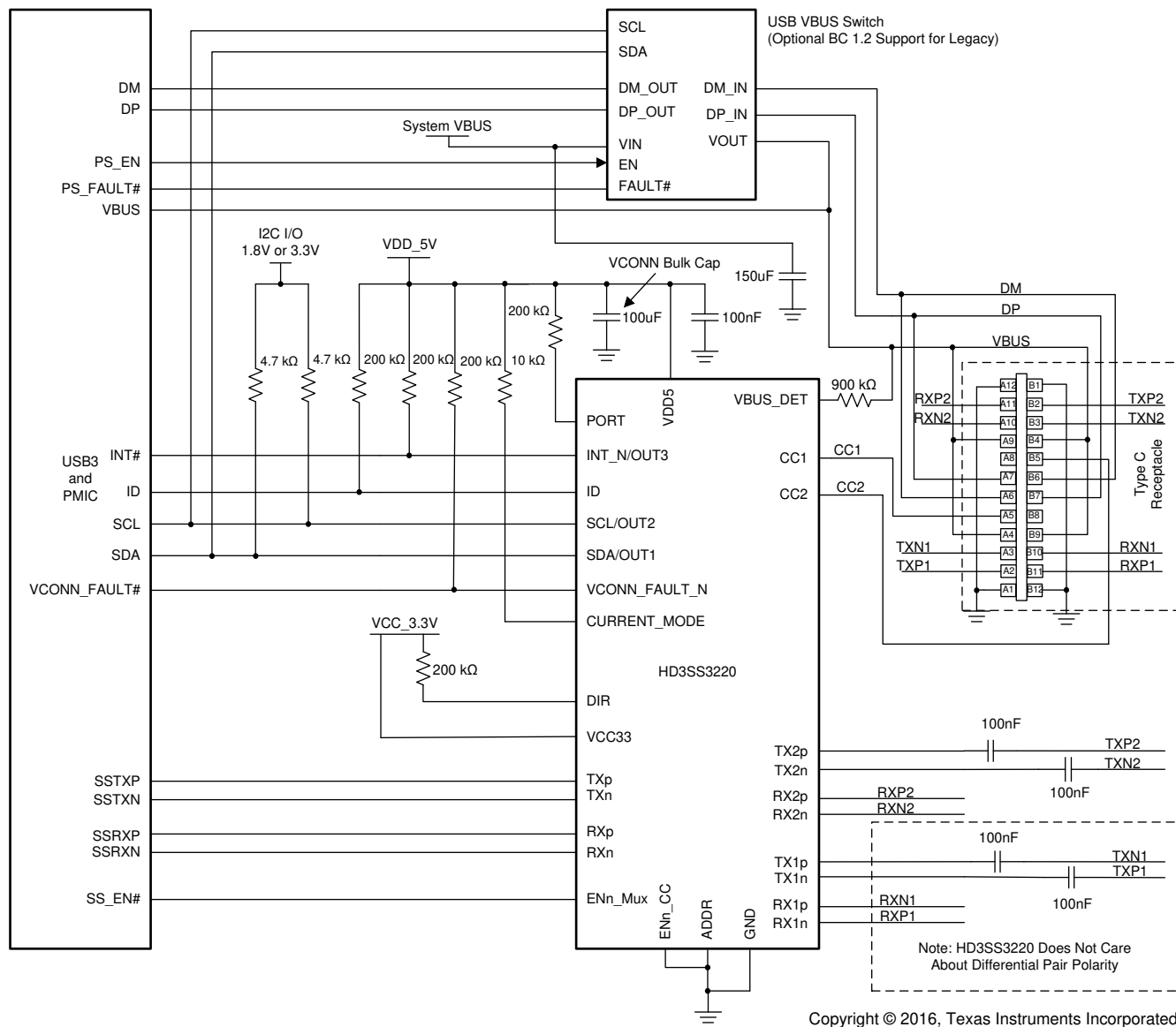
Figure 8-2. DFP Application Using HD3SS3220DFP
