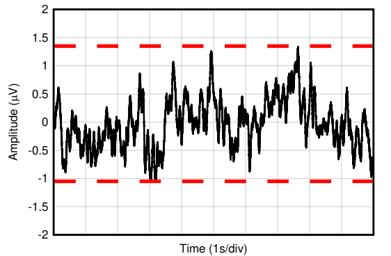
Figure 5-25. 0.1Hz to 10Hz Noise
