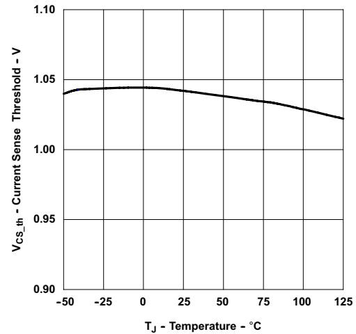
Figure 7-18. Current Sense Threshold Voltage vs Temperature
