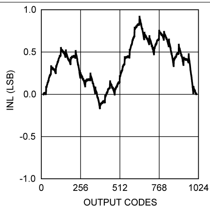
Figure 6. INL at V_A = 5 \text{ V}
