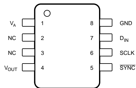
DAC101S101 DGG Package 8-Pin (VSSOP) Top View
