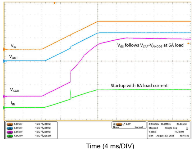
Figure 9-7. Startup With 6-A Load
