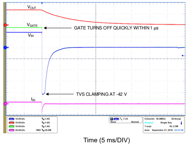
Figure 9-5. Response to ISO 7637-2 Pulse 1
