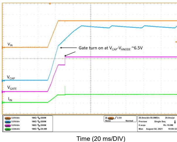
Figure 9-8. VCAP During Startup at 3-A Load
