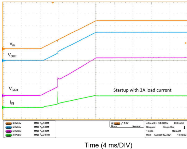
Figure 9-6. Startup With 3-A Load
