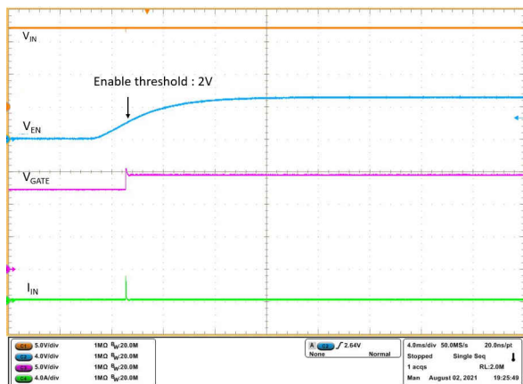
Figure 9-10. Enable Threshold
