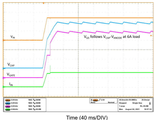
Figure 9-9. VCAP During Startup at 6-A Load
