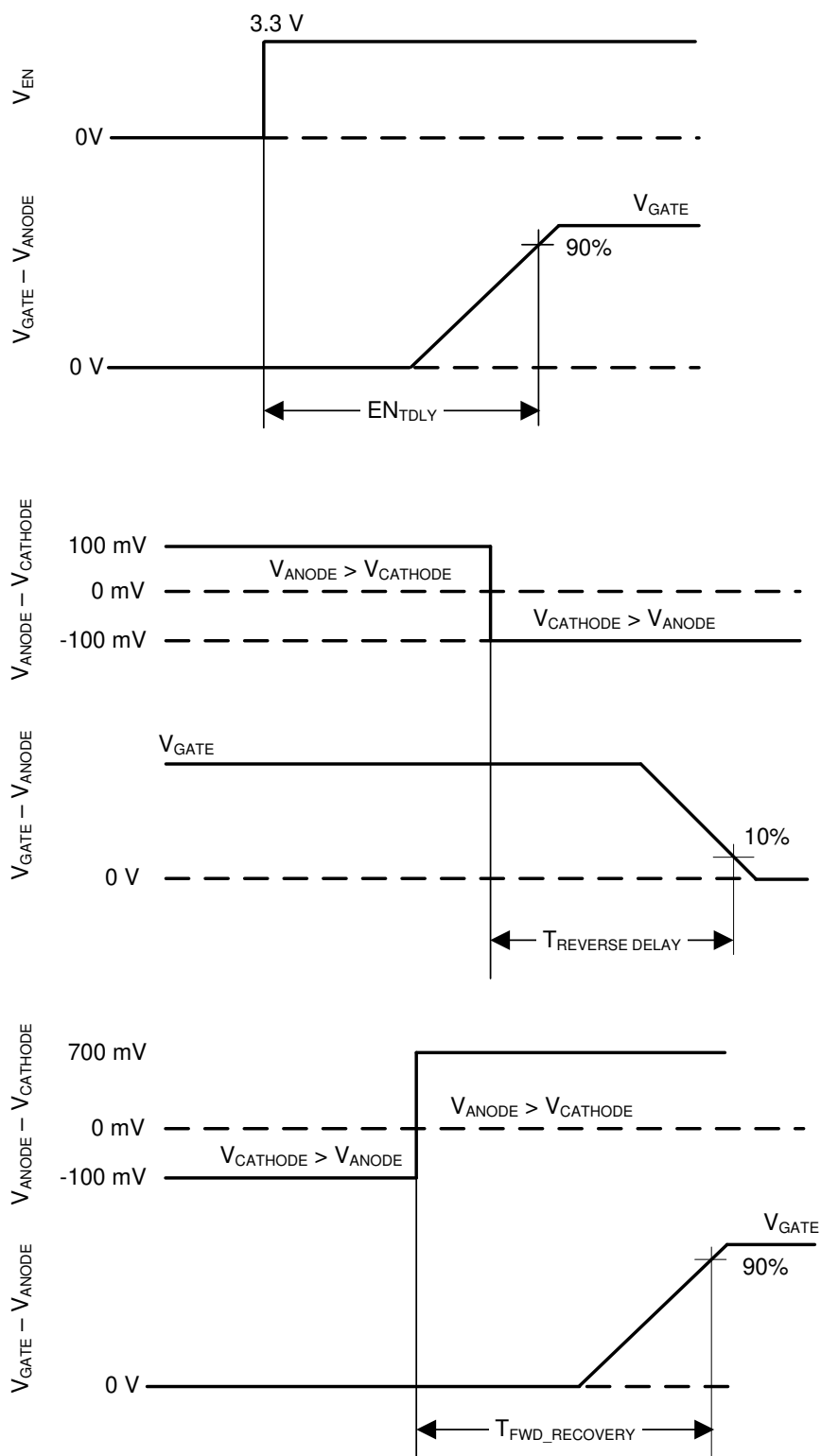
Figure 7-1. Timing Waveforms
