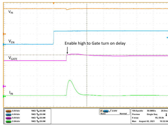
Figure 9-11. Enable Turn ON Delay
