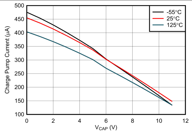
Figure 6-6. Charge Pump V-I Characteristics at V_ANODE >= 12 V
