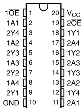
Figure 4-1. SN54AC240 J or W Package; SN74AC240 DB, DW, N, NS, or PW Package (Top View)
