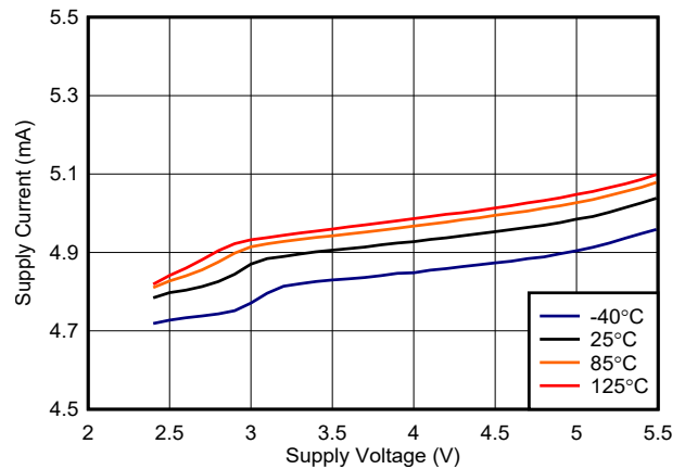
Figure 6-32. TLV3601 Supply Current vs. Voltage (Output High)
