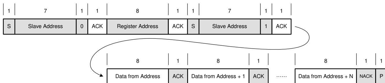
Figure 7-14. Multi-byte Read
