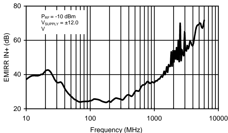
Figure 1. TLE2027 EMIRR IN+ vs Frequency
