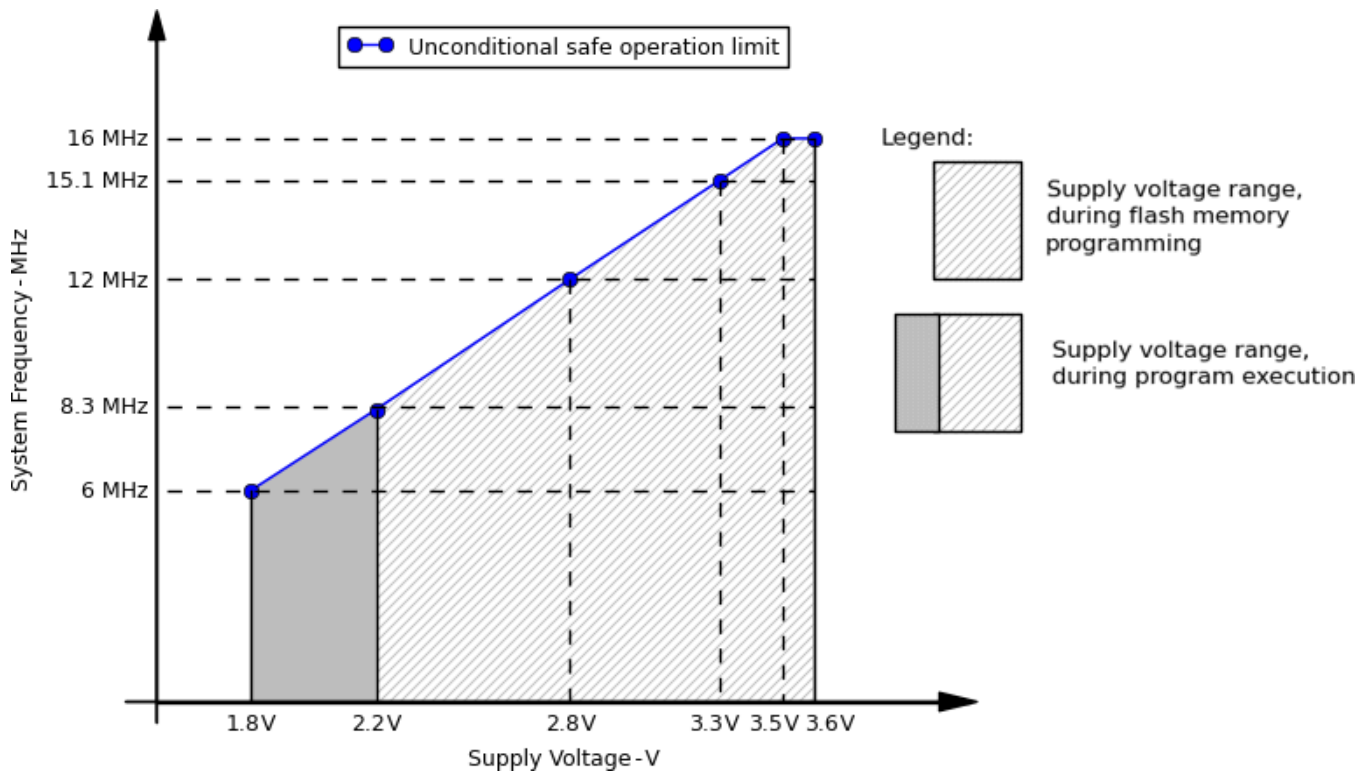
Figure 2. V CC vs Frequency – Safe Operating Conditions for LFXT1 in HF Mode and for Digital External Clock Sources
