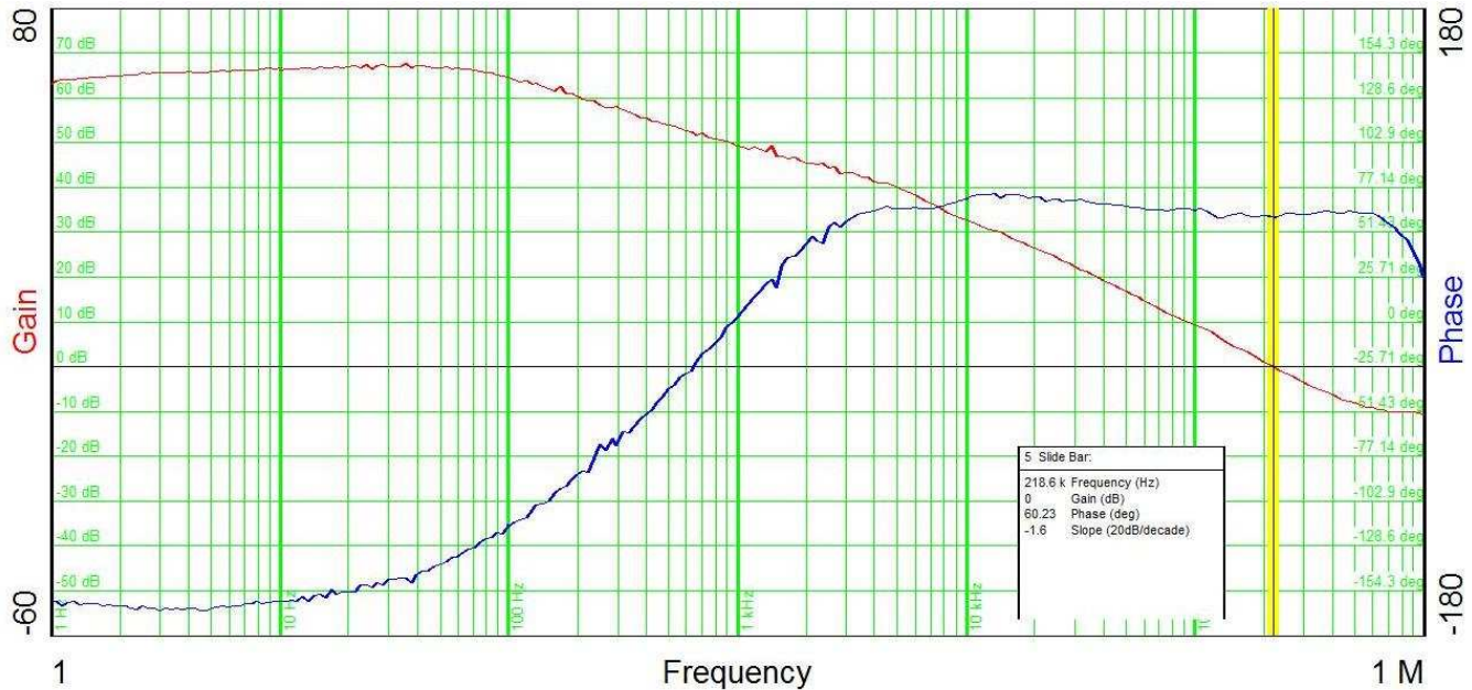
Figure 8. Frequency Response of TPS7H1101A-SP
