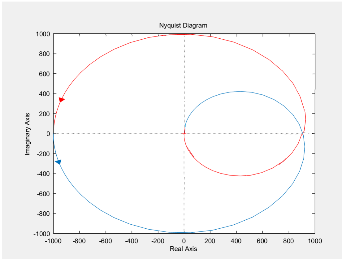
Figure 6. Nyquist Plot Example
