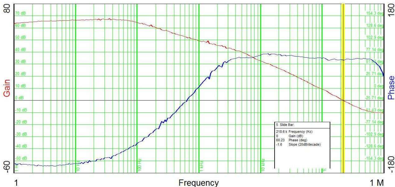
Figure 2. Frequency Response of TPS7H1101A-SP
