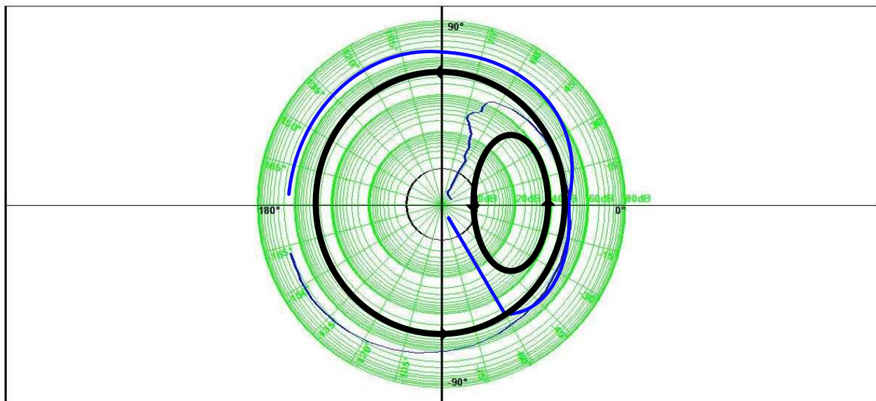
Figure 10. Nyquist Plot of Mirrored Response
