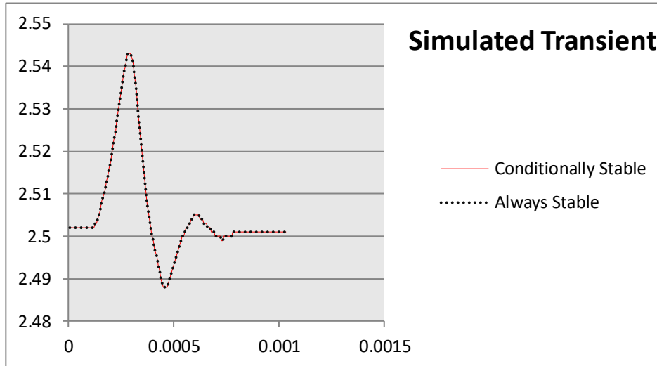
Figure 4. Transient Responses of Models
