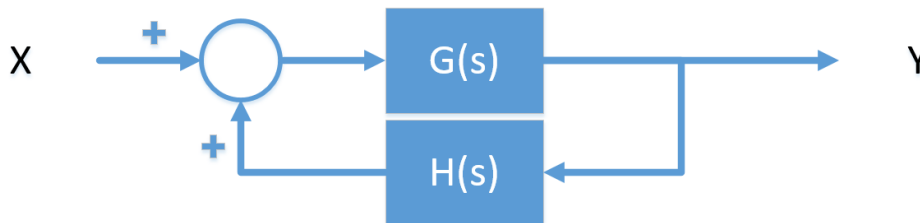
Figure 1. Simple Block Diagram of Control Loop
