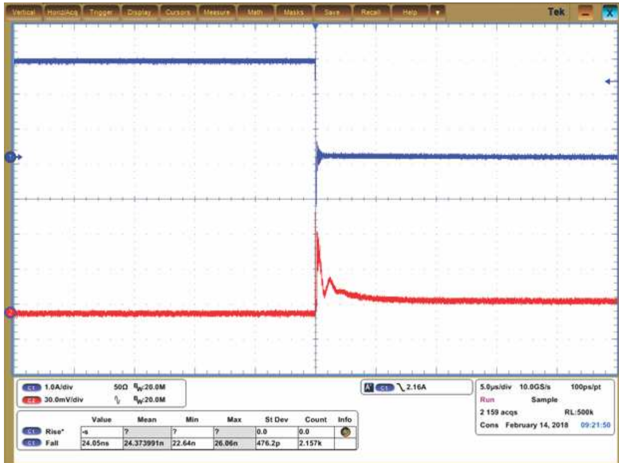
Figure 5. Transient Response of TPS7H1101A-SP
