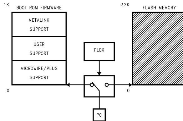
Figure 5. COP8 FLASH Memory Layout
