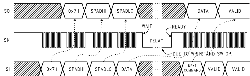
Figure 12. Byte Write Waveform (Relative Bytes are Shown)
