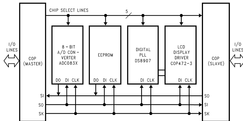
Figure 6. MICROWIRE/PLUS Example
