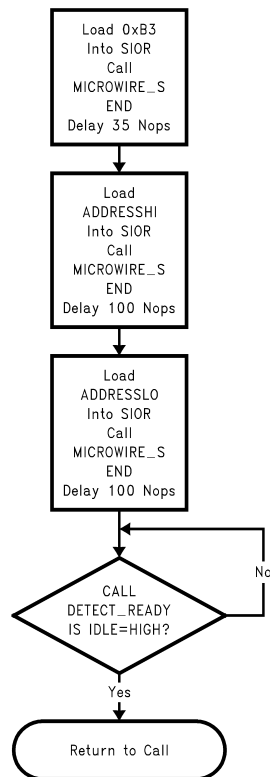
Figure 28. Flow for the Page Erase Function
