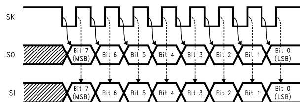
Figure 7. MICROWIRE/PLUS Interface Timing, Normal SK Mode, SK Idle Phase being High
