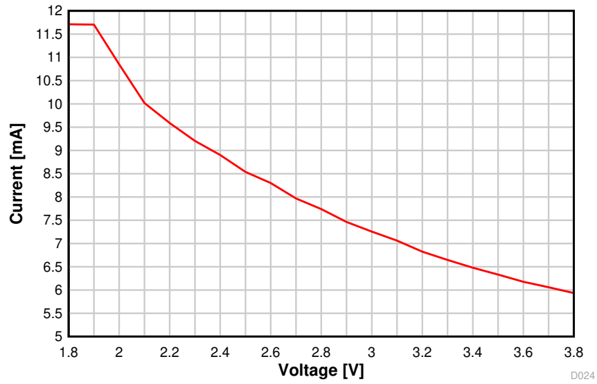
8-16. TX Current vs. Supply Voltage (VDDS) (BLE 1 Mbps, 2.44 GHz)
