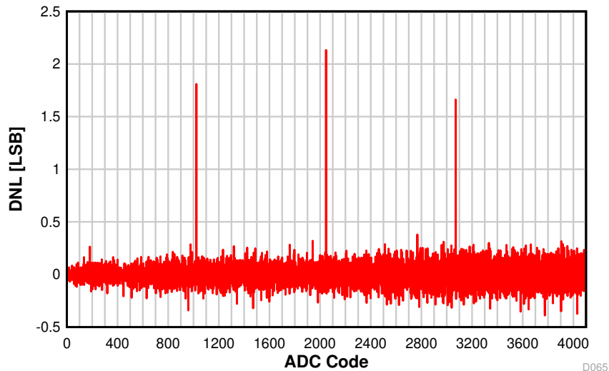
8-46. DNL vs. ADC Code
