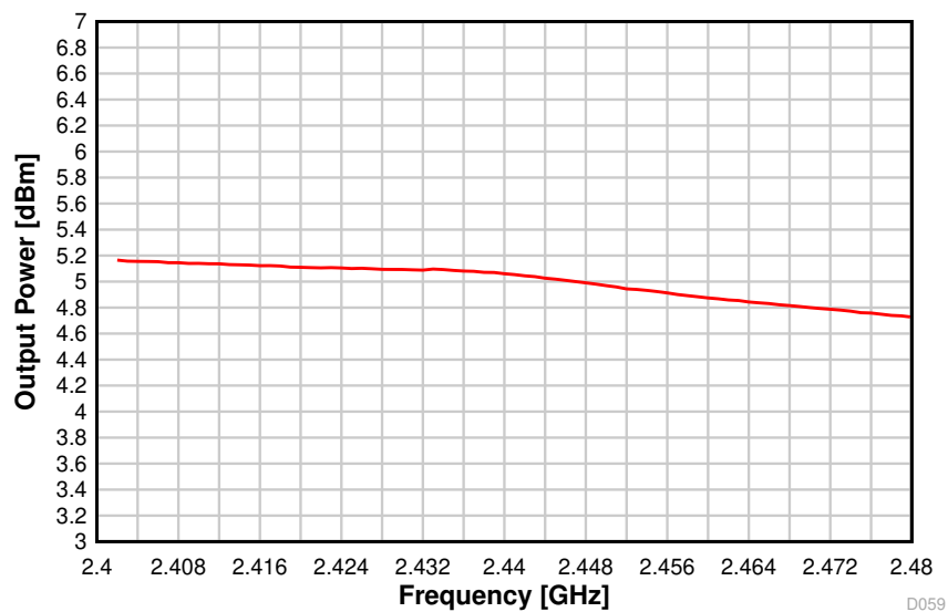
8-42. Output Power vs. Frequency (BLE 1 Mbps, 2.44 GHz, +5 dBm)
