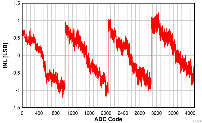
8-45. INL vs. ADC Code
