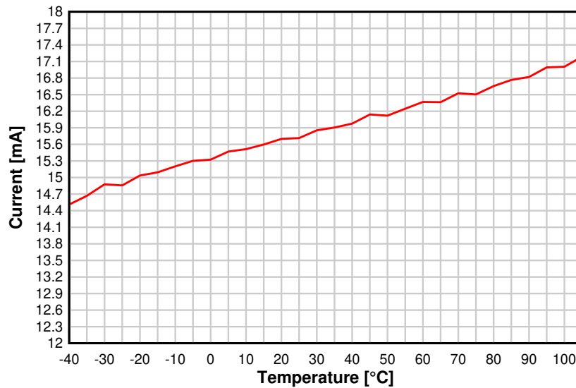
8-12. TX Current vs. Temperature (50 kbps, 868.3 MHz)
