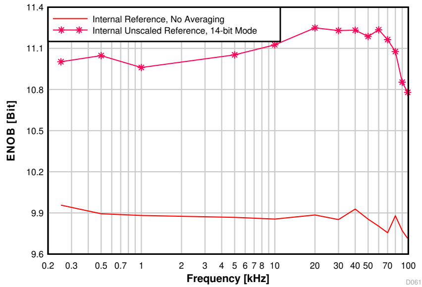
8-43. ENOB vs. Input Frequency
