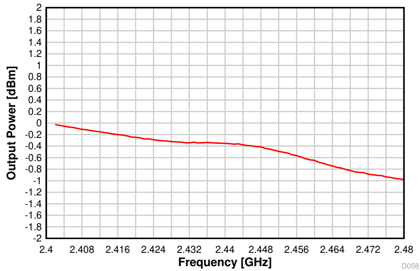
8-41. Output Power vs. Frequency (BLE 1 Mbps, 2.44 GHz)
