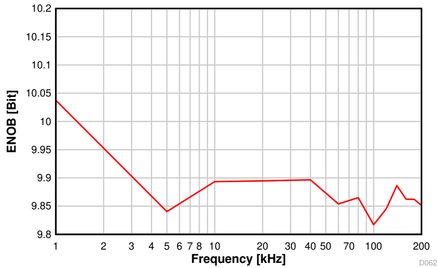
8-44. ENOB vs. Sampling Frequency
