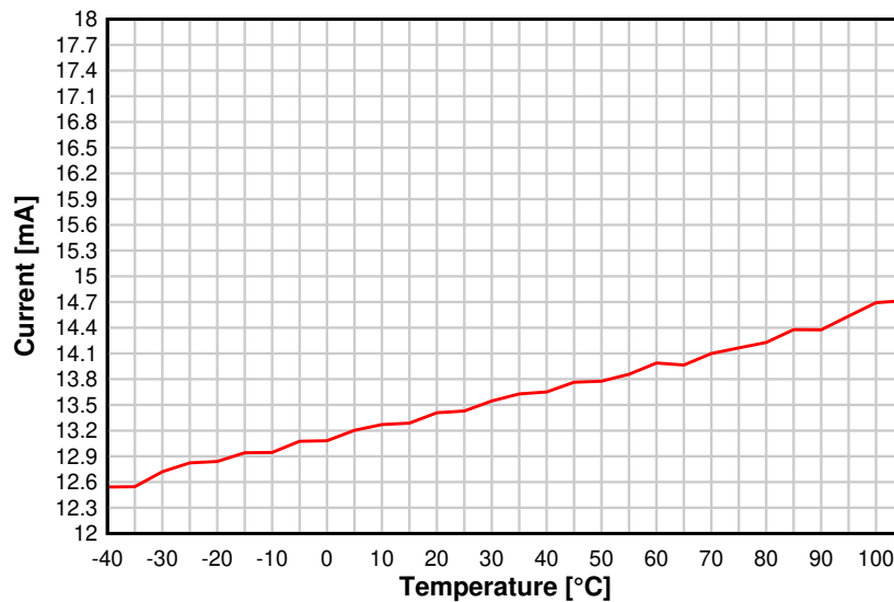
8-13. TX Current vs. Temperature (50 kbps, 868.3 MHz, VDD5 = 3.6 V)
