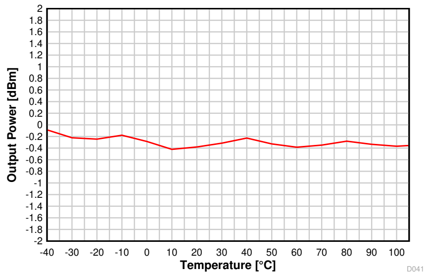
8-34. Output Power vs. Temperature (BLE 1 Mbps, 2.44 GHz)
