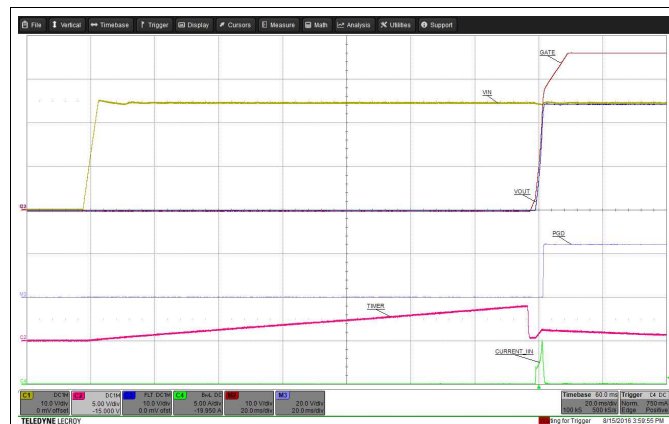
Figure 33. Start-Up
