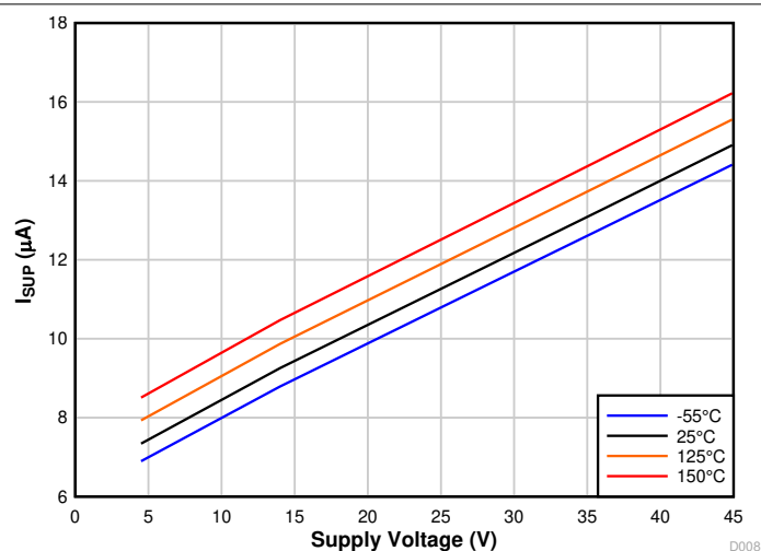
FIG 7-7. Sleep Mode I_{SUP} vs V_{SUP} and Temperature
