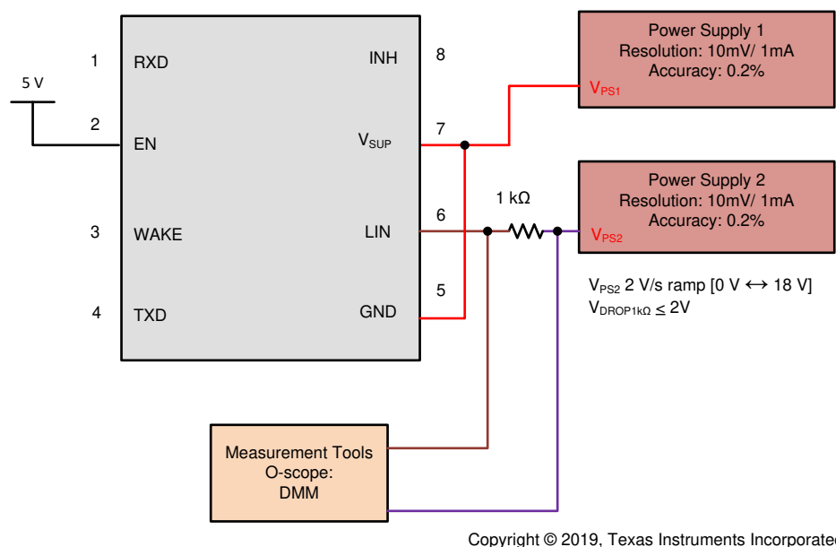
8-9. Test Circuit for I_{BUS\_NO\_GND} Loss of GND
