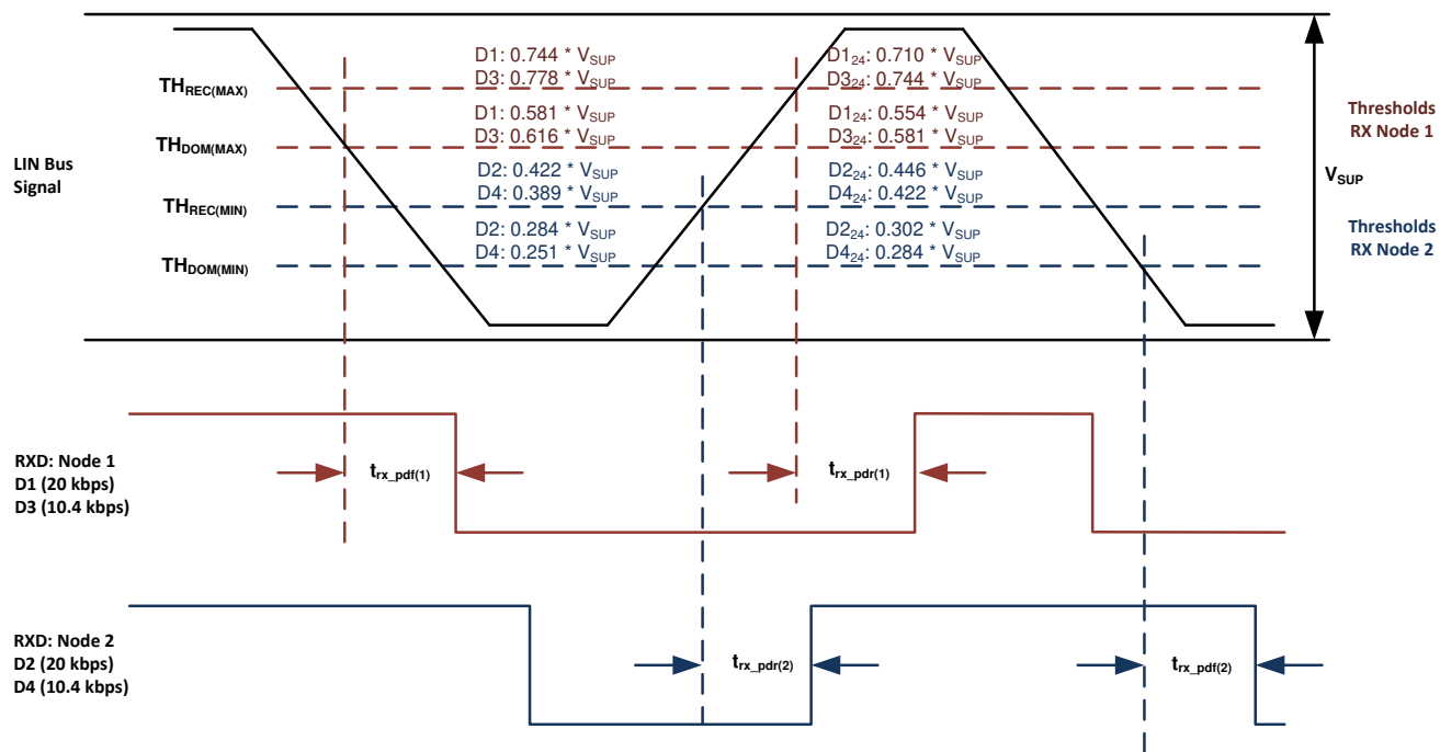
🔍 8-13. Propagation Delay
