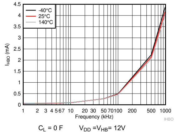
6-5. HB Operating Current
