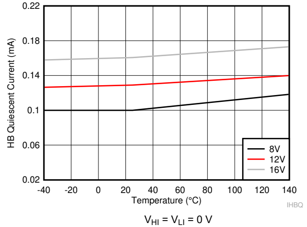
6-3. HB Quiescent Current
