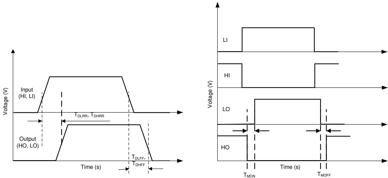
6-1. Timing Diagram
