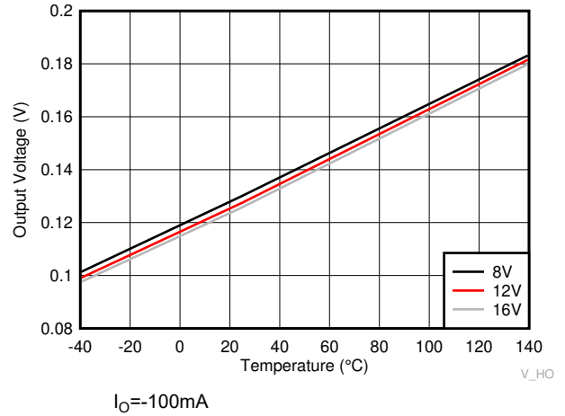
6-15. HO High Output Voltage ( V_{HOH} )
