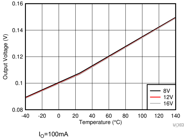
6-14. HO Low Output Voltage ( V_{HOL} )
