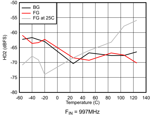
5-37. HD2 vs Temperature
