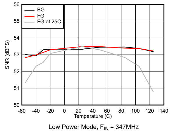
5-40. SNR vs Temperature
