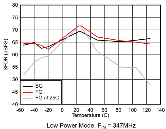
5-41. SFDR vs Temperature
