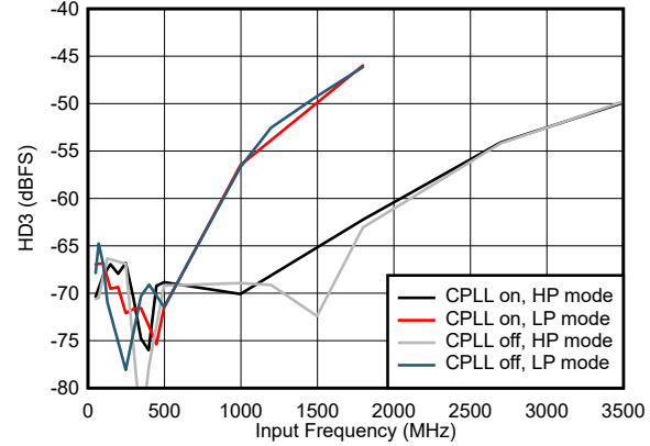
5-70. HD3 vs Input Frequency and CPLL and Power Mode
