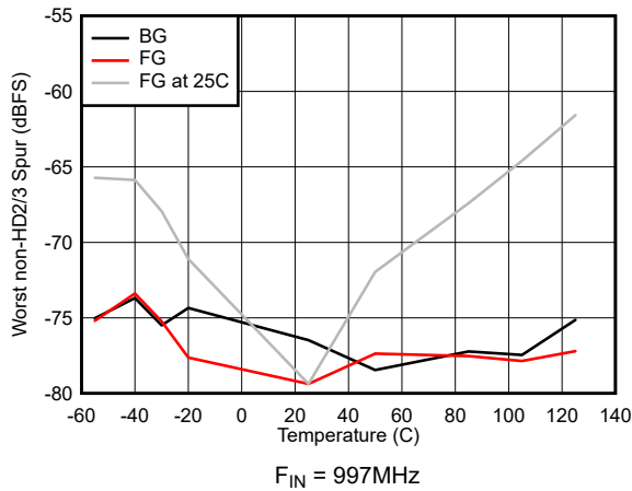
5-39. Worst non-HD2/3 Spur vs Temperature
