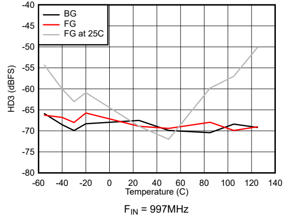
5-38. HD3 vs Temperature
