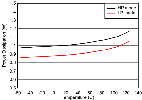
5-113. Quad Channel, Power Dissipation vs Temperature
