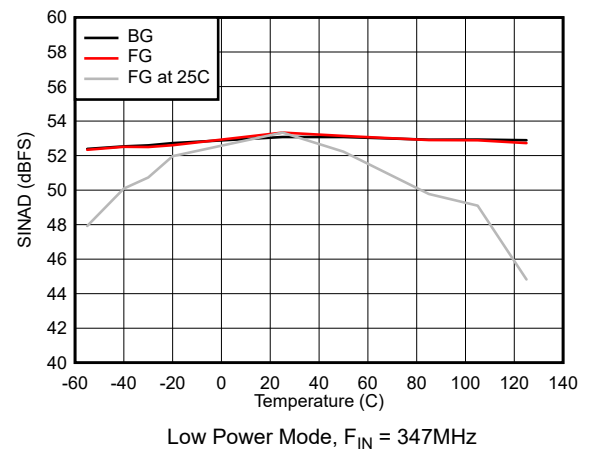
5-42. SINAD vs Temperature
