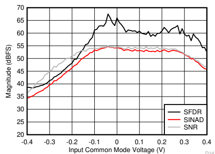
FIG 5-97. SNR, SFDR and SINAD vs Input Common Mode Voltage
