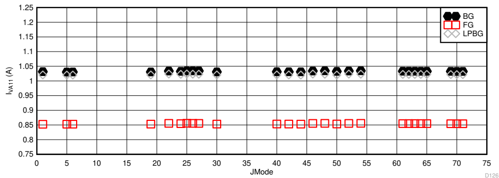
図 5-109. DES Mode: I_{VA19} vs JMODE at 10.4GSPS
