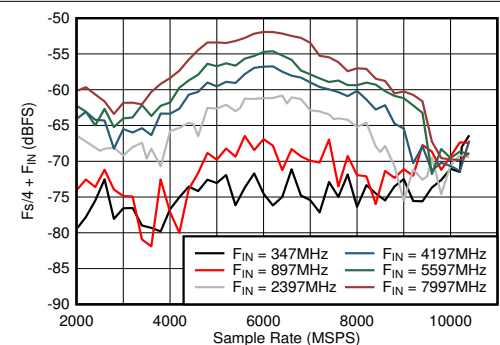
図 5-42. DES Mode: F_s/4 + F_{\text{IN}} vs Sample Rate and Input Frequency
