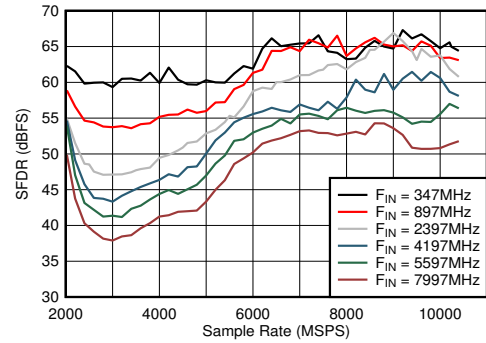
図 5-32. DES Mode: SFDR vs Sample Rate and Input Frequency
