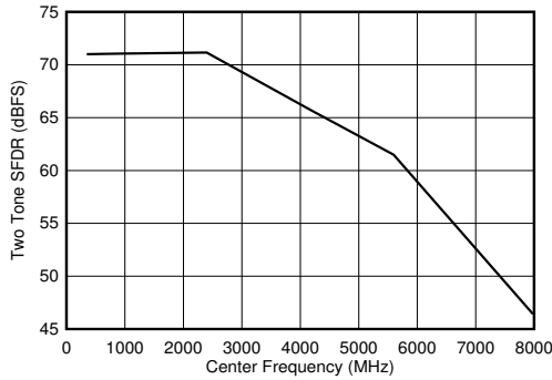
図 5-107. Dual Channel Mode: Two Tone SFDR vs Input Frequency
