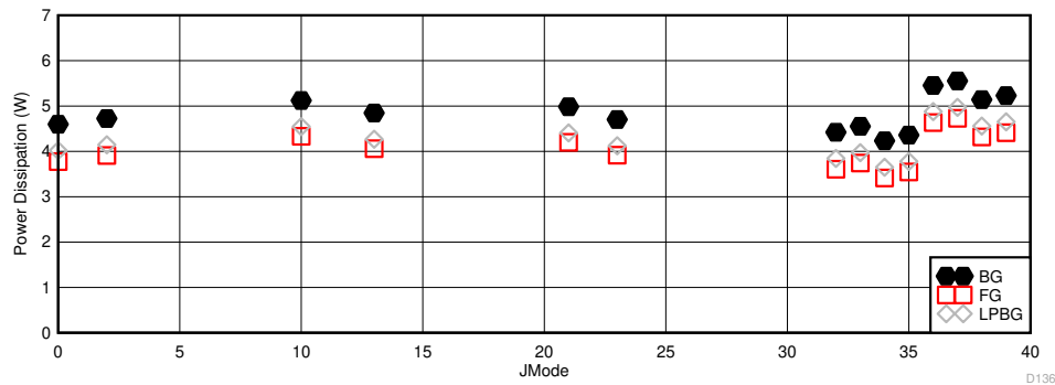
図 5-119. Other Modes with Lower Maximum F_S : I_{D11} vs JMODE
