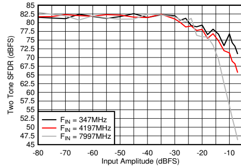
図 5-108. Dual Channel Mode: Two Tone SFDR vs Input Amplitude
