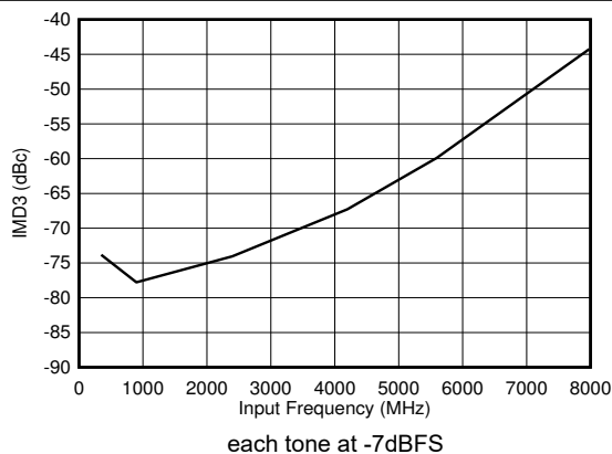
FIG 5-99. DES Mode: IMD3 vs Input Frequency
