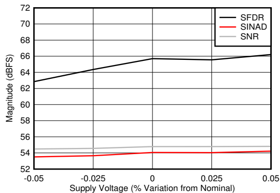
FIG 5-95. Dual Channel Mode: SNR, SINAD and SFDR vs Supply Voltage
