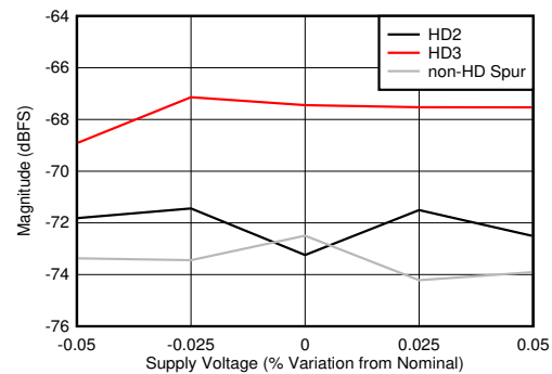
FIG 5-96. Dual Channel Mode: HD2, HD3 and Worst non-HD Spur vs Supply Voltage
