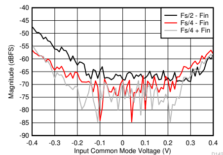
FIG 5-98. F_s/2 - F_{\text{IN}} and F_s/4 \pm F_{\text{IN}} vs Input Common Mode Voltage
