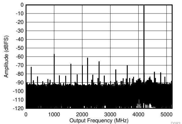
FIG 5-8. DES Mode: Single Tone FFT at 4197 MHz
