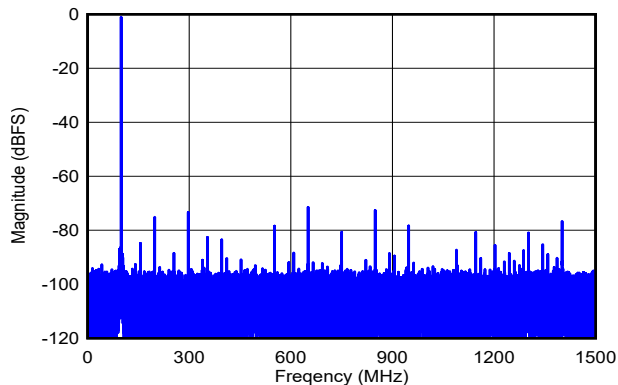
DES_EN = 1, f_S = 3000\text{MHz} , FG calibration, SNR = 57.4dBFS, SFDR = 71.3dBFS, ENOB = 9.0 bits
