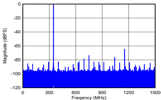
DES_EN = 1, f_S = 3000\text{MHz} , FG calibration, SNR = 57.6dBFS, SFDR = 64.2dBFS, ENOB = 9.1 bits
