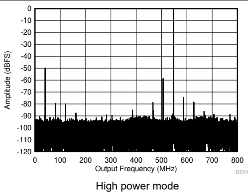
5-11. Single Tone FFT at 3797 MHz and -1 dBFS
