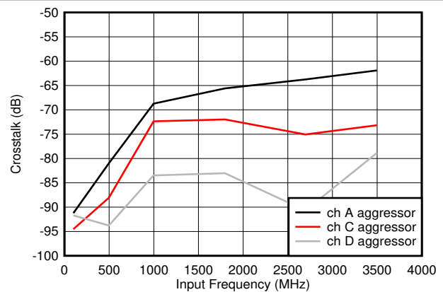
図 5-78. Crosstalk to Channel B vs F_{IN}
