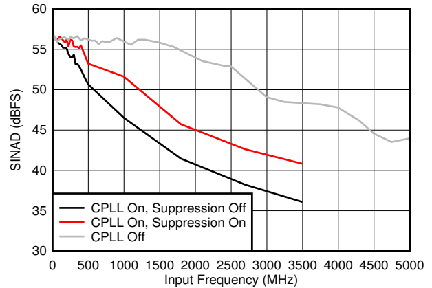
5-42. SINAD vs F_{IN} and C-PLL modes
