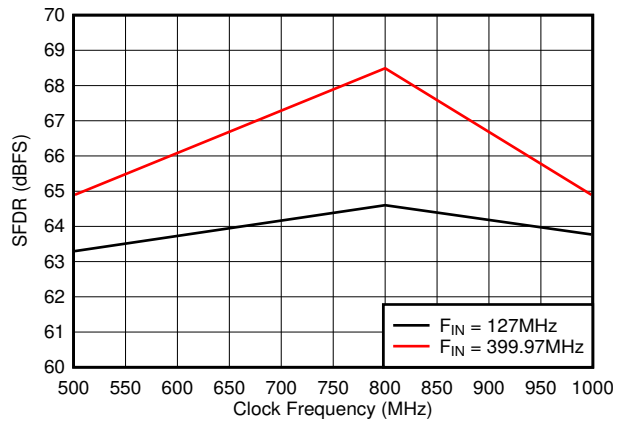
图 5-29. SFDR vs Sample Rate
