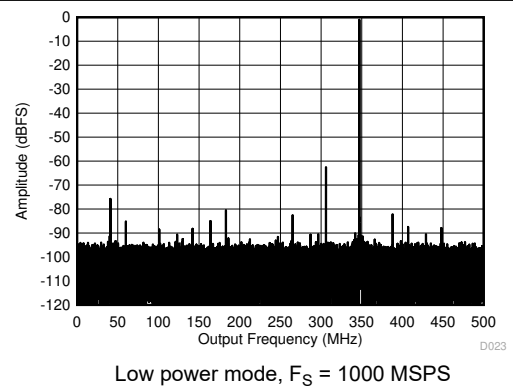
5-12. Single Tone FFT at 347 MHz and -1 dBFS
