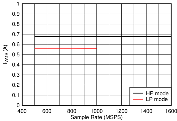
図 5-83. Quad Channel, I_{VA19} vs F_S
