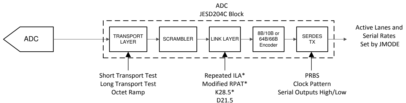
Figure 6-12. Test Mode Insertion Points
