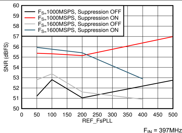
Figure 5-38. SNR vs F_{REF} and Suppression
