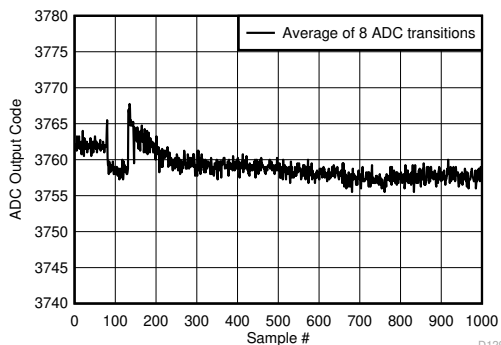
✎ 5-125. Background Calibration Core Transition (offset voltage)
