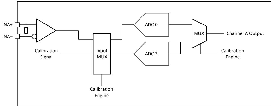
6-15. Single Channel Calibration System Block Diagram
