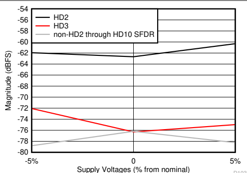
Figure 5-63. HD2, HD3 and Worst non-HD Spur vs Supply Voltage
