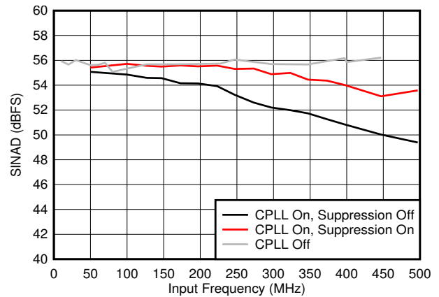
図 5-46. SINAD vs F_{IN} and C-PLL modes
