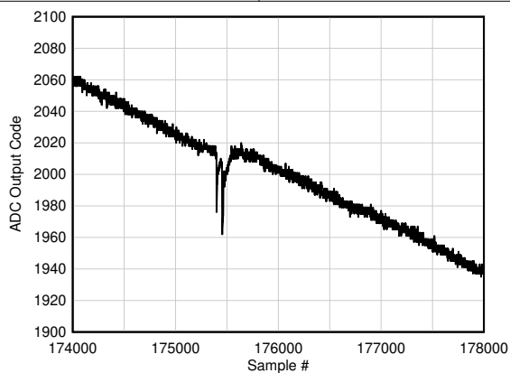
✎ 5-125. Background Calibration Core Transition (offset voltage)
