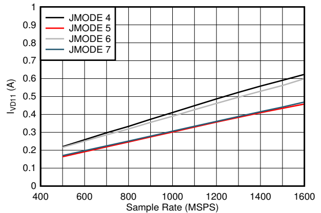
図 5-84. Quad Channel, I_{VDD11} vs F_S
