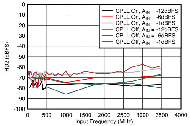
図 5-52. HD2 vs A_{IN} and C-PLL
