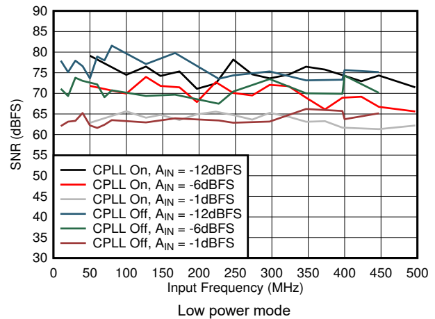
図 5-54. SFDR vs A_{IN} and C-PLL
