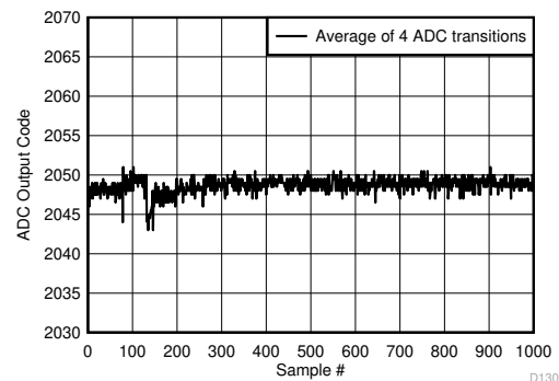
BG Calibration, midscale input voltage, ADC_SRC_DLY=31, MUX_DLY=30
