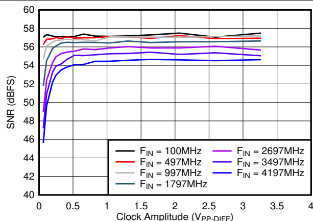
Figure 5-37. SNR vs A_{CLK}
