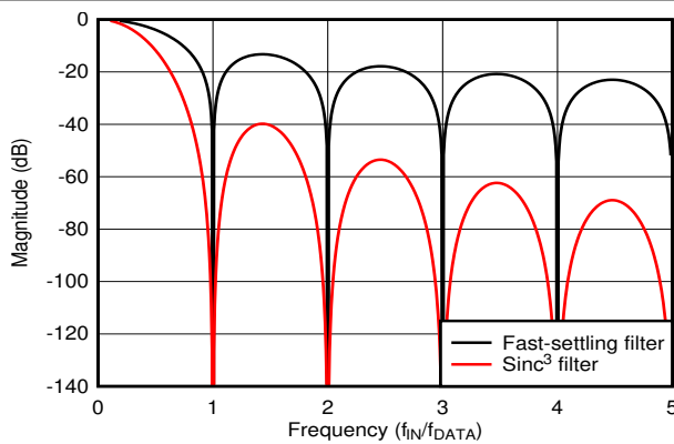
图 8-4. Fast-Settling and Sinc 3 Digital Filter Response
