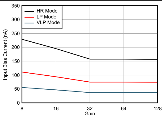
FIG 6-4. Input Bias Current vs Gain
