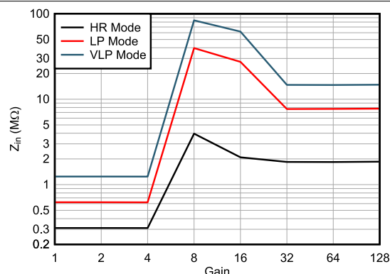
FIG 6-5. Input Impedance vs Gain
