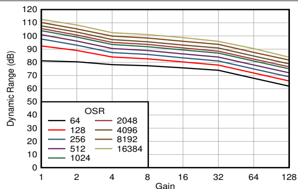
6-23. Dynamic Range vs Gain
