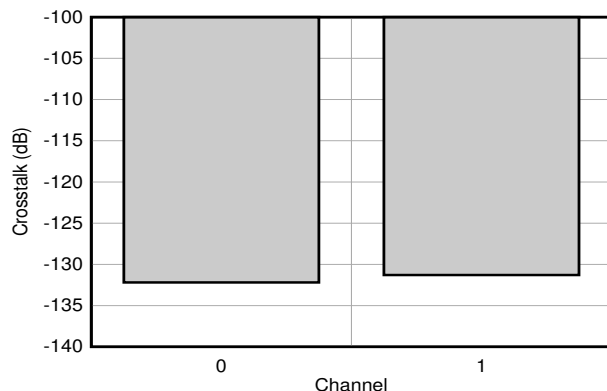
6-24. Crosstalk vs Channel
