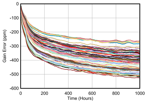
图 6-10. Long-Term Gain Drift
