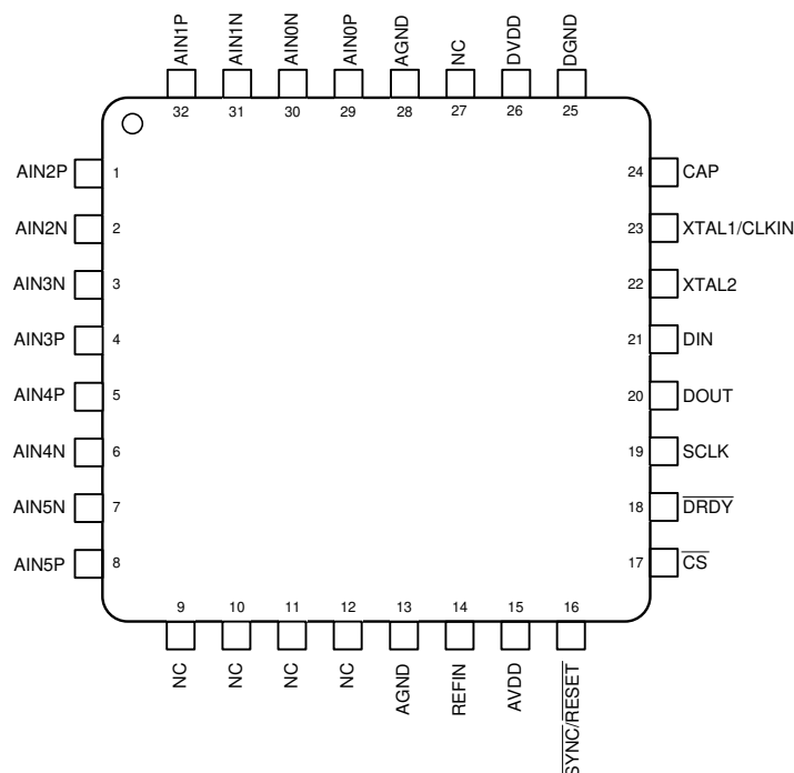
図 5-1. PBS Package, 32-Pin TQFP (Top View)
