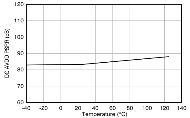
图 6-13. DC AVDD PSRR vs Temperature
