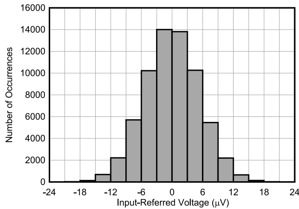
FIG 6-16. Single Device Noise Histogram at 4 kSPS
