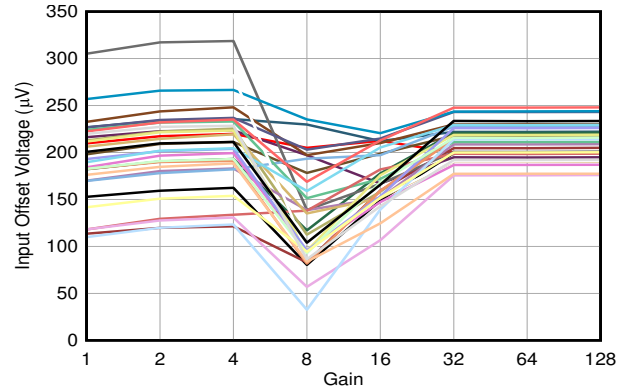
FIG 6-7. Input Offset Voltage vs Gain
