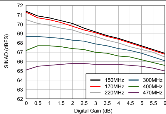
图 6-15. SINAD vs Gain And Input Frequency
