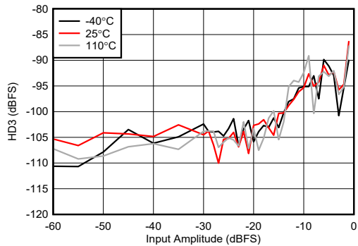
FIG 4-438. RX HD3 vs Digital Amplitude at 8.1GHz
