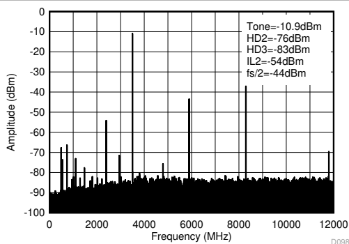
4-148. TX Single Tone (–12dBFS) Output Spectrum at 3.5GHz (0- f_{\text{DAC}} )
