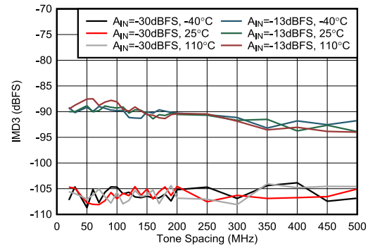
FIG 4-431. RX IMD3 vs Tone Spacing at 8.1GHz
