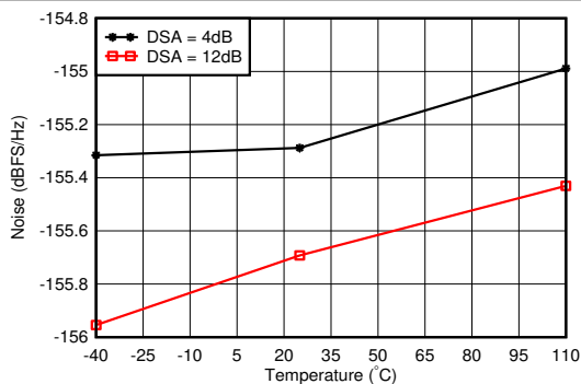
FIG 4-405. RX Noise Spectral Density vs Temperature at 4.9GHz
