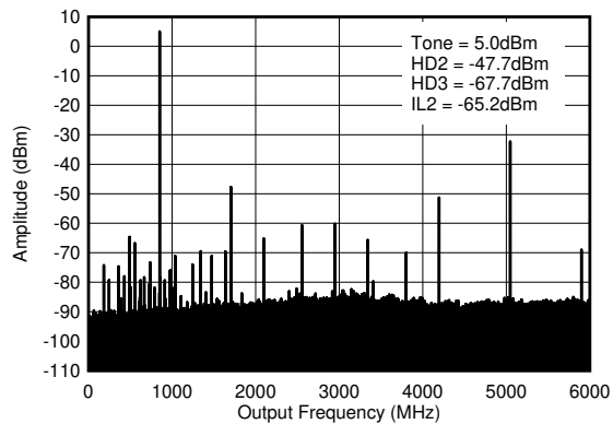
図 4-43. TX Single Tone (-1dBFS) Output Spectrum at 0.85GHz (0- f_{\text{DAC}} )
