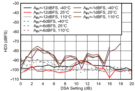
FIG 4-439. RX HD3 vs DSA Setting at 8.1GHz
