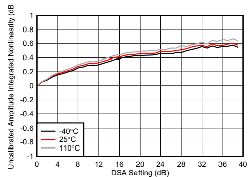
4-193. TX DSA Uncalibrated Amplitude Integrated Nonlinearity at 8.1GHz
