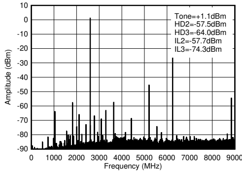
図 4-114. TX Single Tone (-12dBFS) Output Spectrum at 2.6GHz ( 0-f_{\text{DAC}} )
