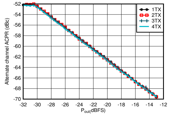
4-34. TX 20-MHz LTE alt-ACPR vs Digital Level at 0.85GHz
