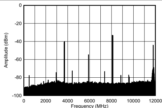
FIG 4-211. TX Dual Tone Output Spectrum at 8.11GHz
