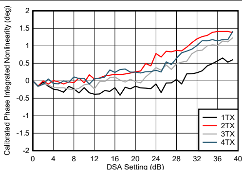
FIG 4-200. TX DSA Calibrated Phase Integrated Nonlinearity at 8.1GHz
