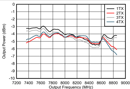
FIG 4-184. TX Output Power vs Frequency at 8.1GHz
