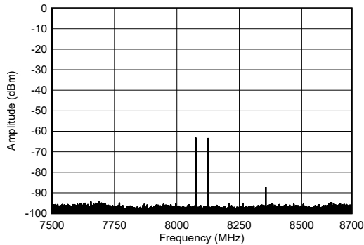
FIG 4-214. TX Dual Tone Output Spectrum at 8.11GHz
