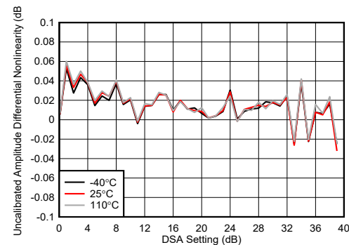
FIG 4-189. TX DSA Uncalibrated Amplitude Differential Nonlinearity at 8.1GHz
