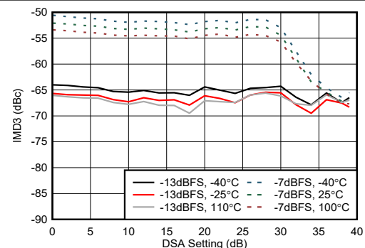
FIG 4-254. TX IMD3 vs DSA Setting at 9.61GHz
