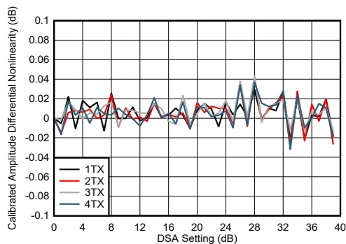
FIG 4-188. TX DSA Calibrated Amplitude Differential Nonlinearity at 8.1GHz
