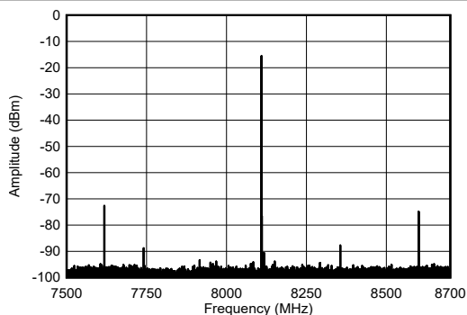
FIG 4-208. TX Single Tone Output Spectrum at 8.11GHz
