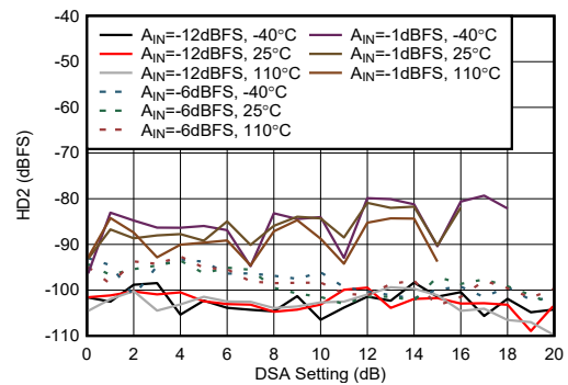
FIG 4-437. RX HD2 vs DSA Setting at 8.1GHz
