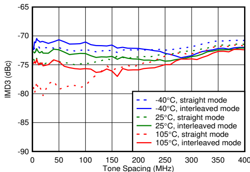
FIG 4-99. TX IMD3 vs Tone Spacing and Temperature at 2.6GHz
