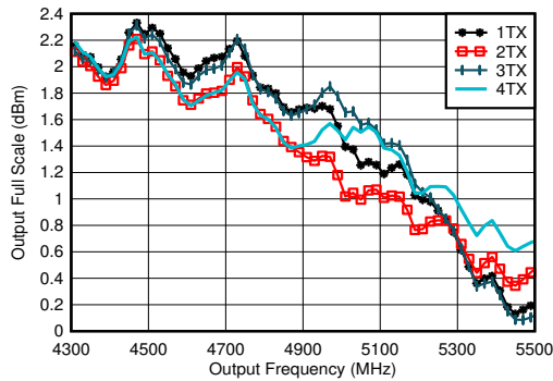
図 4-149. TX Full Scale vs RF Frequency and Channel at 11796.48MSPS
