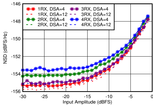
FIG 4-352. RX Noise Spectral Density vs Input Amplitude and Channel at 2.6GHz
