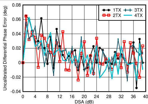
図 4-124. TX Uncalibrated Differential Phase Error vs DSA Setting and Channel at 3.5GHz
