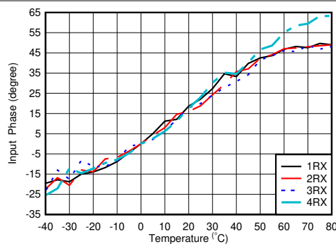
FIG 4-395. RX Input Phase vs Temperature and DSA at f_{\text{OUT}} = 4.9\text{GHz}
