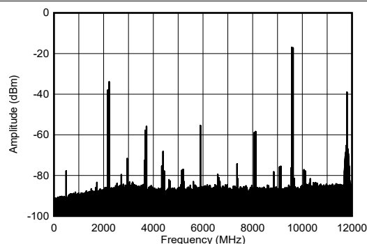
図 4-272. TX 2-Tone Spectrum at 9.61GHz and -7dBFS (wideband)
