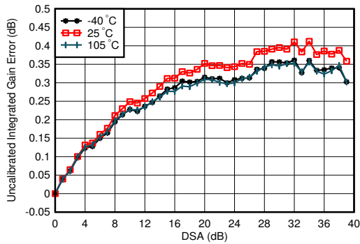
图 4-130. TX Uncalibrated Integrated Gain Error vs DSA Setting and Temperature at 3.5GHz
