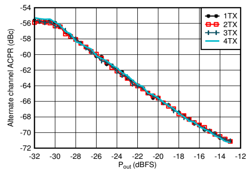
4-176. TX 20MHz LTE alt-ACPR vs Digital Level at 4.9GHz
