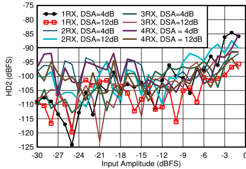
FIG 4-334. RX HD2 vs DSA Setting and Channel at 1.9 GHz
