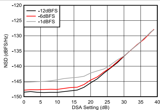
Figure 4-262. TX NSD vs DSA Setting at 9.61GHz
