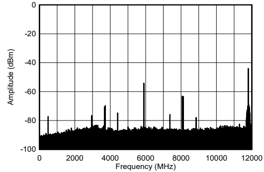
FIG 4-215. TX Dual Tone Output Spectrum at 8.11GHz
