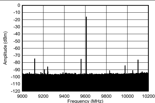
図 4-269. TX Single Tone Spectrum at 9.61GHz and -6dBFS (1.2GHz BW)
