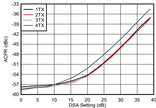
FIG 4-226. TX NR100MHz ACPR vs DSA Setting 8.1GHz
