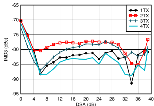
FIG 4-63. TX IMD3 vs DSA Setting at 1.8GHz
