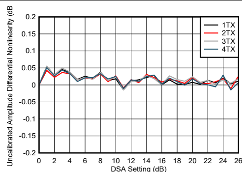
FIG 4-236. TX DSA Uncalibrated Amplitude Differential Nonlinearity
