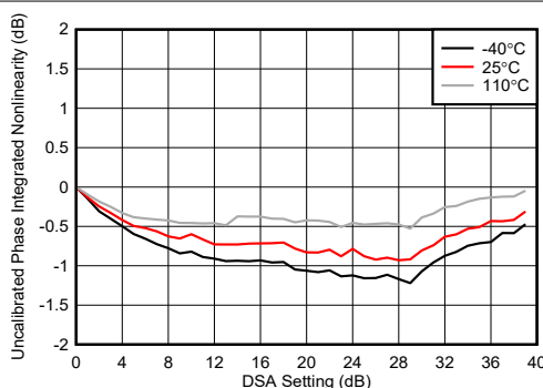
FIG 4-201. TX DSA Uncalibrated Phase Integrated Nonlinearity at 8.1GHz
