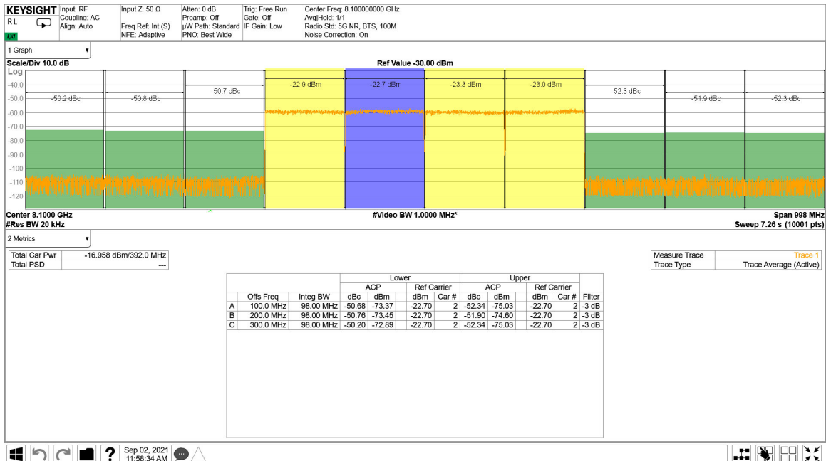
4-231. TX 4x100MHz NR Output Spectrum 8.1GHz
