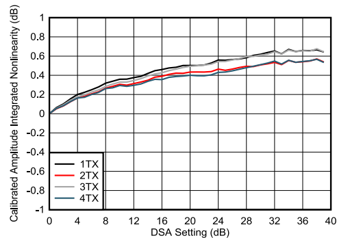
4-192. TX DSA Calibrated Amplitude Integrated Nonlinearity at 8.1GHz
