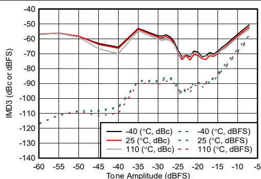
FIG 4-253. TX IMD3 vs Digital Amplitude at 9.61GHz
