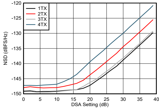
Figure 4-263. TX NSD vs DSA Setting at 9.61GHz
