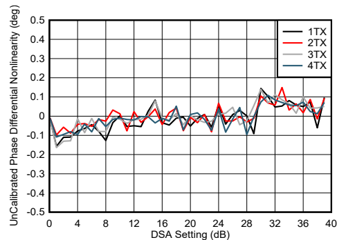
4-195. TX DSA Uncalibrated Phase Differential Nonlinearity at 8.1GHz
