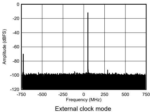
図 4-442. RX Single Tone Output FFT at 8.1GHz, -12dBFS
