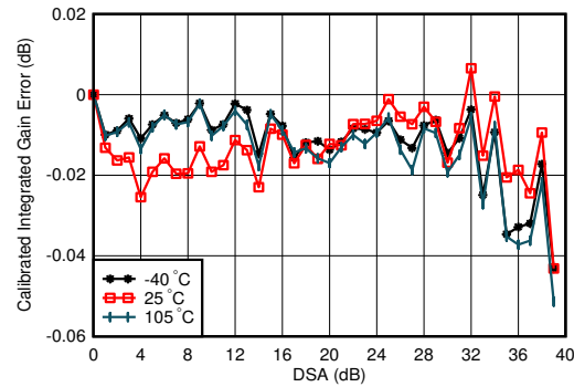
图 4-131. TX Calibrated Integrated Gain Error vs DSA Setting and Temperature at 3.5GHz
