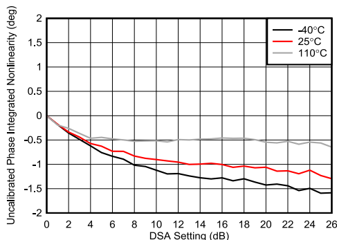
4-250. TX DSA Uncalibrated Phase Integrated Nonlinearity
