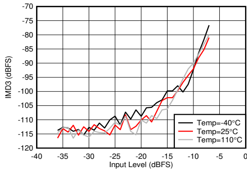
FIG 4-354. RX IMD3 vs Input Level and Temperature at 2.6GHz
