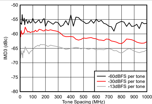
Figure 4-258. TX IMD3 vs Tone Spacing at 9.61GHz
