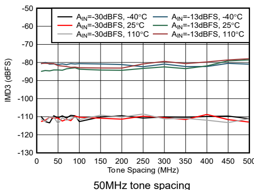
図 4-458. RX IMD3 vs Tone Spacing at 9.6GHz
