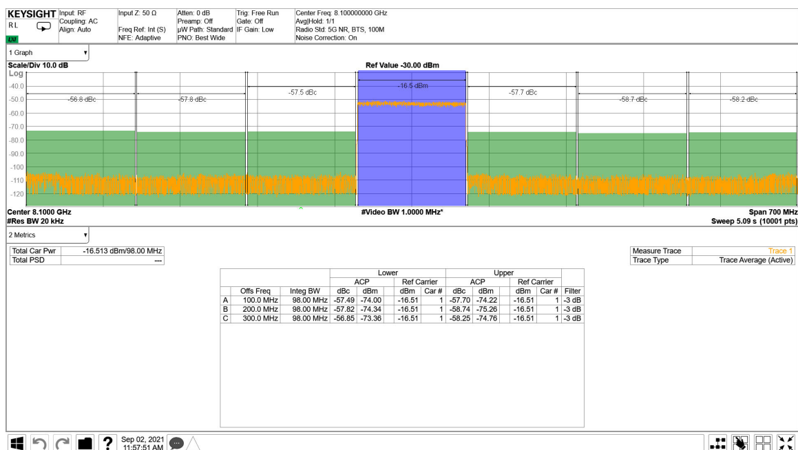
FIG 4-229. TX 100MHz NR Output Spectrum at 8.1GHz
