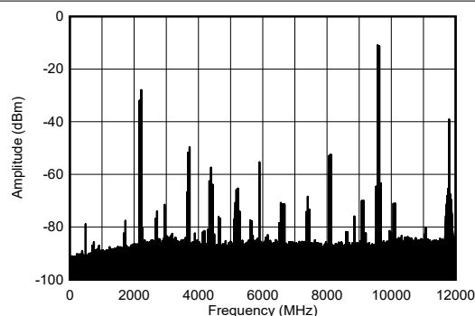
図 4-270. TX Single Tone Spectrum at 9.61GHz and -12dBFS (wideband)
