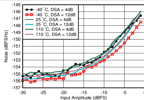
FIG 4-406. RX Noise Spectral Density vs Input Amplitude and Temperature at 4.9GHz
