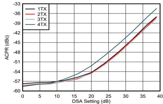
FIG 4-227. TX NR100MHz alt-ACPR vs DSA Setting 8.1GHz
