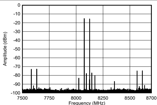
FIG 4-210. TX Dual Tone Output Spectrum at 8.11GHz
