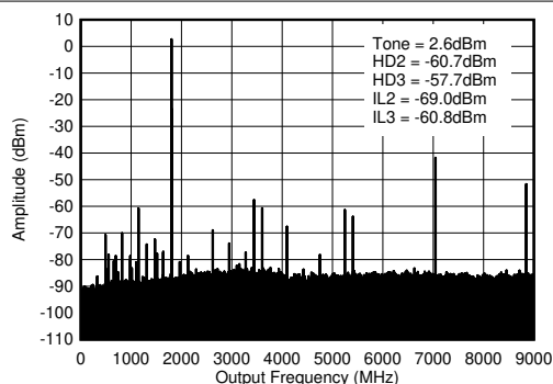
図 4-75. TX Single Tone (-12 dBFS) Output Spectrum at 1.8GHz ( 0-f_{\text{DAC}} )
