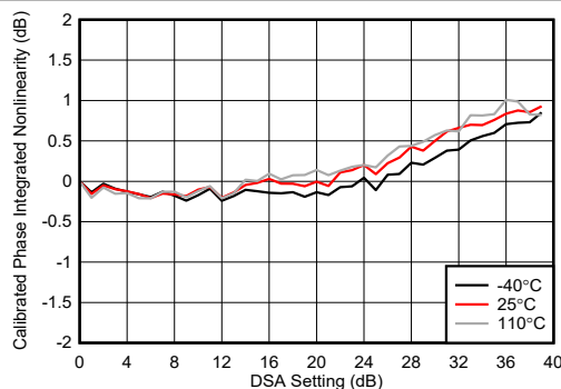
FIG 4-202. TX DSA Calibrated Phase Integrated Nonlinearity at 8.1GHz
