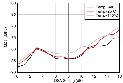
FIG 4-353. RX IMD3 vs DSA Setting and Temperature at 2.6GHz
