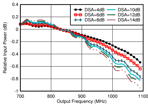
FIG 4-285. RX In-Band Gain Flatness for Channel 1RX, f_{\text{IN}} = 830\text{MHz}
