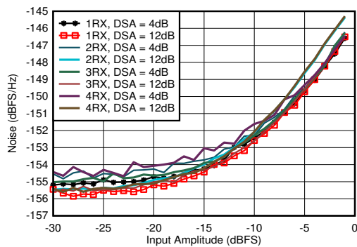
FIG 4-330. RX Noise Spectral Density vs Input Amplitude and Channel at 1.75GHz
