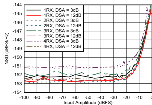
FIG 4-433. RX NSD vs Digital Amplitude at 8.1GHz
