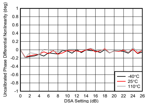
4-246. TX DSA Uncalibrated Phase Differential Nonlinearity
