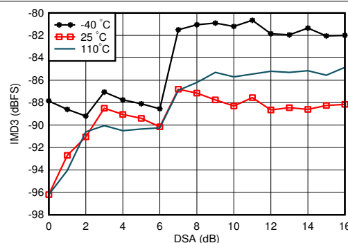
FIG 4-300. RX IMD3 vs DSA Setting and Temperature at 0.8GHz
