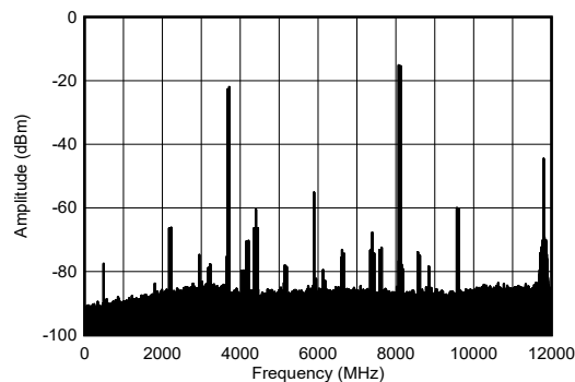
FIG 4-209. TX Dual Tone Output Spectrum at 8.11GHz
