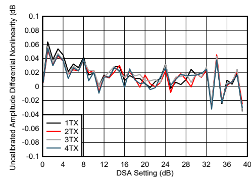
FIG 4-187. TX DSA Uncalibrated Amplitude Differential Nonlinearity at 8.1GHz
