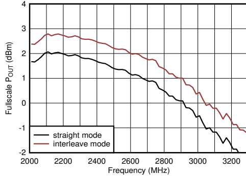
FIG 4-78. TX Full Scale vs RF Frequency at 11796.48MSPS
