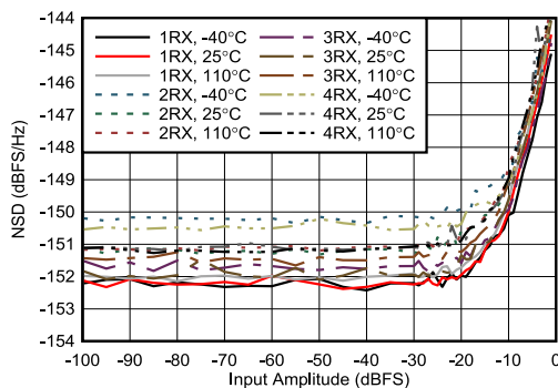
FIG 4-432. RX NSD vs Digital Amplitude at 8.1GHz
