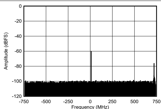
FIG 4-468. RX Single Tone Output FFT at 9.61GHz
