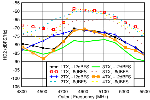
図 4-179. TX HD2 vs Digital Amplitude and Output Frequency at 4.9GHz
