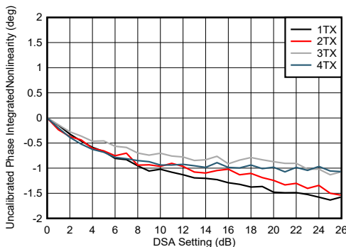
4-248. TX DSA Uncalibrated Phase Integrated Nonlinearity
