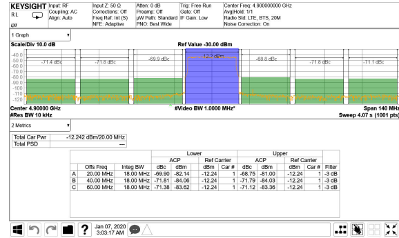
4-174. TX 20MHz LTE Output Spectrum at 4.9GHz
