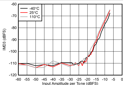
図 4-455. RX IMD3 vs Digital Amplitude at 9.6GHz
