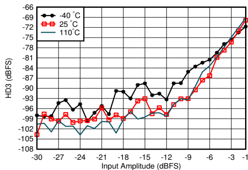
FIG 4-417. RX HD3 vs Input Level and Temperature at 4.9GHz
