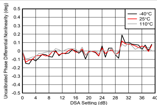
FIG 4-197. TX DSA Uncalibrated Phase Differential Nonlinearity at 8.1GHz
