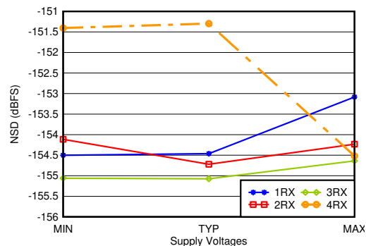
FIG 4-420. RX IMD3 vs Supply and Channel at 4.9GHz
