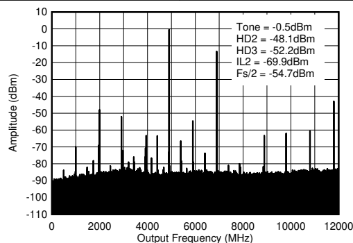
図 4-181. TX Single Tone (-12 dBFS) Output Spectrum at 4.9GHz ( 0-f_{\text{DAC}} )
