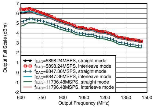
図 4-1. TX Output Fullscale vs Output Frequency
