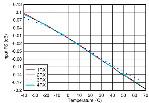
FIG 4-286. RX Input Fullscale vs Temperature and Channel at 800MHz
