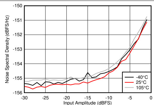
図 4-351. RX Noise Spectral Density vs Input Amplitude and Temperature at 2.6GHz
