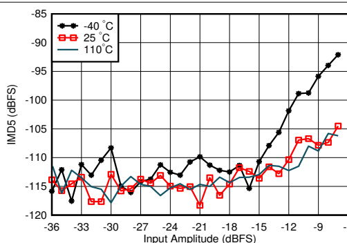
FIG 4-304. RX IMD5 vs Input Level and Temperature at 0.8GHz
