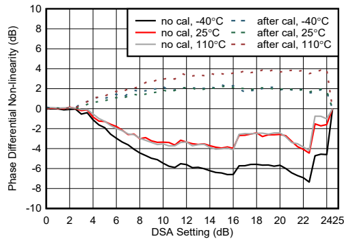
FIG 4-428. RX Phase Differential Nonlinearity at 8.1GHz
