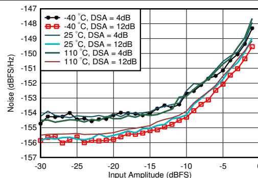
図 4-298. RX Noise Spectral Density vs Input Amplitude and Temperature at 0.8GHz
