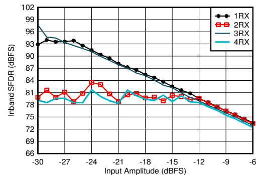
FIG 4-418. RX In-Band SFDR ( \pm 400 MHz) vs Input Amplitude and Channel at 4.9GHz
