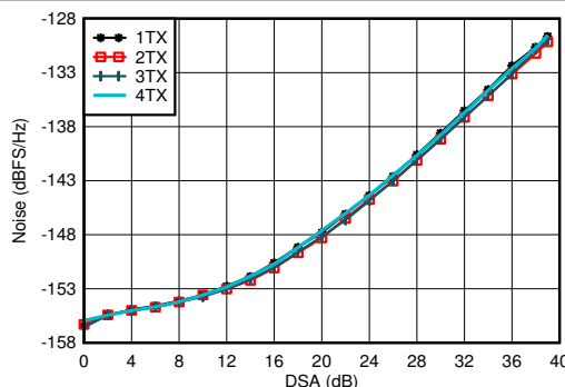
FIG 4-168. TX Output Noise vs Channel and Attenuation at 2.6GHz
