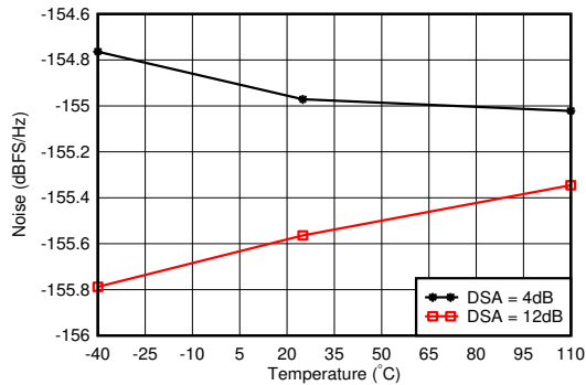
FIG 4-328. RX Noise Spectral Density vs Temperature at 1.75GHz
