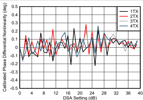
FIG 4-196. TX DSA Calibrated Phase Differential Nonlinearity at 8.1GHz
