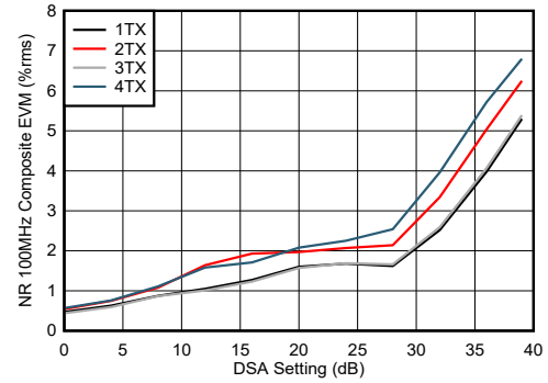
4-282. TX NR100MHz EVM vs DSA Setting at 9.6GHz
