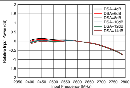
図 4-346. RX Inband Gain Flatness, f_{\text{IN}} = 2600\text{MHz}
