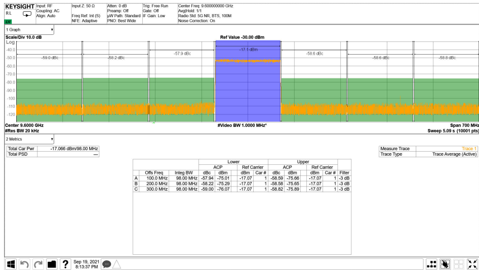
4-281. TX NR100MHz ACPR vs DSA Setting at 9.6GHz NR100MHz alt-ACPR vs DSA Setting at 9.6GHz
