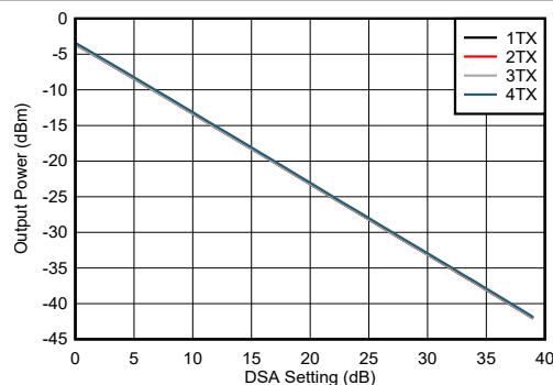
FIG 4-185. TX Output Power vs DSA Setting at 8.1GHz
