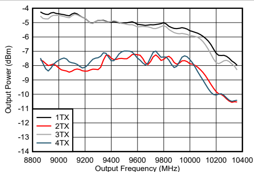
FIG 4-233. TX Output Power vs Frequency at 9.61GHz
