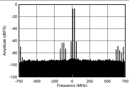
FIG 4-469. RX Single Tone Output FFT at 9.61GHz
