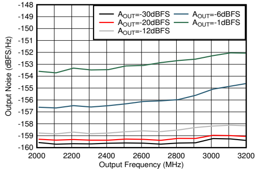
FIG 4-102. TX Single Tone Output Noise vs Frequency and Amplitude at 2.6GHz
