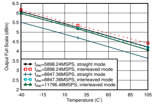
図 4-2. TX Output Fullscale vs Temperature
