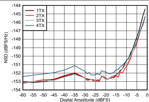
Figure 4-260. TX NSD vs Digital Amplitude at 9.61GHz
