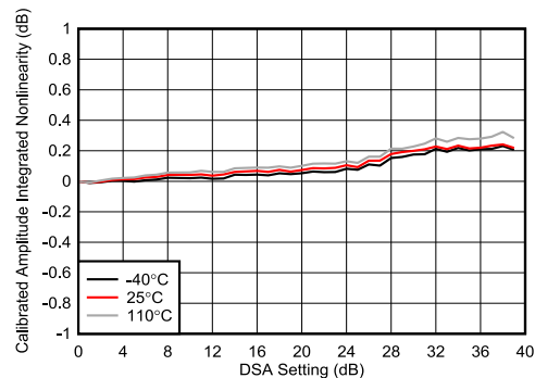
4-194. TX DSA Calibrated Amplitude Integrated Nonlinearity at 8.1GHz
