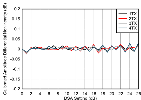
FIG 4-237. TX DSA Calibrated Amplitude Differential Nonlinearity
