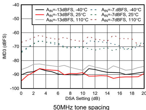
図 4-457. RX IMD3 vs DSA Setting at 9.6GHz
