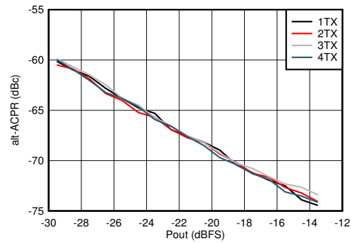
FIG 4-105. TX 20-MHz LTE alt-ACPR vs Digital Level at 2.6GHz
