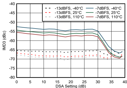
図 4-220. TX IMD3 vs DSA Setting at 8.11GHz
