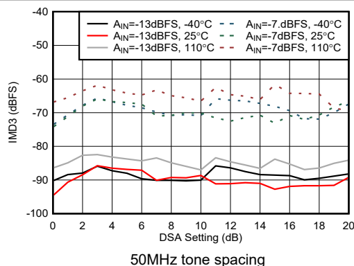
図 4-456. RX IMD3 vs DSA Setting at 9.6GHz
