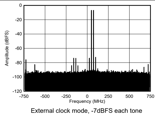
図 4-445. RX Dual Tone Output FFT at 8.1GHz
