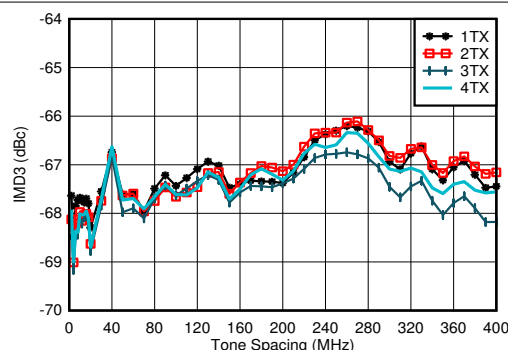
FIG 4-170. TX IMD3 vs Tone Spacing and Channel at 4.9GHz
