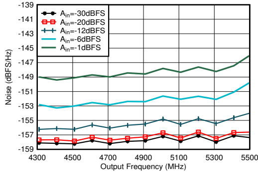
4-173. TX Single Tone Output Noise vs Frequency and Amplitude at 4.9GHz
