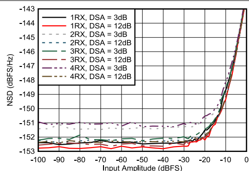
図 4-460. RX NSD vs Digital Amplitude at 9.6GHz
