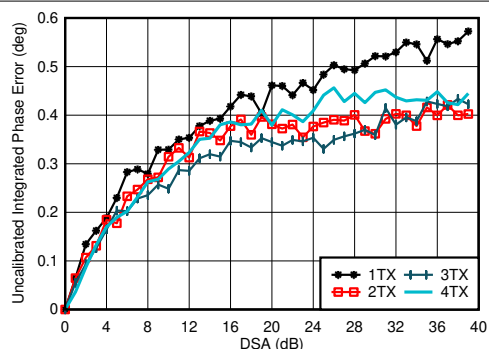
図 4-126. TX Uncalibrated Integrated Phase Error vs DSA Setting and Channel at 3.5GHz
