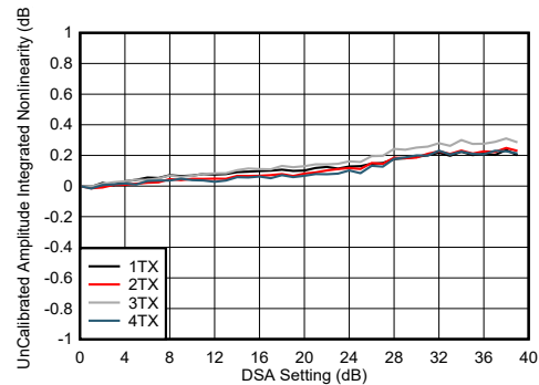
4-191. TX DSA Uncalibrated Amplitude Integrated Nonlinearity at 8.1GHz
