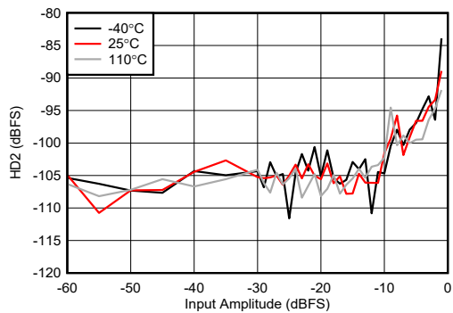
FIG 4-436. RX HD2 vs Digital Amplitude at 8.1GHz
