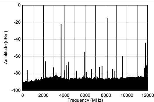
FIG 4-205. TX Single Tone Output Spectrum at 8.1GHz
