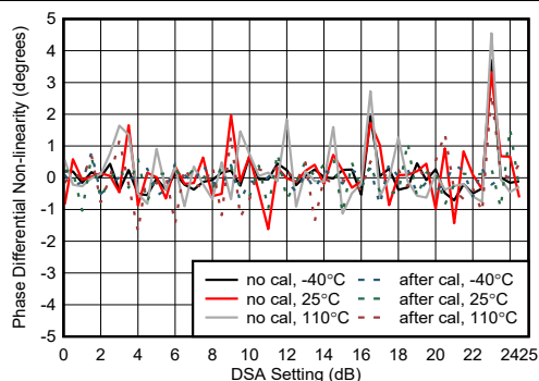
Figure 4-453. RX Phase Differential Non-linearity at 9.6GHz
