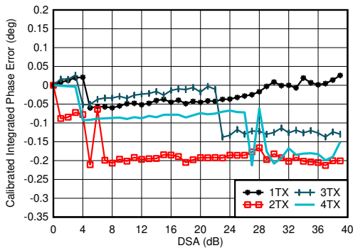
図 4-13. TX Calibrated Differential Phase Error vs DSA Setting and Channel at 0.85GHz
