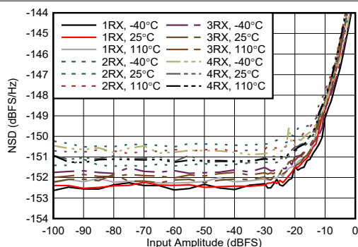
図 4-459. RX NSD vs Digital Amplitude at 9.6GHz
