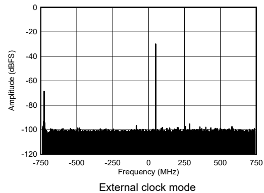
図 4-443. RX Single Tone Output FFT at 8.1GHz, -30 dBFS
