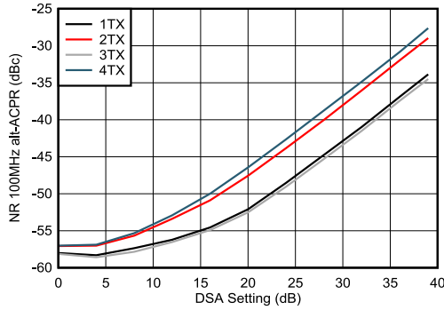
4-281. TX NR100MHz ACPR vs DSA Setting at 9.6GHz NR100MHz alt-ACPR vs DSA Setting at 9.6GHz
