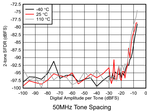
図 4-440. RX 2-tone SFDR vs Digital Amplitude at 8.1GHz
