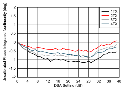
FIG 4-199. TX DSA Uncalibrated Phase Integrated Nonlinearity at 8.1GHz
