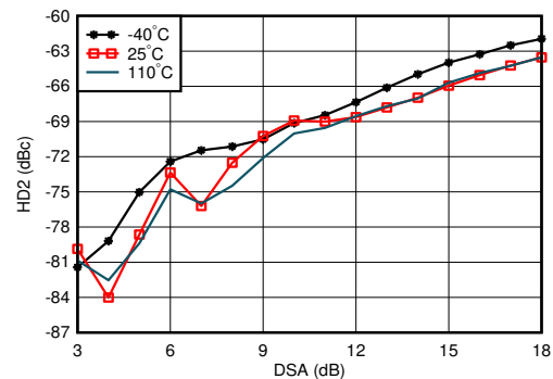
FIG 4-306. RX HD2 vs DSA Setting and Temperature at 0.8GHz
