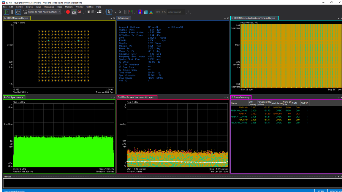
4-230. TX 100MHz NR EVM at 8.1GHz
