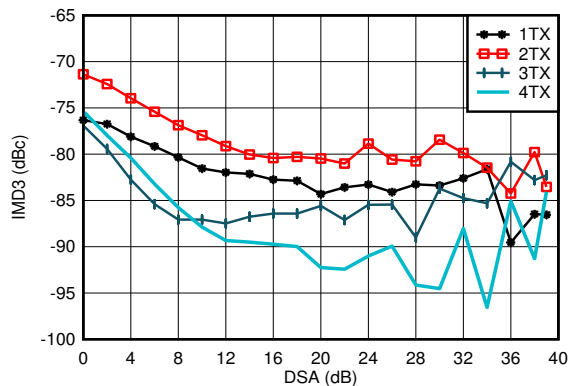
図 4-21. TX IMD3 vs DSA Setting at 0.85GHz
