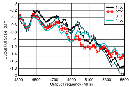
図 4-150. TX Full Scale vs RF Frequency and Channel at 5898.24 MSPS, Straight Mode, 2nd Nyquist Zone
