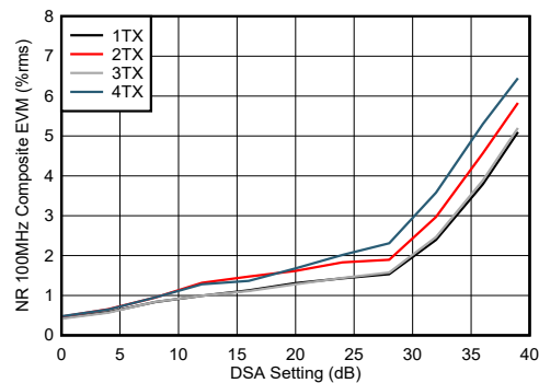
FIG 4-228. TX NR100MHz EVM vs DSA Setting 8.1GHz
