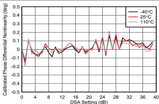
FIG 4-198. TX DSA Calibrated Phase Differential Nonlinearity at 8.1GHz
