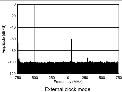
図 4-444. RX Single Tone Output FFT at 8.1GHz, -60 dBFS
