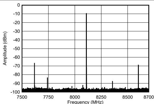
FIG 4-204. TX Single Tone Output Spectrum at 8.1GHz
