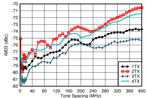
図 4-22. TX IMD3 vs Tone Spacing and Channel at 0.85GHz
