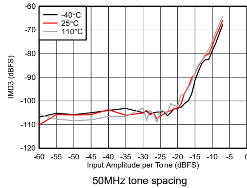
FIG 4-429. RX IMD3 vs Input Amplitude at 8.1GHz
