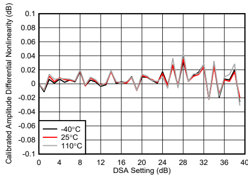
4-190. TX DSA Calibrated Amplitude Differential Nonlinearity at 8.1GHz
