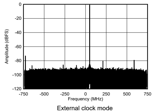
図 4-441. RX Single Tone Output FFT at 8.1GHz, -1dBFS
