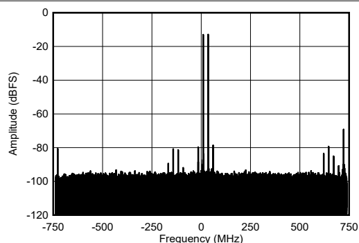
FIG 4-470. RX Single Tone Output FFT at 9.61GHz
