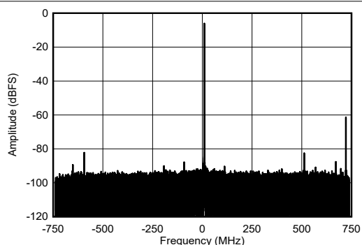
FIG 4-467. RX Single Tone Output FFT at 9.61GHz
