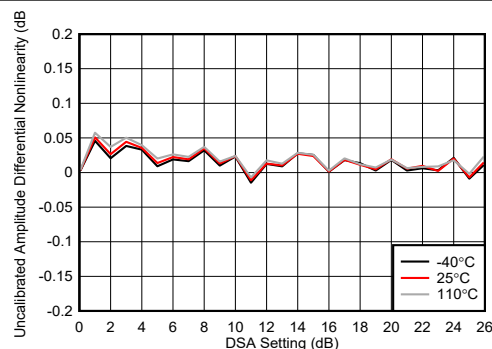
FIG 4-238. TX DSA Uncalibrated Amplitude Differential Nonlinearity
