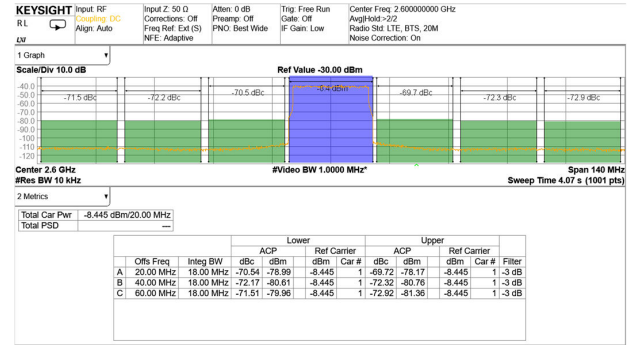
FIG 4-103. TX 20-MHz LTE Output Spectrum at 2.6GHz (Band 41)
