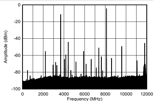
FIG 4-203. TX Single Tone Output Spectrum at 8.1GHz
