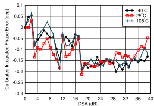
图 4-133. TX Calibrated Differential Phase Error vs DSA Setting and Temperature at 3.5GHz
