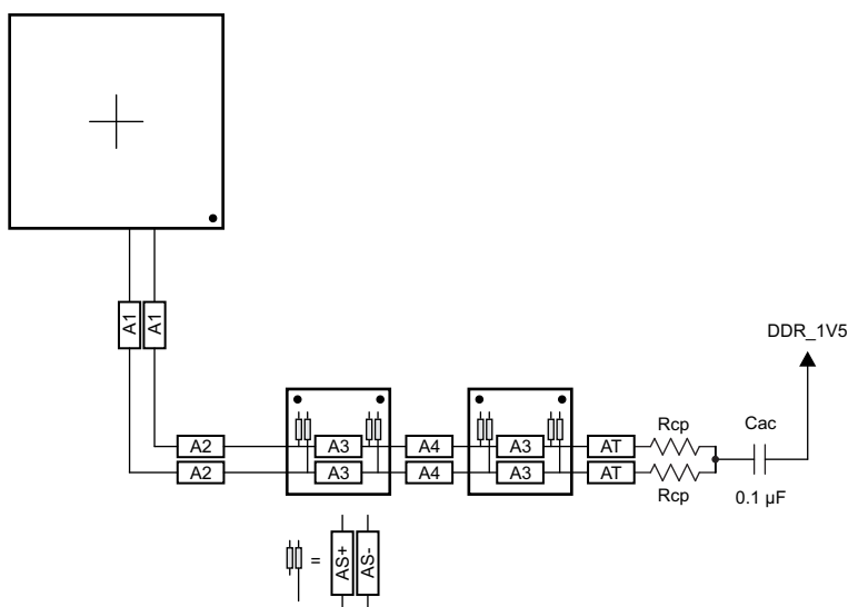
8-10. CK Routing for Four Mirrored DDR3 Devices
