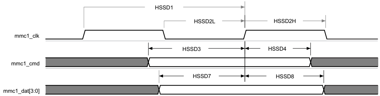
图 7-62. MMC/SD/SDIO in - High Speed - Receiver Mode
