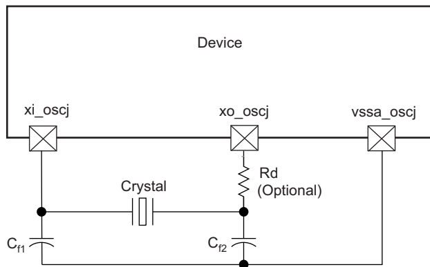
8-33. Grounding Scheme for High-Frequency Clock
