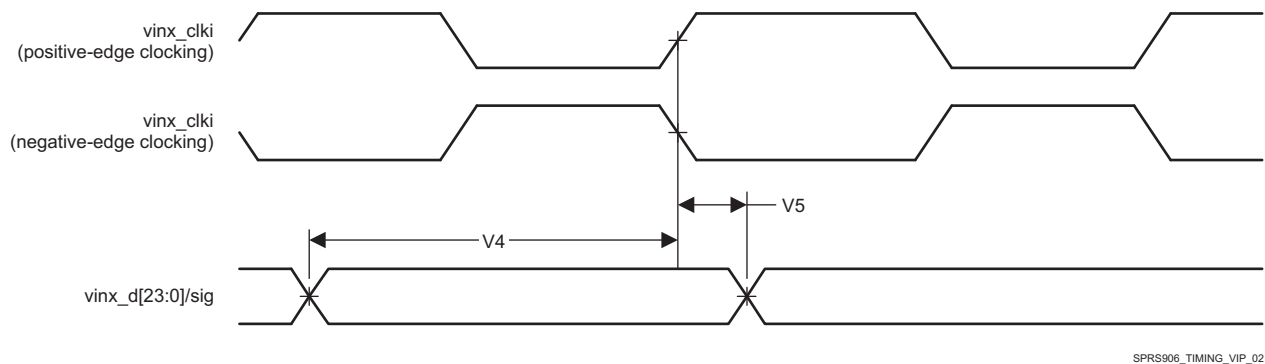
図 7-5. Video Input Ports timings
