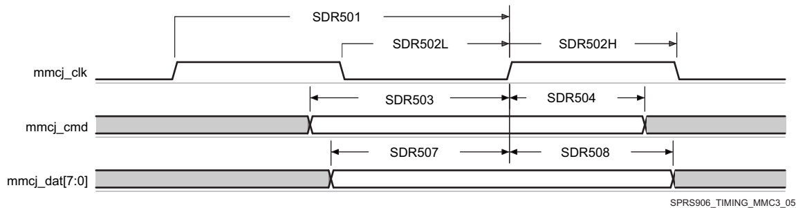
图 7-89. MMC/SD/SDIOj in - High Speed SDR50 - Receiver Mode
