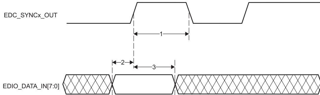
図 7-101. PRU-ICSS ECAT Input Validated With SYNCx Timing
