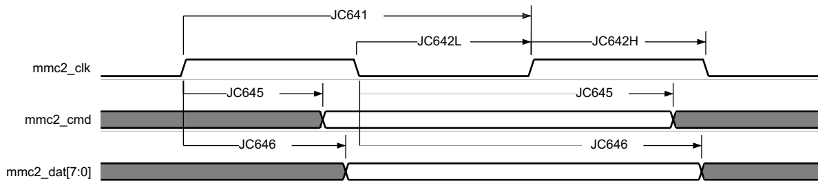
図 7-77. MMC/SD/SDIO in - High Speed JC64 - Transmitter Mode
