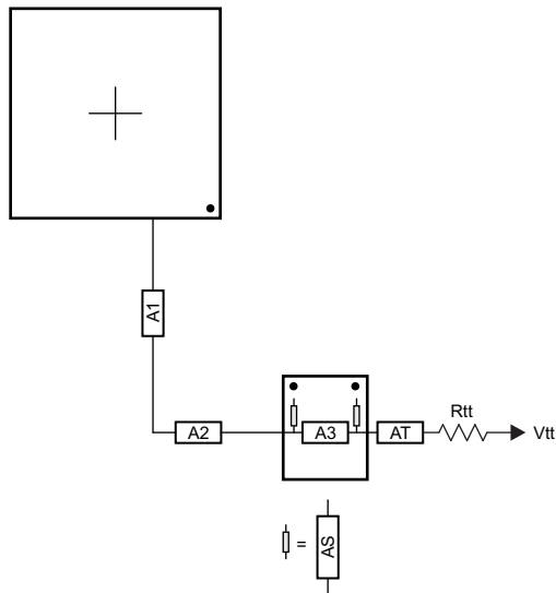
8-17. ADDR_CTRL Routing for Two Mirrored DDR3 Devices
