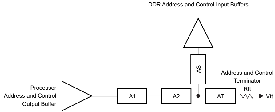
FIG 8-19. ADDR_CTRL Topology for One DDR3 Device
