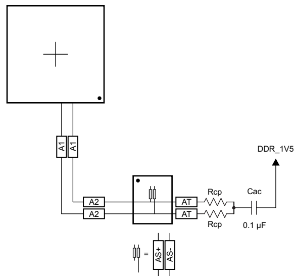
FIG 8-20. CK Routing for One DDR3 Device
