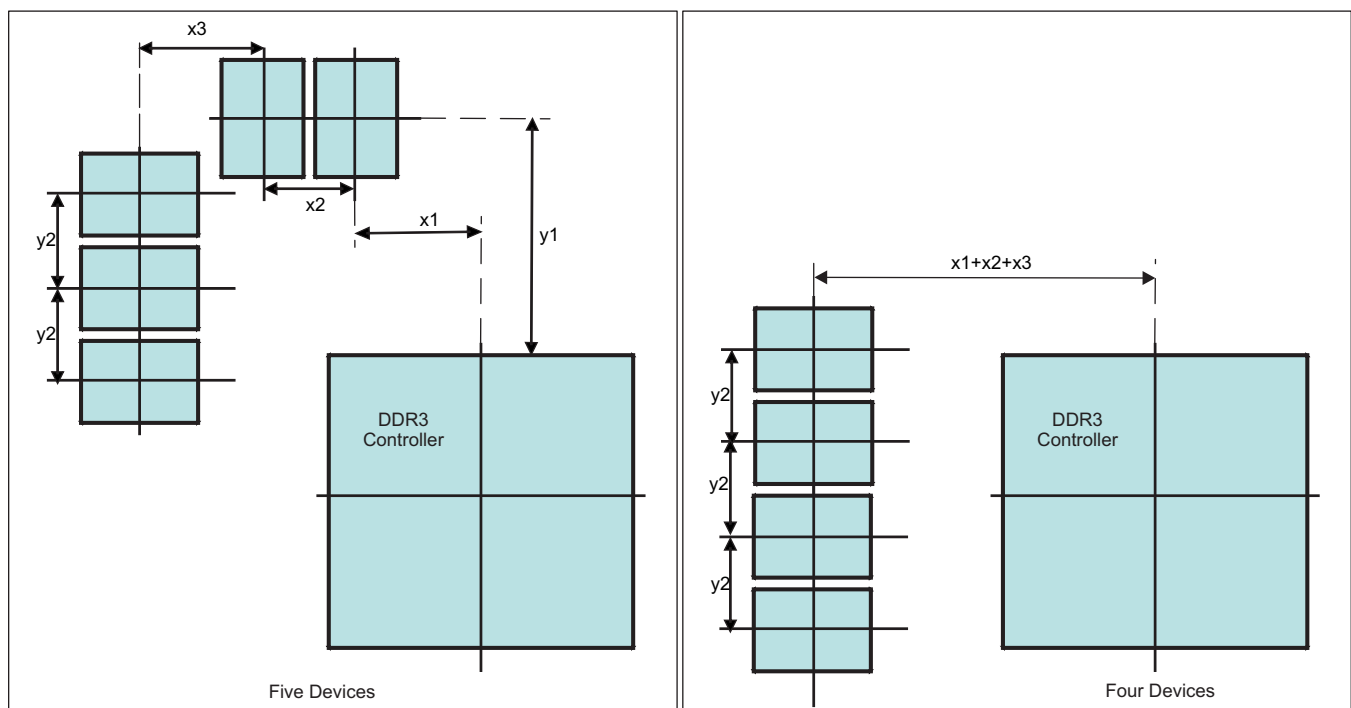
図 8-4. Placement Specifications
