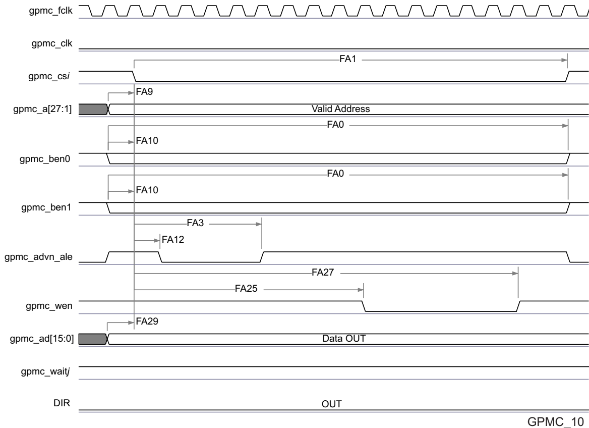
7-16. GPMC / NOR Flash - Asynchronous Write - Single Word (1)
