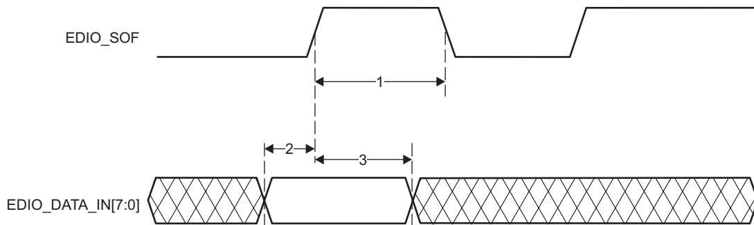
図 7-102. PRU-ICSS ECAT Input Validated With SOF
