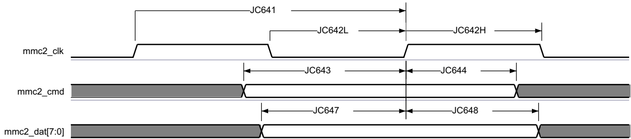
図 7-76. MMC/SD/SDIO in - High Speed JC64 - Receiver Mode
