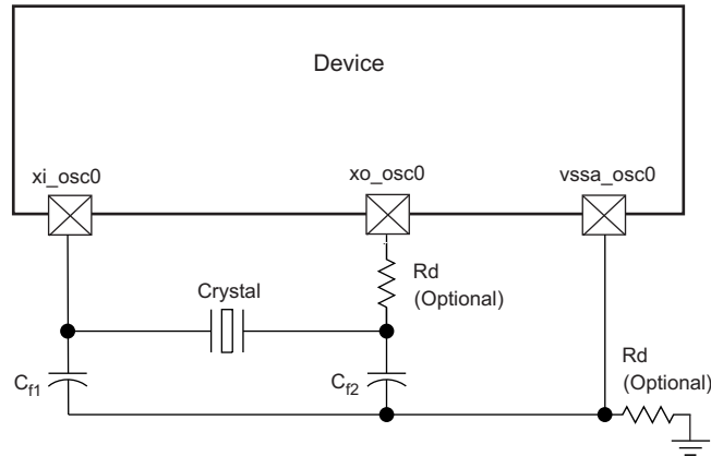
6-2. Crystal Implementation
