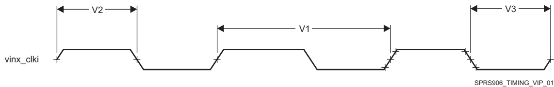
図 7-4. Video Input Ports clock signal
