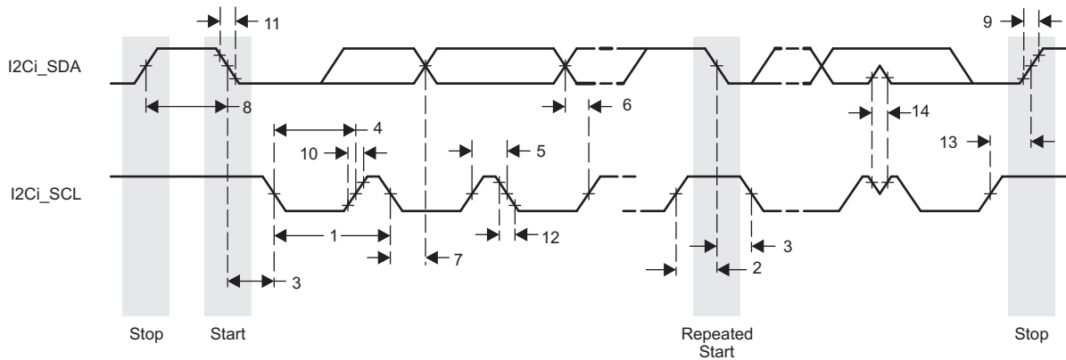
图 7-23. I2C Receive Timing
