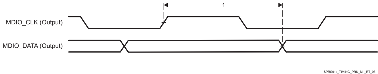
图 7-106. PRU-ICSS MDIO_DATA Timing - Output Mode
