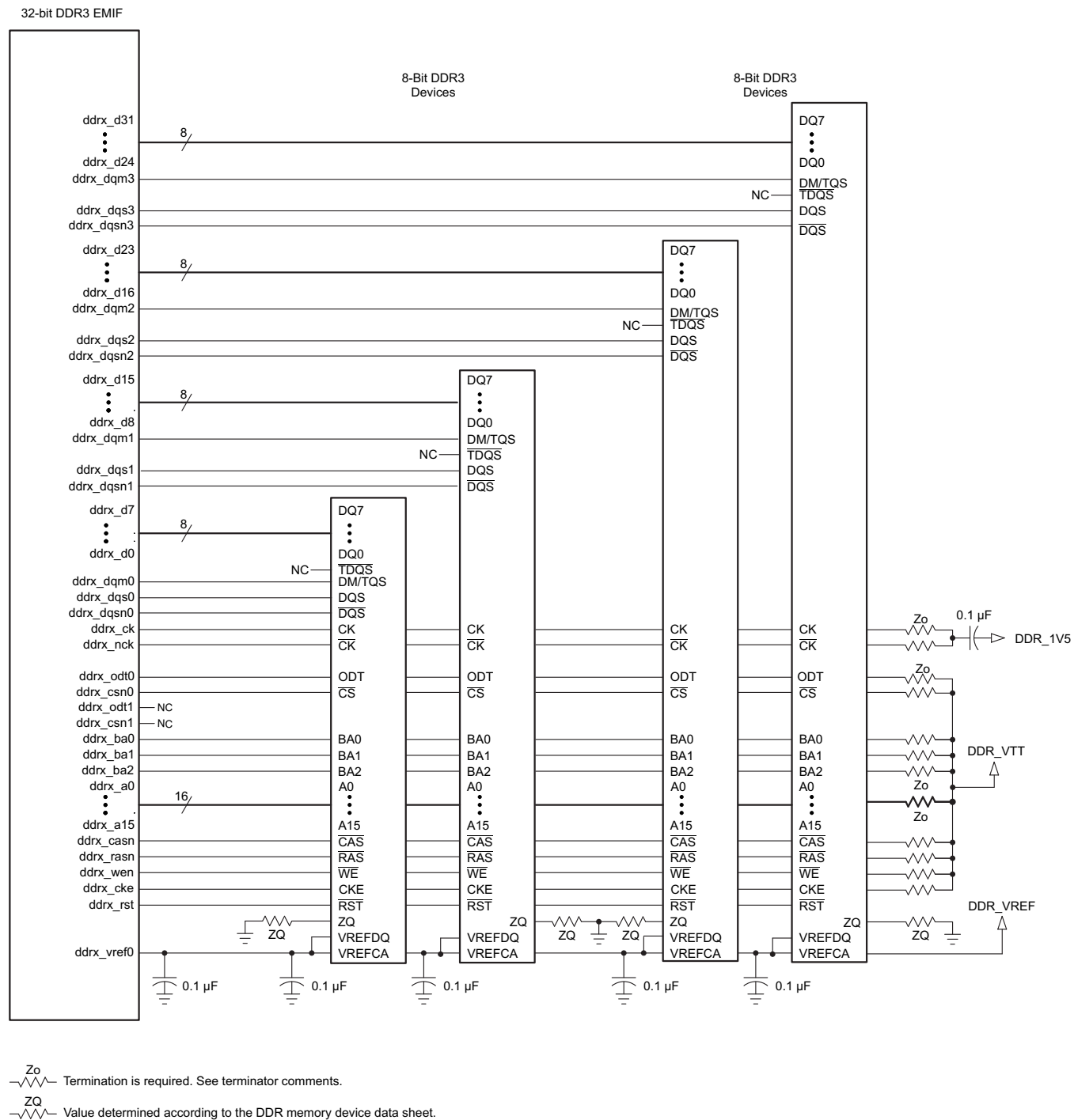
8-3. 32-Bit, One-Bank DDR3 Interface Schematic Using Four 8-Bit DDR3 Devices
