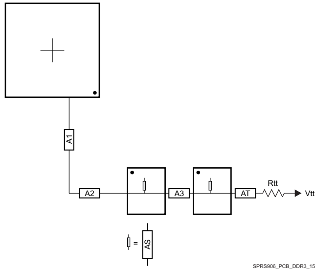
FIG 8-15. ADDR_CTRL Routing for Two Single-Side DDR3 Devices
