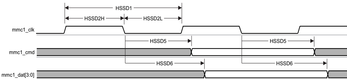
图 7-63. MMC/SD/SDIO in - High Speed - Transmitter Mode
