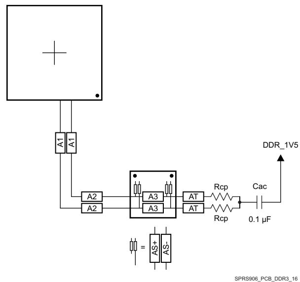
FIG 8-16. CK Routing for Two Mirrored DDR3 Devices
