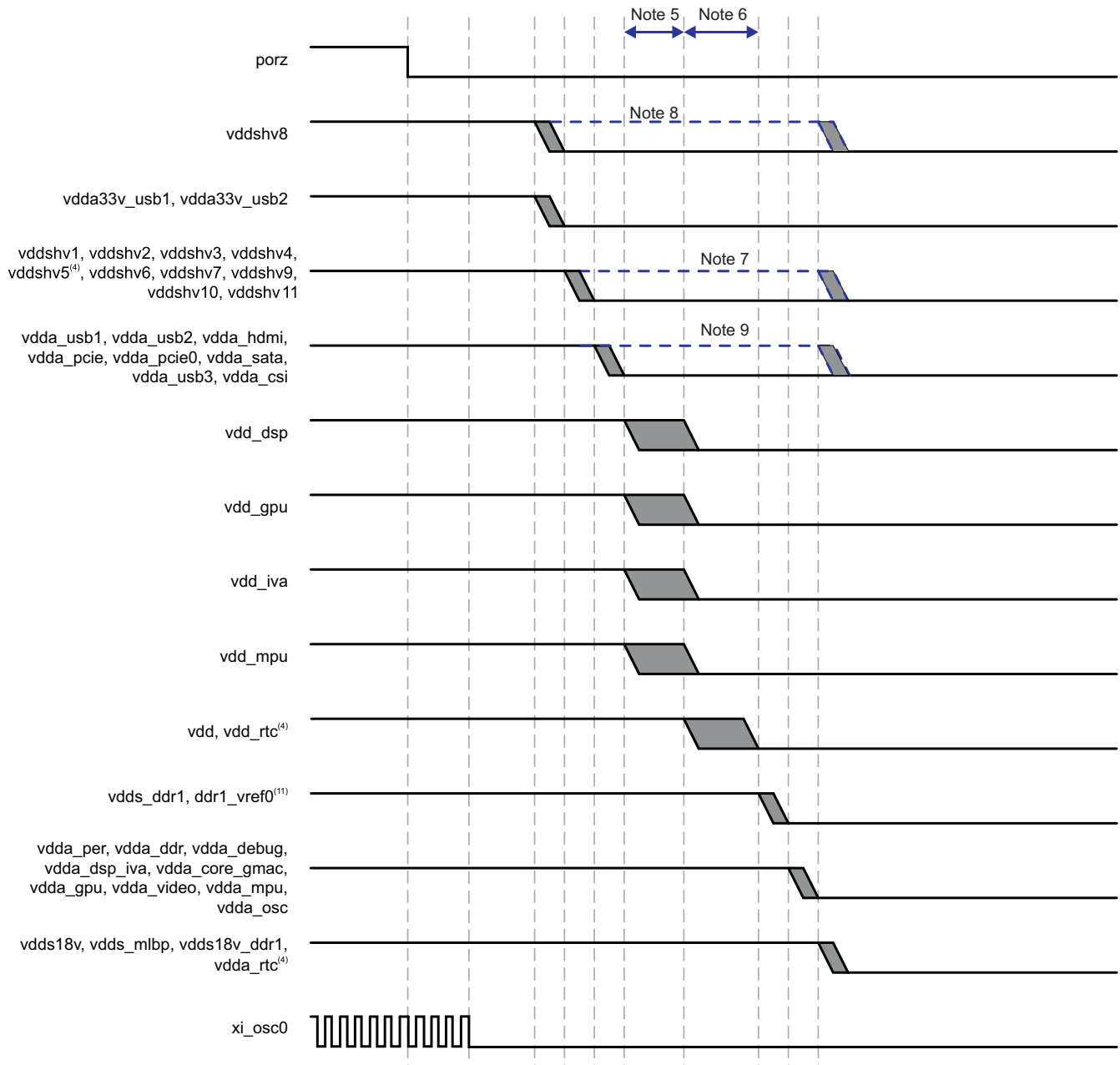
图 5-3. Power-Down Sequencing (10)(12)
