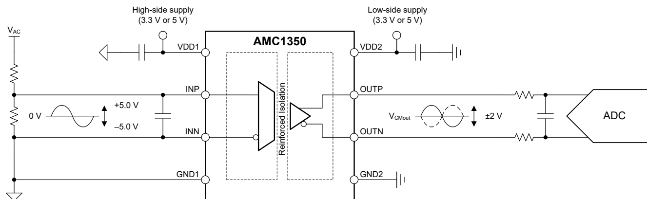
Typical Application
