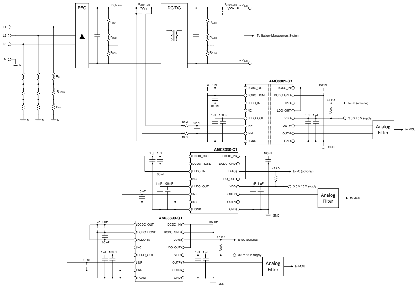
7-1. The AMC3330-Q1 in an OBC Application
