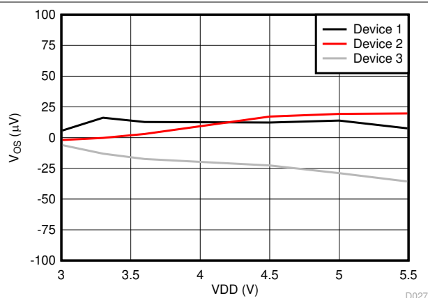
図 5-18. Offset Error vs Supply Voltage
