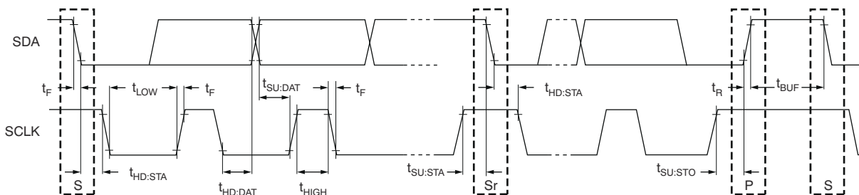
7-1. Timing Specification
