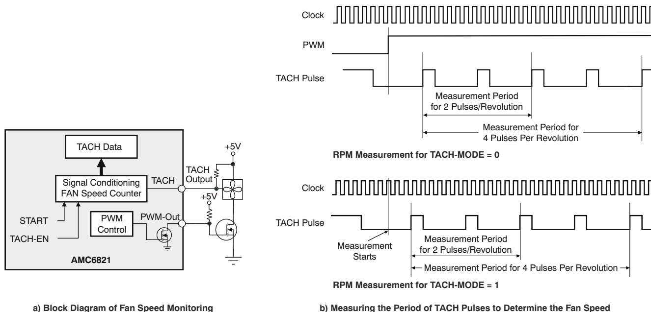
Figure 8-7. Fan Speed Measurement
