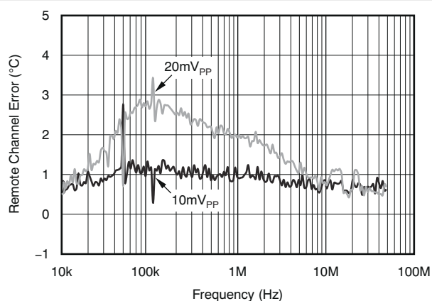
FIG 7-8. Temperature Error vs Differential Mode Noise Frequency
