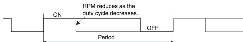
FIG 8-6. PWM Waveform (PWMinv = 1)
