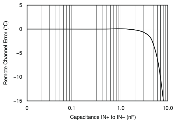
FIG 7-9. Temperature Error vs Capacitance Between In+ and In-
