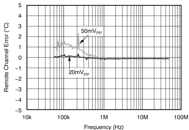
7-5. Temperature Error vs Common-Mode Noise Frequency
