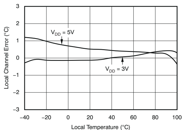
7-3. Local Channel Error From Calibrated Bath
