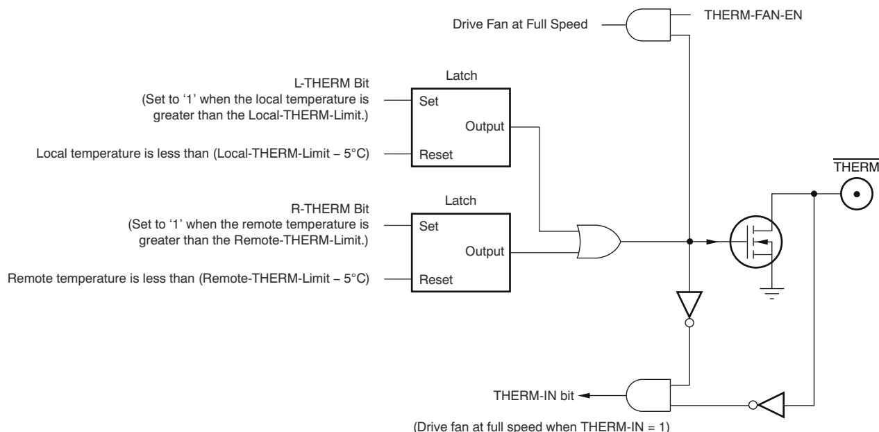
8-12. Structure of the \overline{\text{THERM}} Pin
