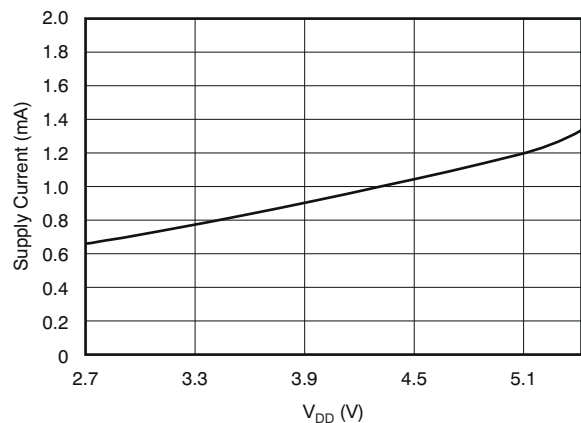
FIG 7-6. Supply Current vs V DD
