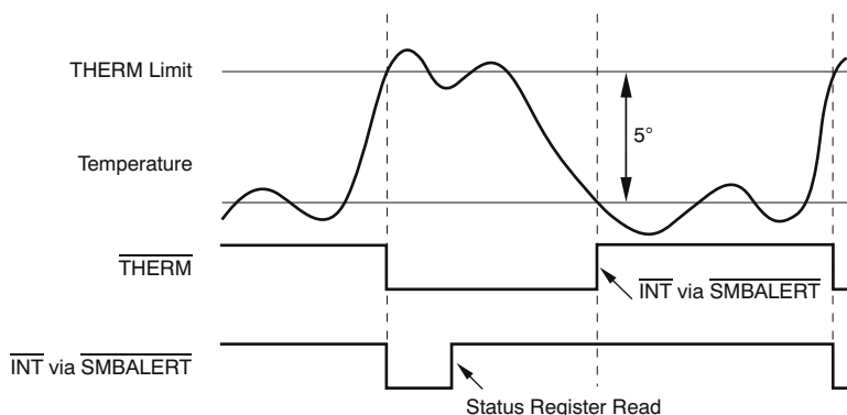
8-13. Operation of the Therm Interrupt and the \overline{\text{THERM}} Pin
