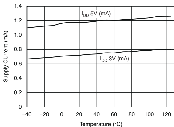
FIG 7-7. Supply Current vs Temperature
