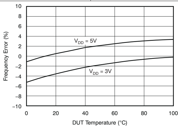
FIG 7-10. PWM Frequency Error vs Temperature
