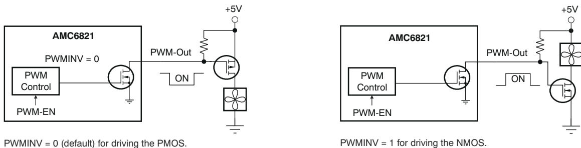
FIG 8-5. PWM Output
