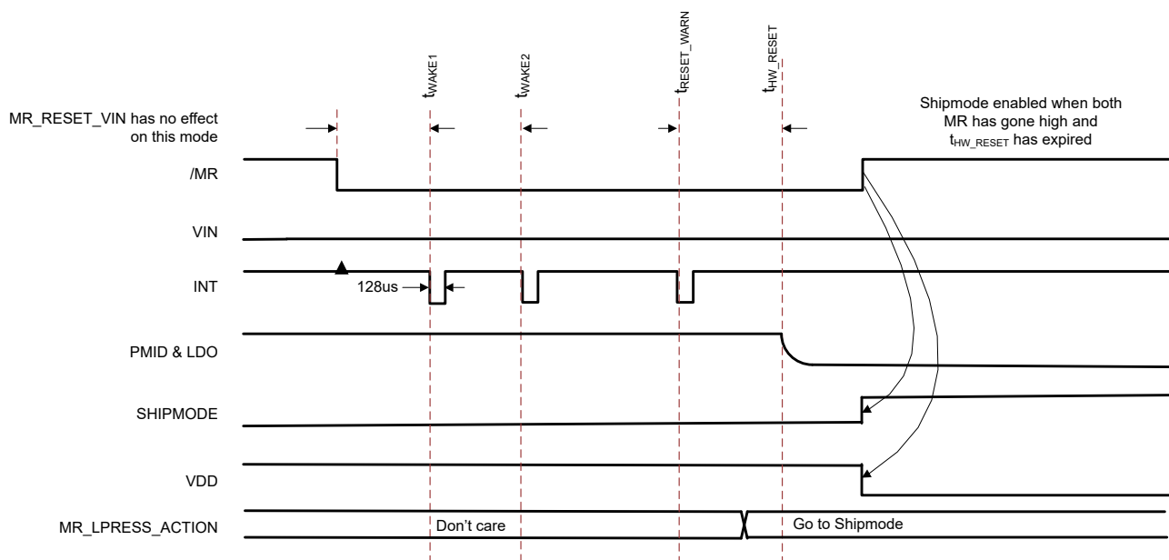
FIG 9-6. MR Wake and Reset Timing Active Mode When MR_LPRESS_ACTION = 1x (Ship Mode) and Only BAT is Present
