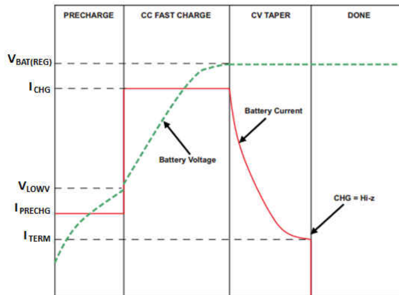
図 9-2. BQ21062 Typical Charge Cycle
