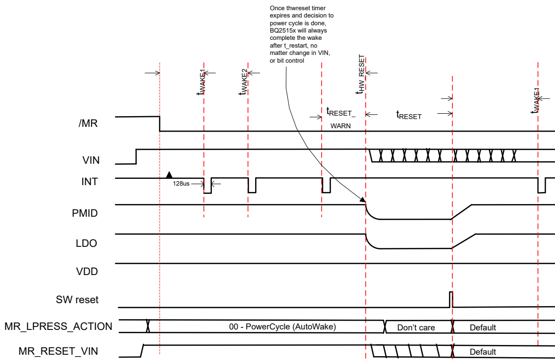
FIG 9-5. MR Wake and Reset Timing with VIN Present or BAT Active Mode When MR_LPRESS_ACTION = 00
