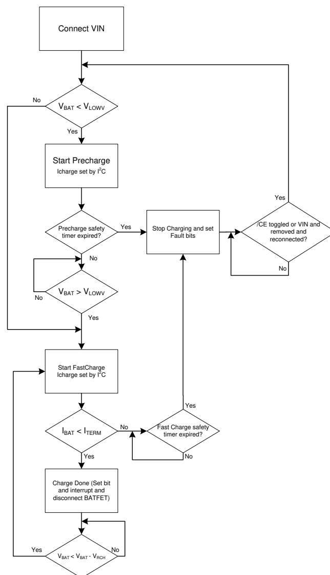
FIG 9-1. BQ21062 Charger Flow Diagram
