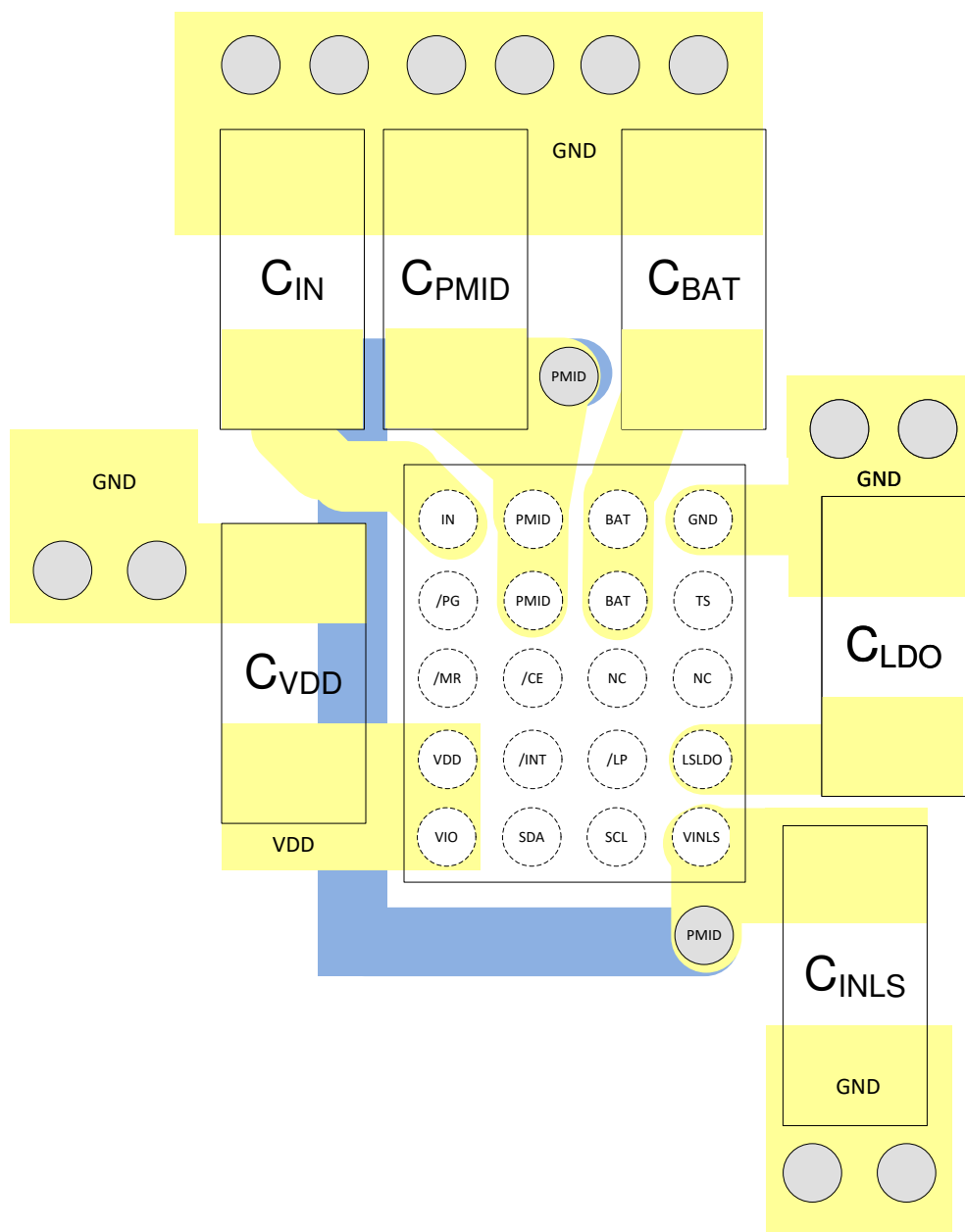
12-1. Layout Example
