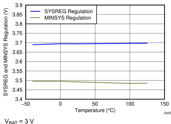
FIG 7-3. SYSREG and MINSYS Regulation vs Temperature
