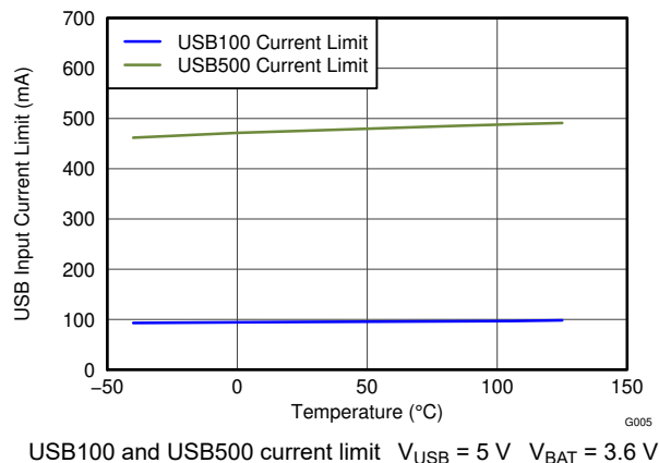
FIG 7-5. USB Input Current Limit vs Temperature
