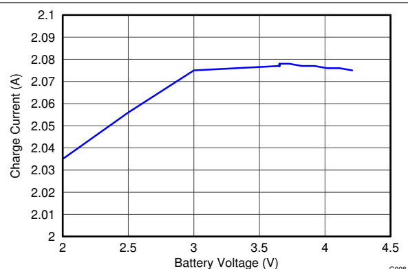
FIG 7-8. Charge Current vs Battery Voltage
