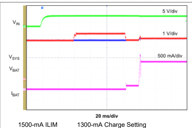
☒ 9-4. IN Plug-in with Battery Connected
