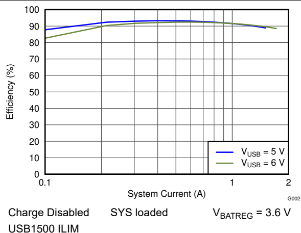
FIG 7-2. USB Efficiency
