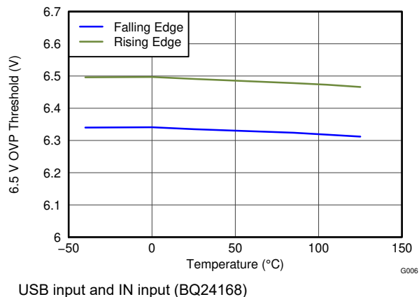
FIG 7-6. 6.5-V OVP Threshold vs Temperature
