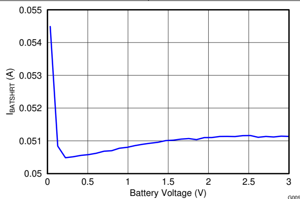
FIG 7-9. I_{\text{BATSHRT}} vs Battery Voltage
