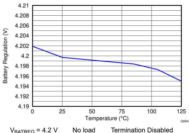
FIG 7-4. Battery Regulation vs Temperature
