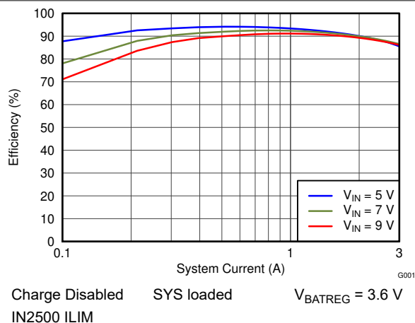
FIG 7-1. IN Efficiency
