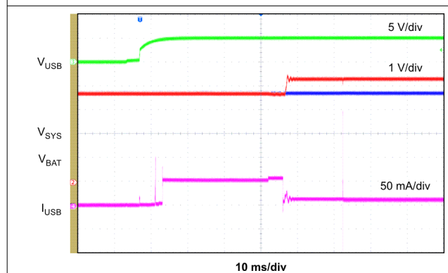
☒ 9-5. Adapter Detection USB
