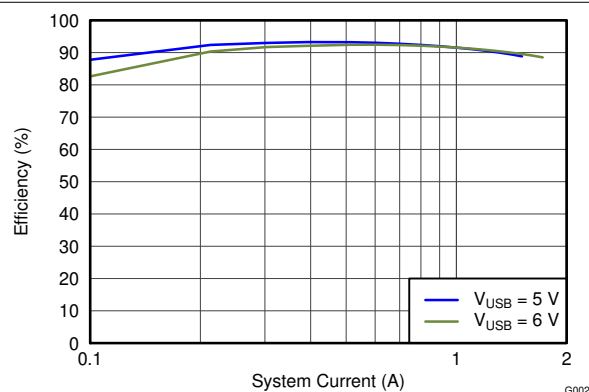
9-12. USB Efficiency
