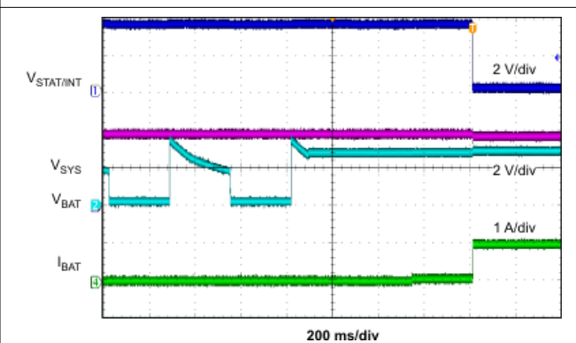
☒ 9-4. IN Plug-in with Battery Connected
