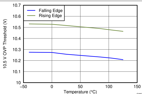
FIG 7-7. 10.5-V OVP Threshold vs Temperature
