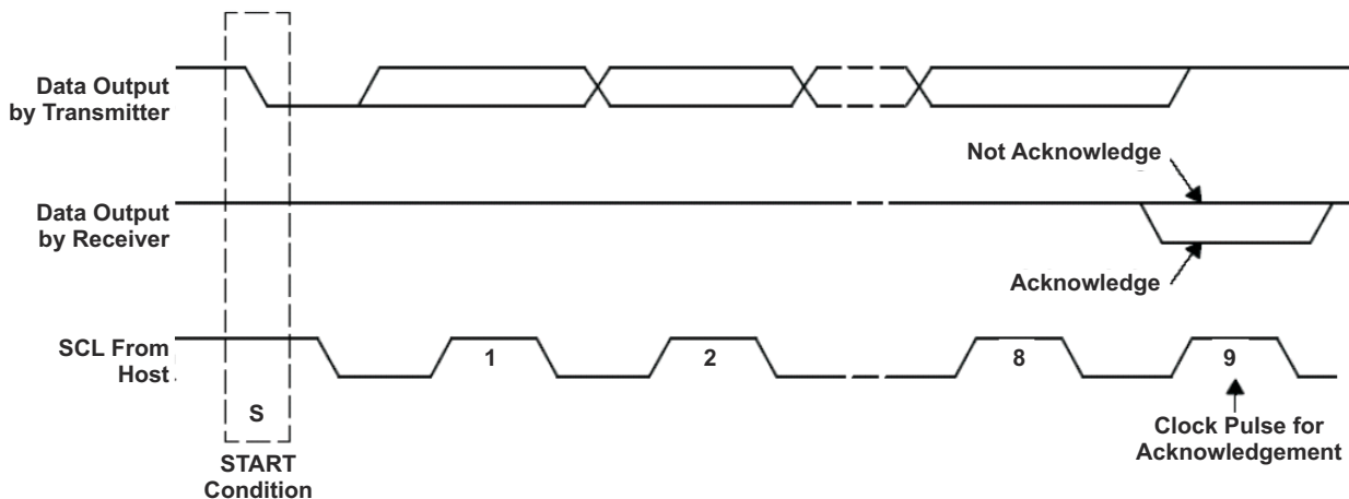
❏ 8-10. Acknowledge on the I 2 C Bus
