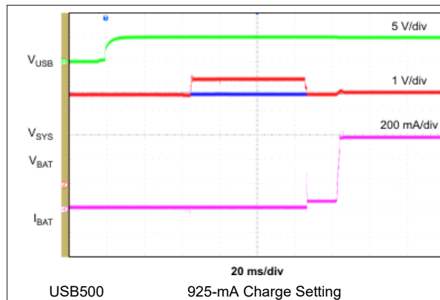
☒ 9-3. USB Plug-In with Battery Connected
