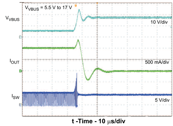
Figure 19. OVP Response
