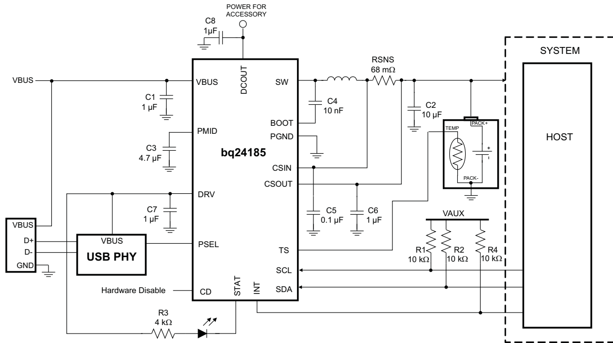
Figure 3. I²C Controlled 1-Cell USB Charger Application Circuit
