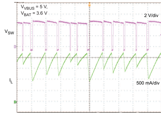
t -Time - 2 \mu s/div Figure 9. Cycle by Cycle Current Limit
