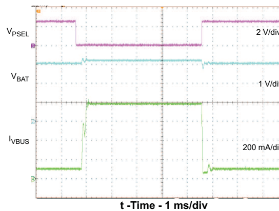
Figure 15. PSEL Transition
