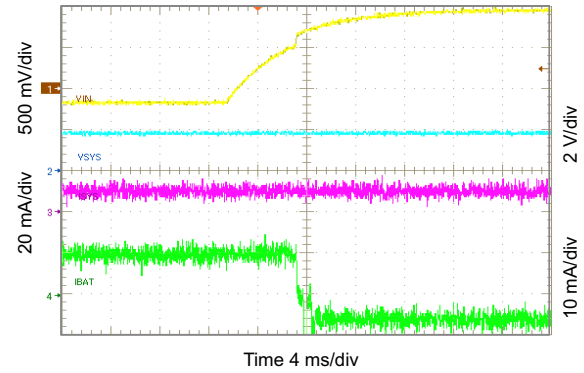
Figure 10-9. OVP Fault
