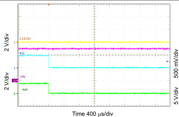
FIG 10-61. \overline{PG} Functions as Shifted \overline{MR} Output
