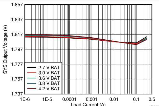
10-17. 1.8 V sys Load Regulation
