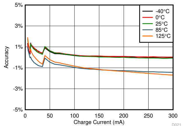
FIG 8-10. Charge Current Accuracy vs Charge Current
