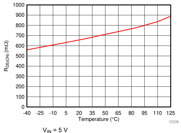
FIG 8-12. R_{DS(ON)} of High Side MOSFET vs Temperature
