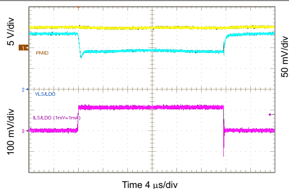
10-54. 1.8 V_{LSLDO} Load Transient, 0 to 100 mA
