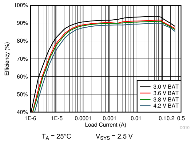
10-13. 2.5 V_{\text{SYS}} System Efficiency
