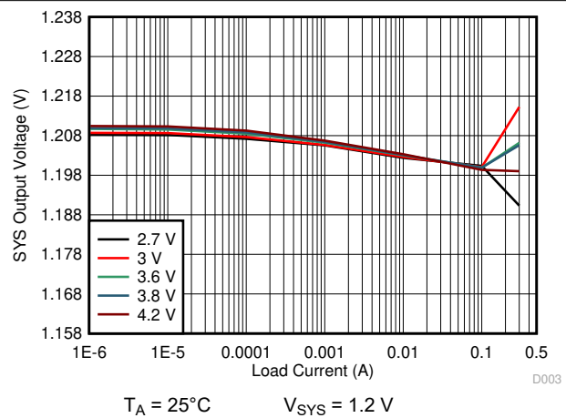
10-15. 1.2 V_{\text{SYS}} Load Regulation
