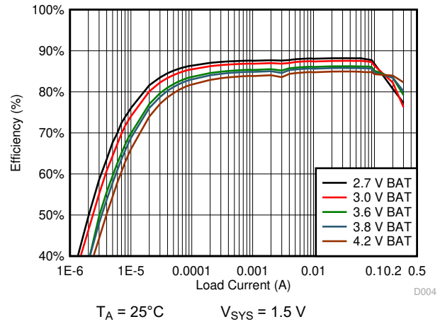
10-11. 1.5 V_{\text{SYS}} System Efficiency
