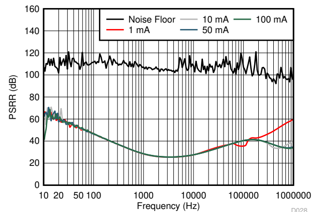
FIG 8-14. LS/LDO PSRR vs Frequency
