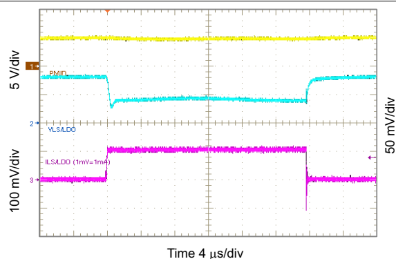
10-52. 0.8 V_{LSLDO} Load Transient, 0 to 100 mA
