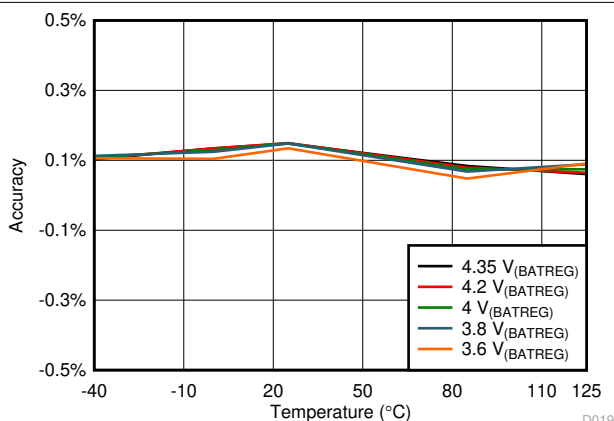
Figure 8-8. V_{BAT(REG)} Accuracy vs Temperature
