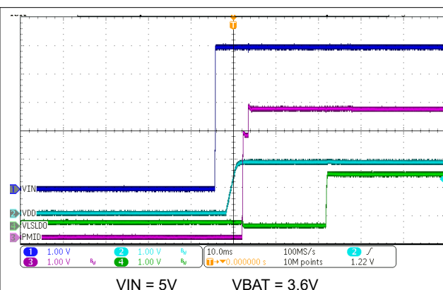
FIG 10-3. Power Up from Ship Mode with IN Supply Insertion
