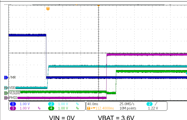
FIG 10-5. Power Up from Ship Mode with \overline{\text{MR}} Press
