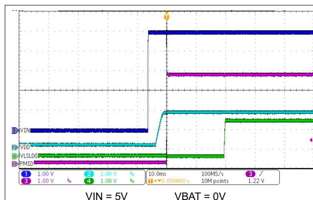
FIG 10-2. Power Up from IN Supply Insertion with No Battery
