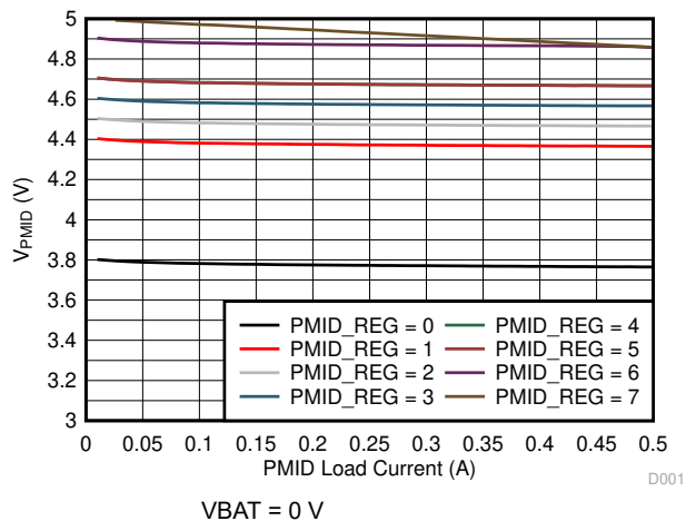
8-13. PMID Load Regulation
