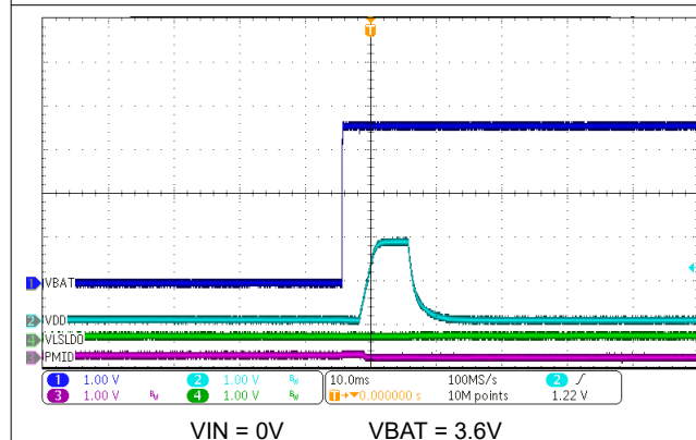
FIG 10-4. Wake In To Ship Mode on Battery Insertion with No IN Supply
