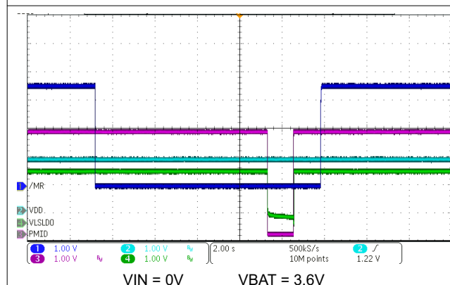
FIG 10-6. HW Reset on \overline{\text{MR}} Long Button Press
