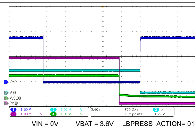
FIG 10-7. Ship Mode Entry with \overline{\text{MR}} Long Button Press
