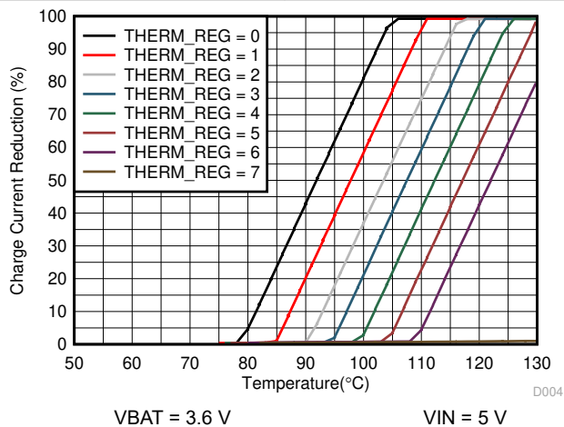
8-15. Charge Current Thermal Regulation
