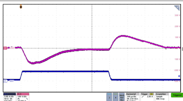
図 7-15. Forward Mode 28-V Transient Reponse with 20 Vin
