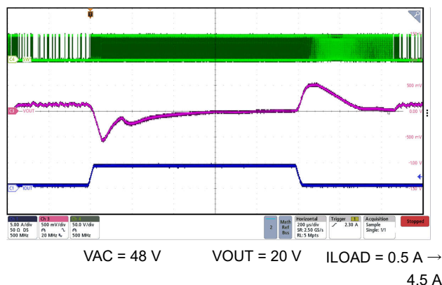
図 7-14. Forward Mode 20-V Transient Reponse with 48 Vin
