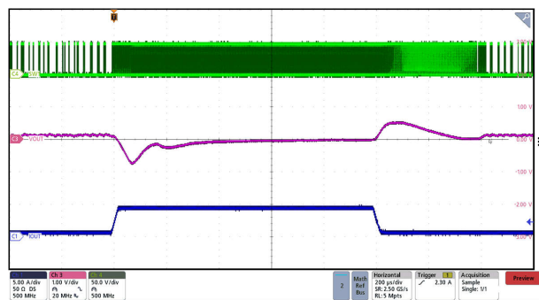
図 7-16. Forward Mode 28-V Transient Reponse with 48 Vin
