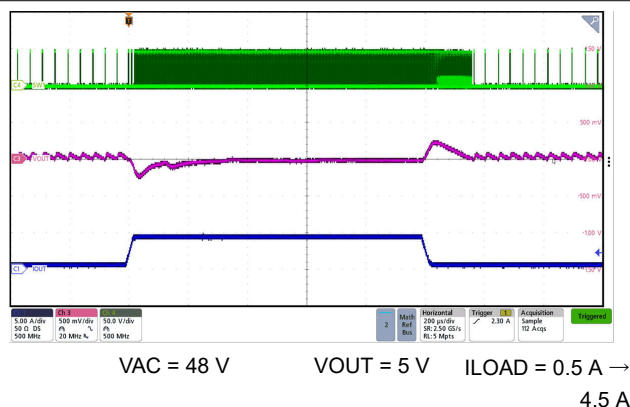
図 7-12. Forward Mode 5-V Transient Reponse with 48 Vin
