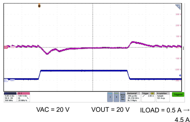
図 7-13. Forward Mode 20-V Transient Reponse with 20 Vin
