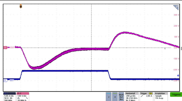
図 7-17. Forward Mode 36-V Transient Reponse with 20 Vin
