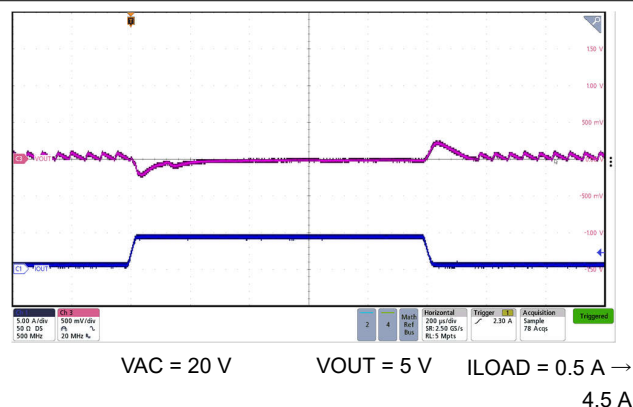
図 7-11. Forward Mode 5-V Transient Reponse with 20 Vin
