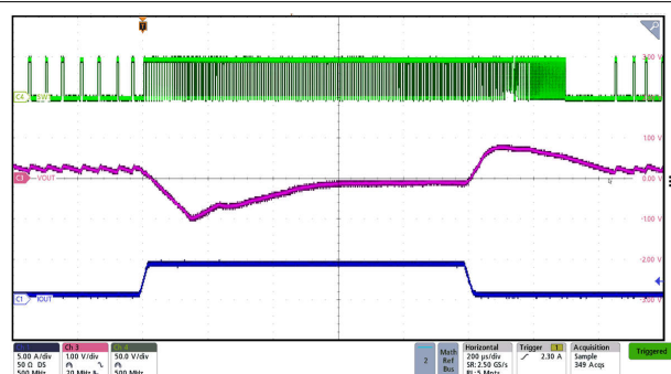
図 7-18. Forward Mode 36-V Transient Reponse with 48 Vin
