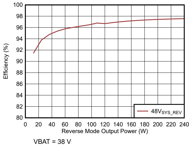
6-11. Reverse Mode Efficiency (10s battery configuration)
