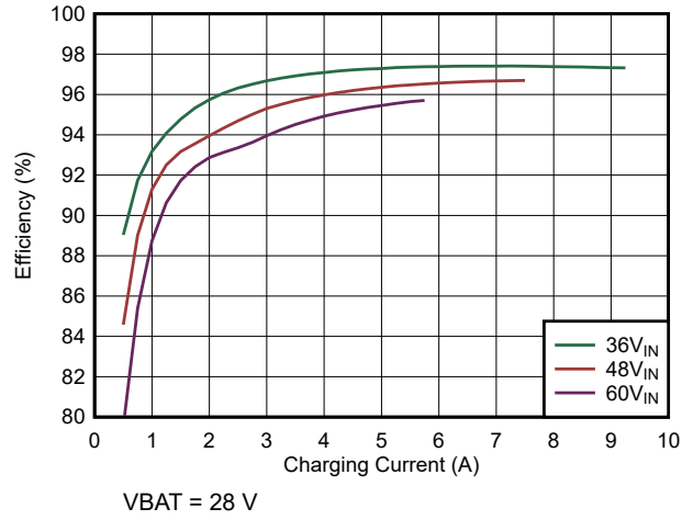
6-2. Charge Efficiency vs Charge Current (7s battery configuration)
