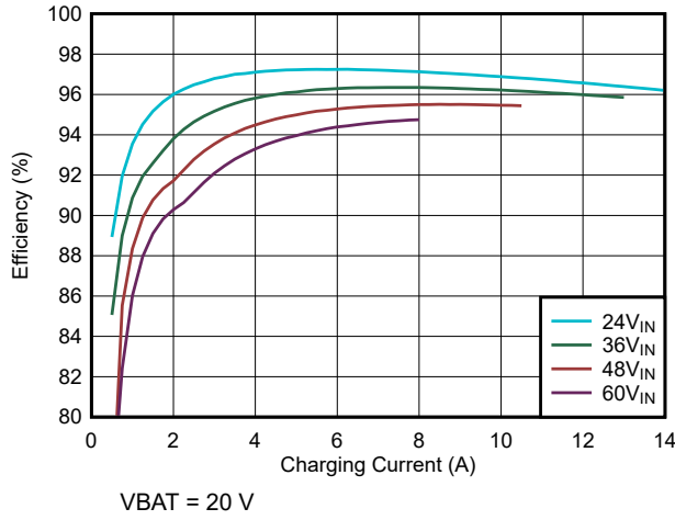
6-1. Charge Efficiency vs Charge Current (5s battery configuration)
