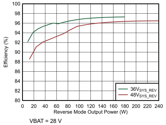
6-10. Reverse Mode Efficiency (7s battery configuration)
