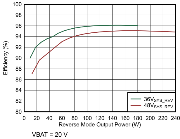
6-9. Reverse Mode Efficiency (5s battery configuration)
