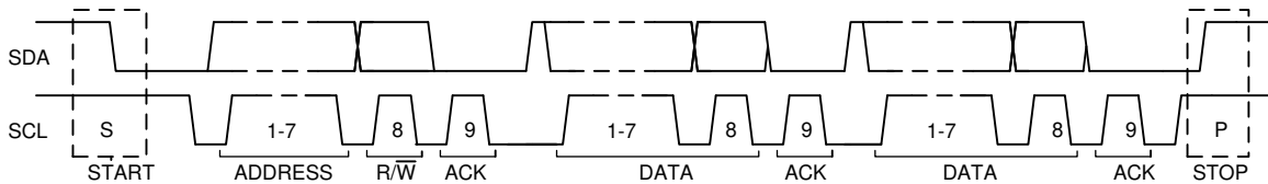
7-10. Complete Data Transfer on the I 2 C Bus
