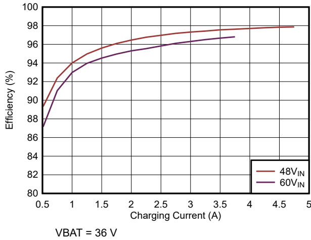
6-3. Charge Efficiency vs Charge Current (9s battery configuration)
