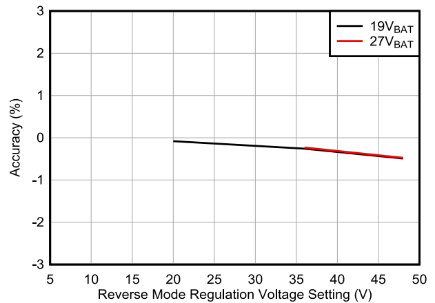
6-12. Reverse Mode Output Voltage Accuracy vs VAC_REV Setting
