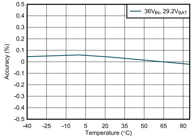
6-4. Charge Voltage Accuracy vs Temperature
