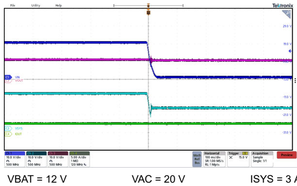
図 8-9. VAC to VBAT Power Path Transfer
