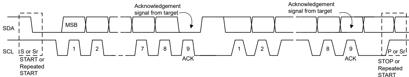
7-9. Data Transfer on the I 2 C Bus
