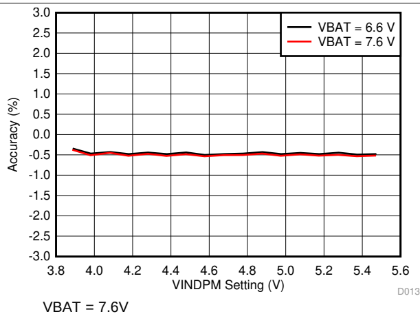
Figure 6. Input Voltage Limit Accuracy vs. VINDPM Setting
