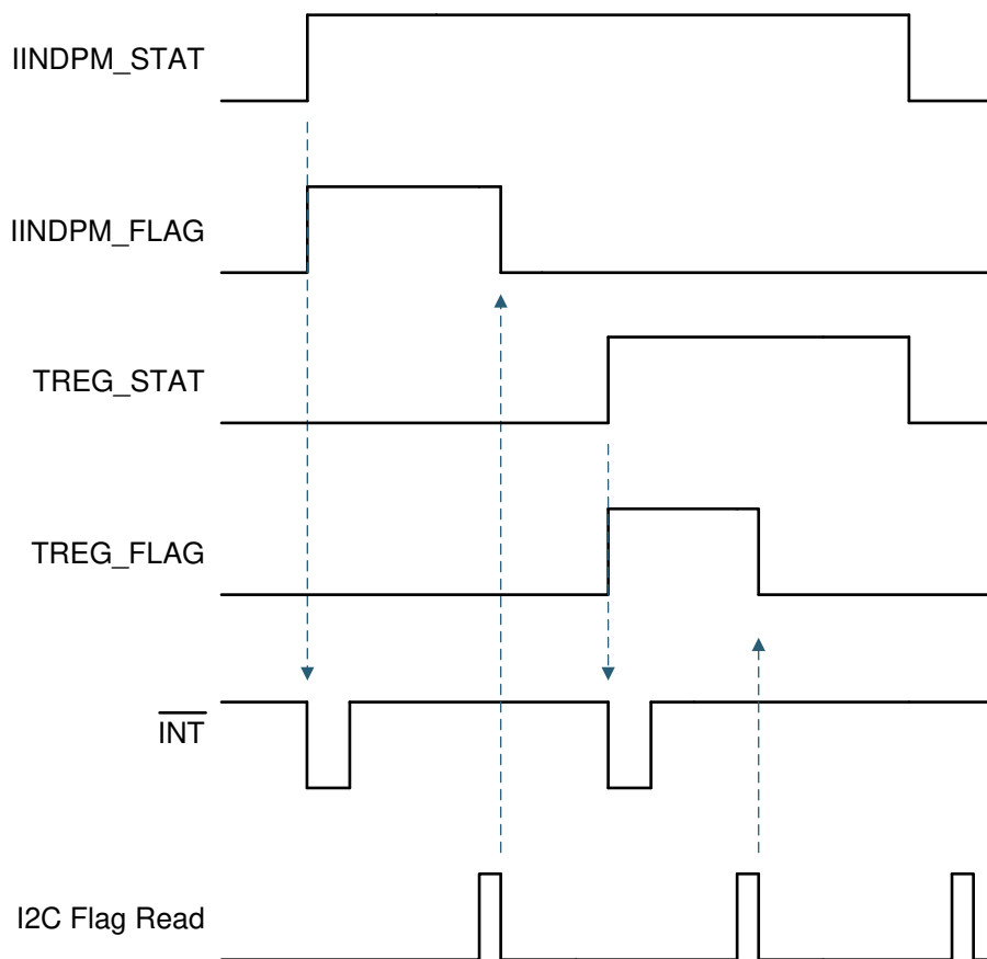
FIG 13. INT Generation Behavior Example
