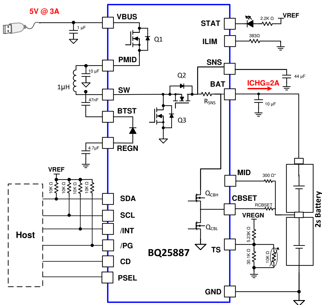
69. BQ25887 (Cell Balancing and I 2 C) Typical Application Diagram
