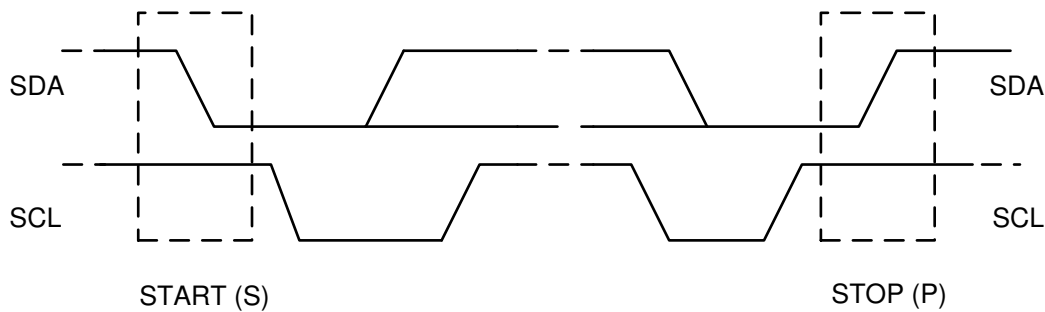
✎ 15. START and STOP conditions on the I2C bus
