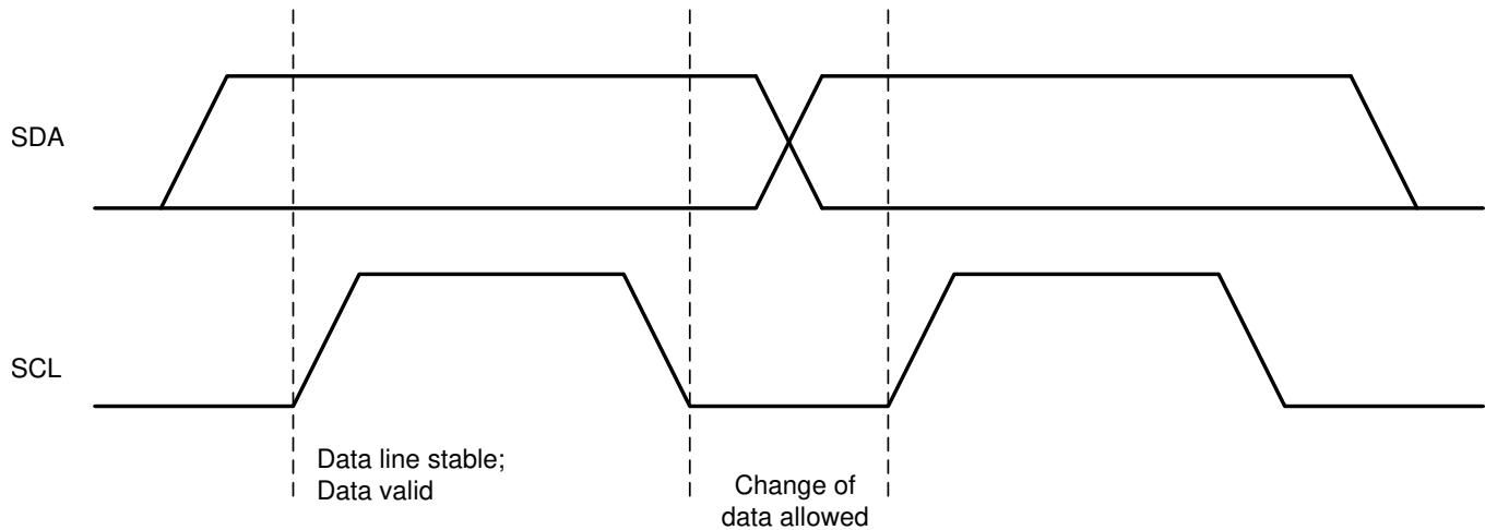
✎ 14. Bit Transfers on the I2C bus
