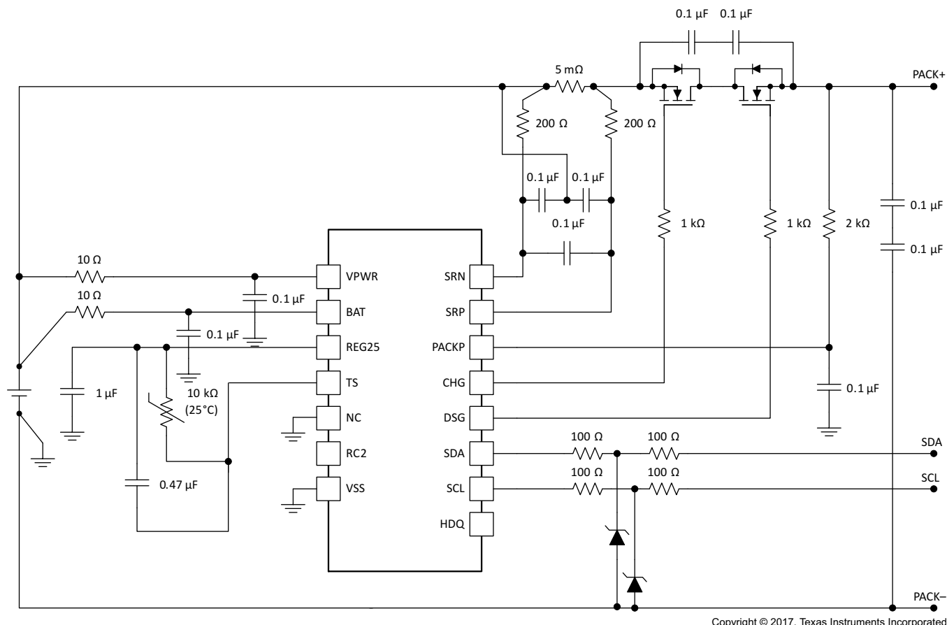
Figure 19. I²C Mode Schematic
