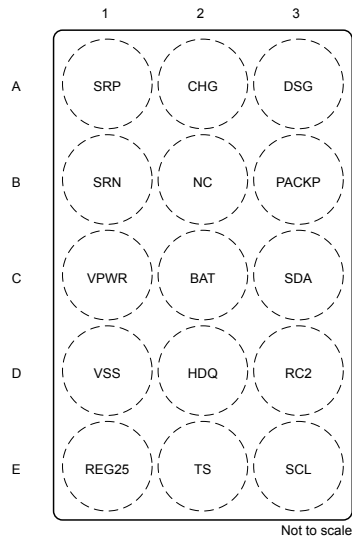
Pin Functions
