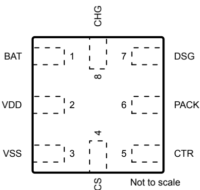
図 5-1. RUG Package 8-Pin X2QFN Top View
