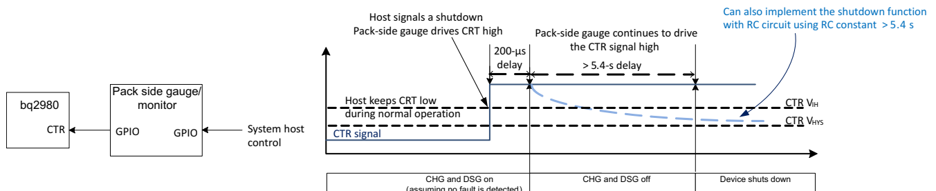
図 7-3. Potential System- Controlled Shutdown Implementation
