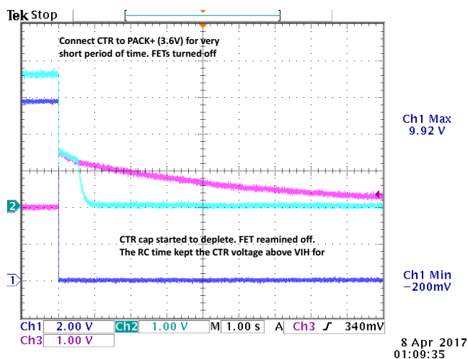
図 8-11. Setup CTR for System Reset (Using 5M \Omega and 1 \mu F RC)
