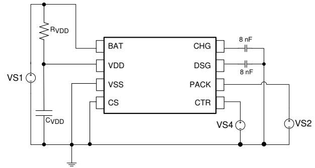
✎ 8-4. Test Circuit 4
