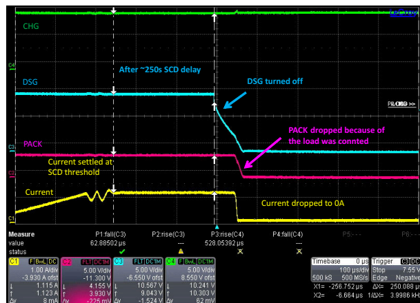
図 8-10. Short Circuit (SCD) Protection
