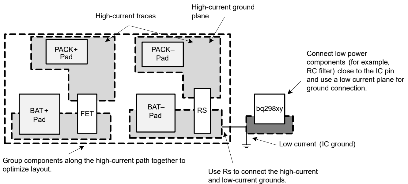
図 10-1. Component Placement and Grounding Pattern Example
