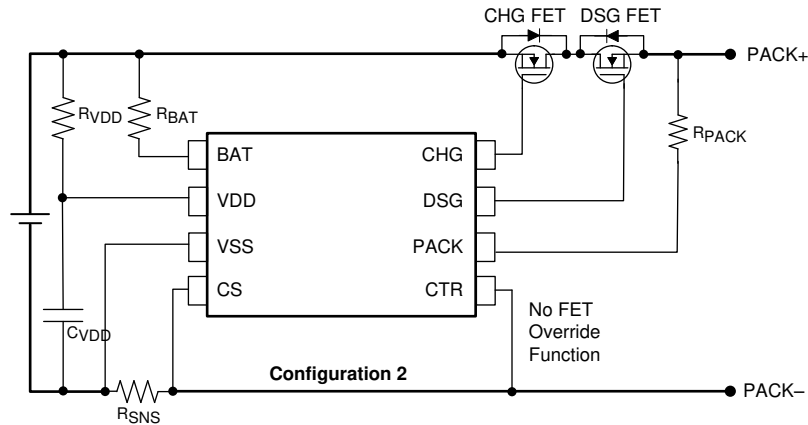
8-13. BQ298xx Reference Schematic Configuration 2
