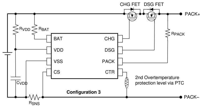
8-14. BQ298xx Reference Schematic Configuration 3
