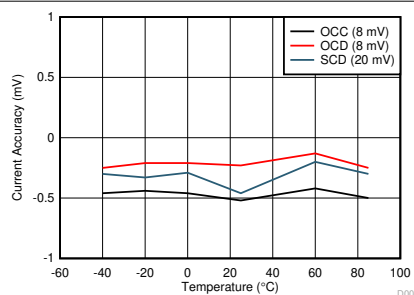
Figure 6-4. Overcurrent Accuracy Across Temperature
